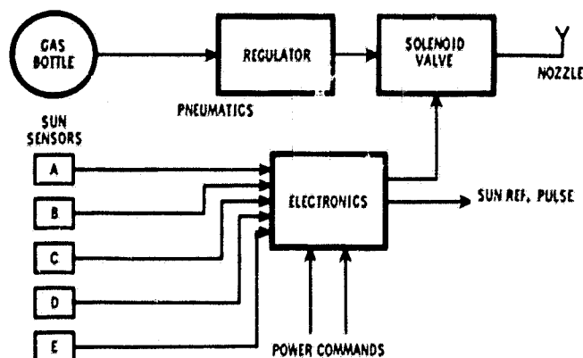
Figure 2. Orientation Control Subsystem Block Diagram
