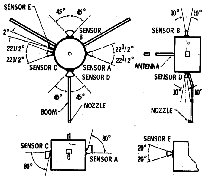
Figure 3. Sun Sensor Locations and Fields-of-View
