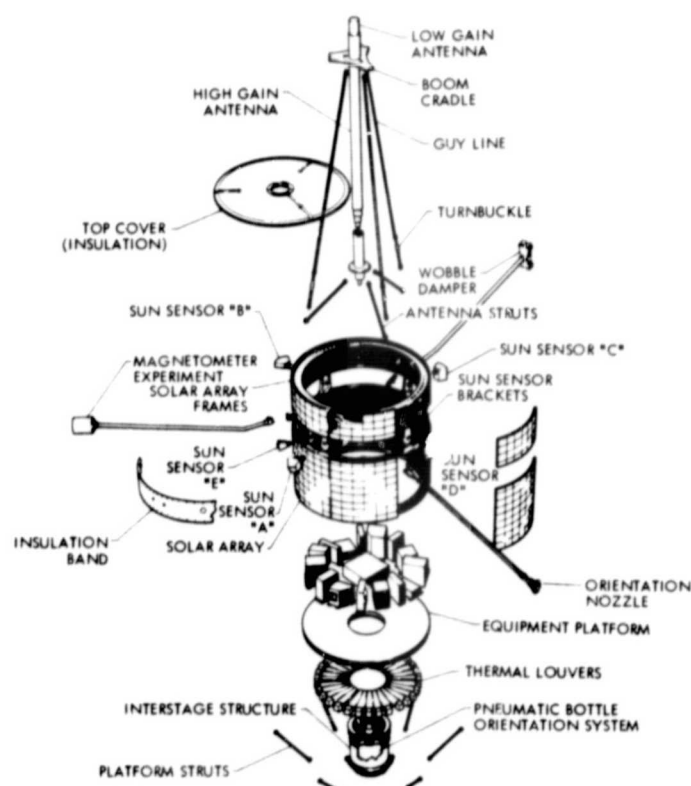
Figure 1. Pioneer VI Spacecraft
