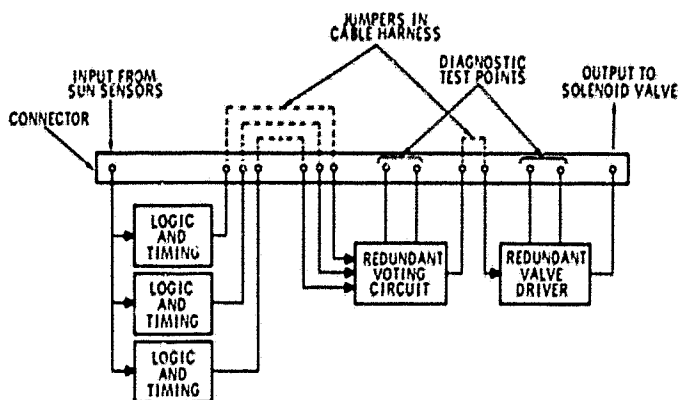
Figure 7. Alternate Redundancy Technique for Orientation Control Electronics
