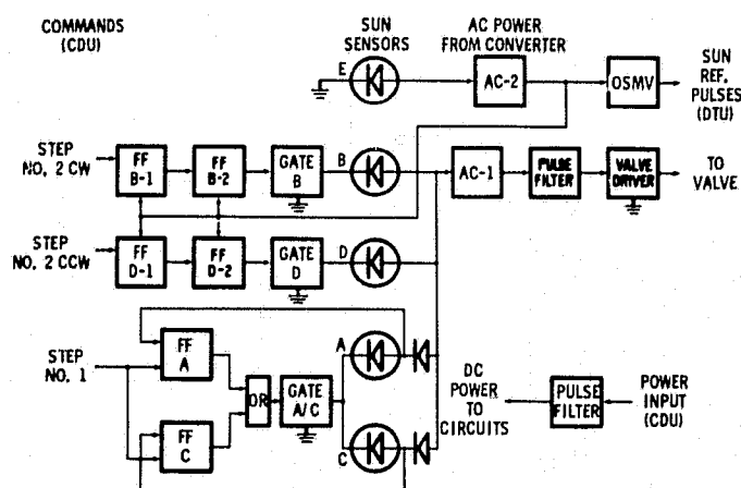
Figure 5. Electronics Assembly Block Diagram
