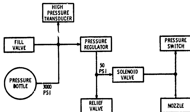
Figure 4. Pneumatics Assembly Block Diagram
