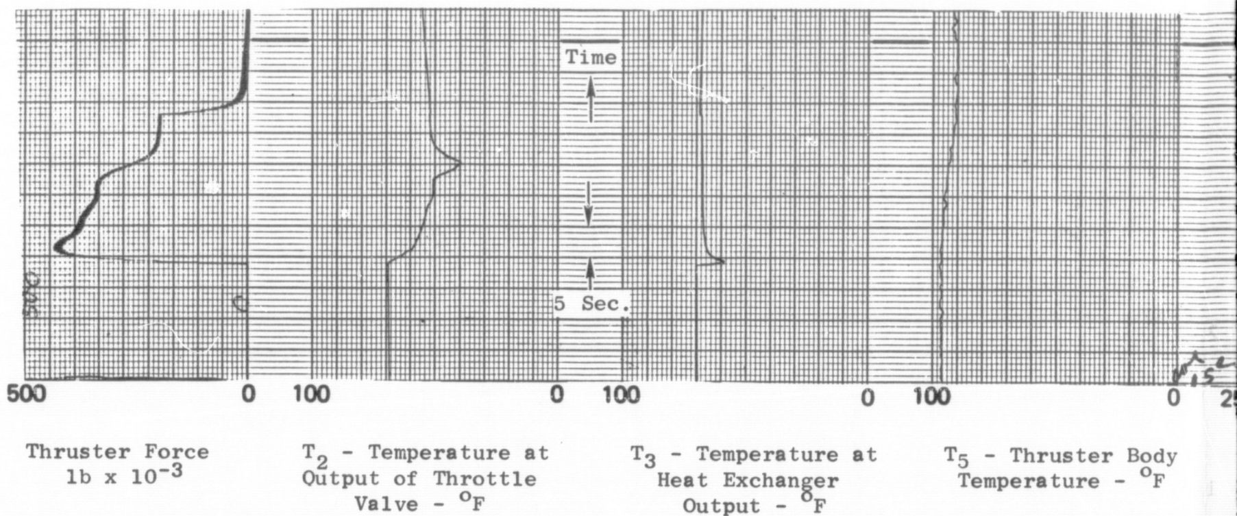
Vapor Feed Pulse Data
