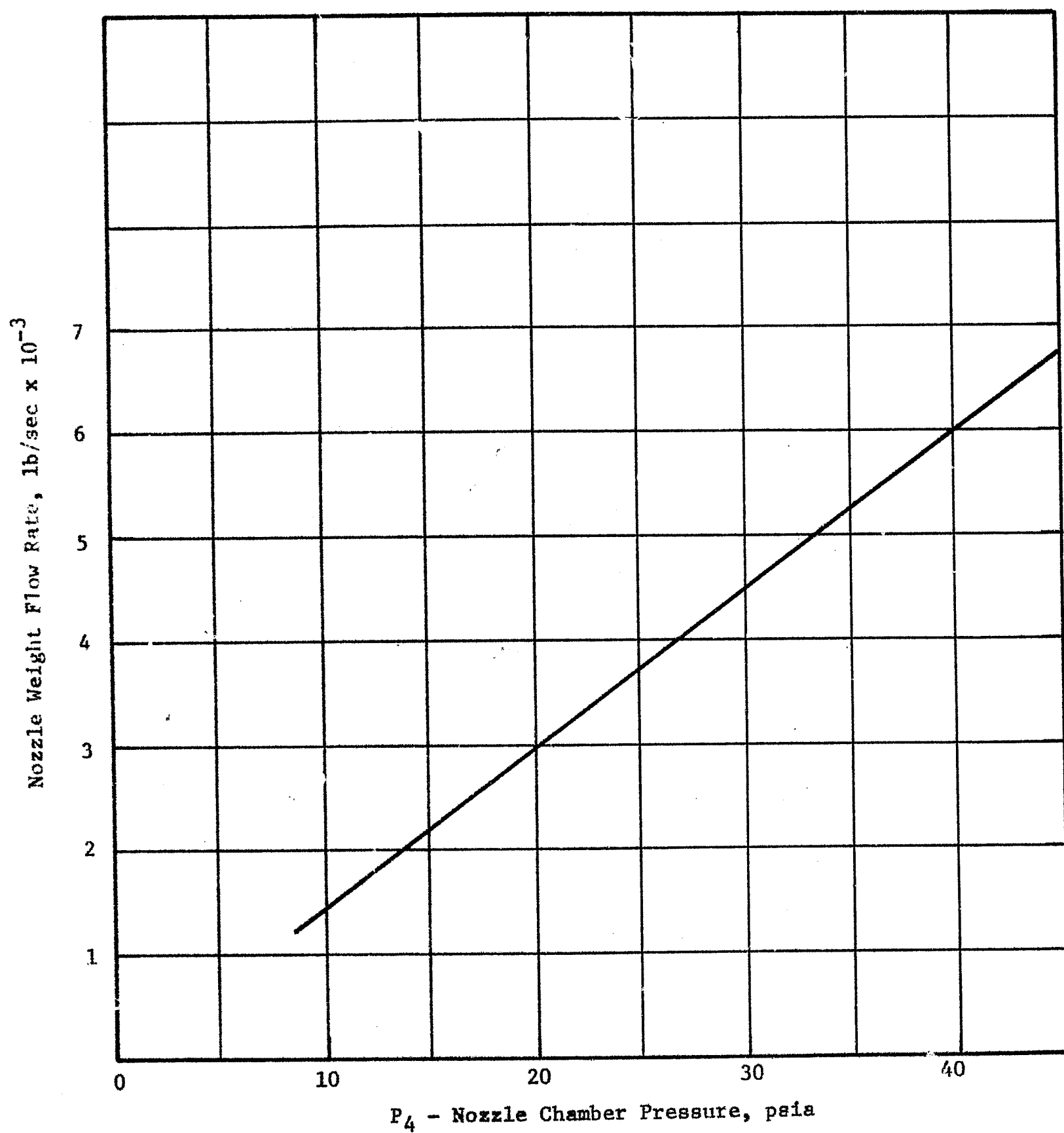
Figure 27. Nozzle Weight Flow Rate As A Function of Chamber Pressure (P 4 ).
