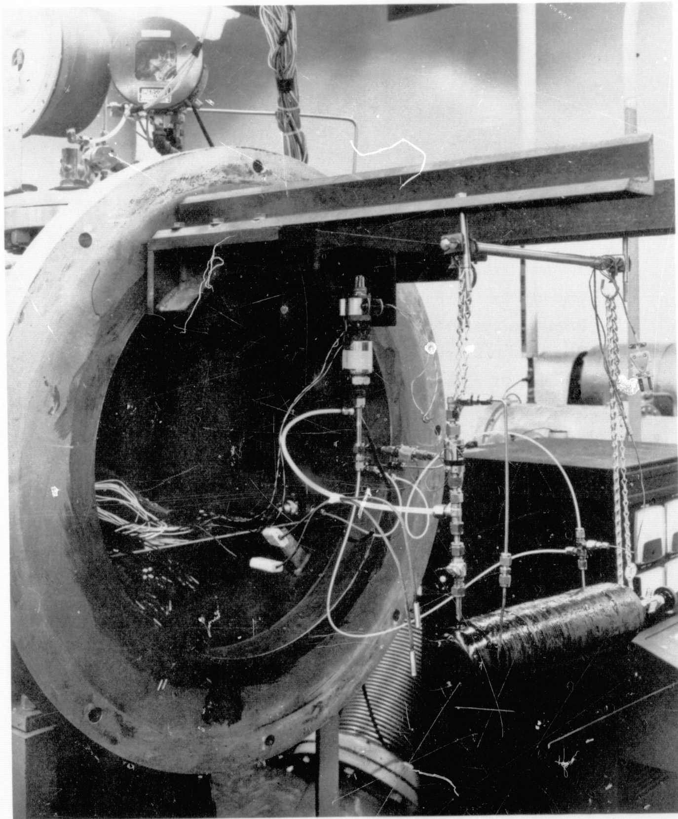
Figure 21. Sub-Scale Test Hardware in Vacuum Tank.
