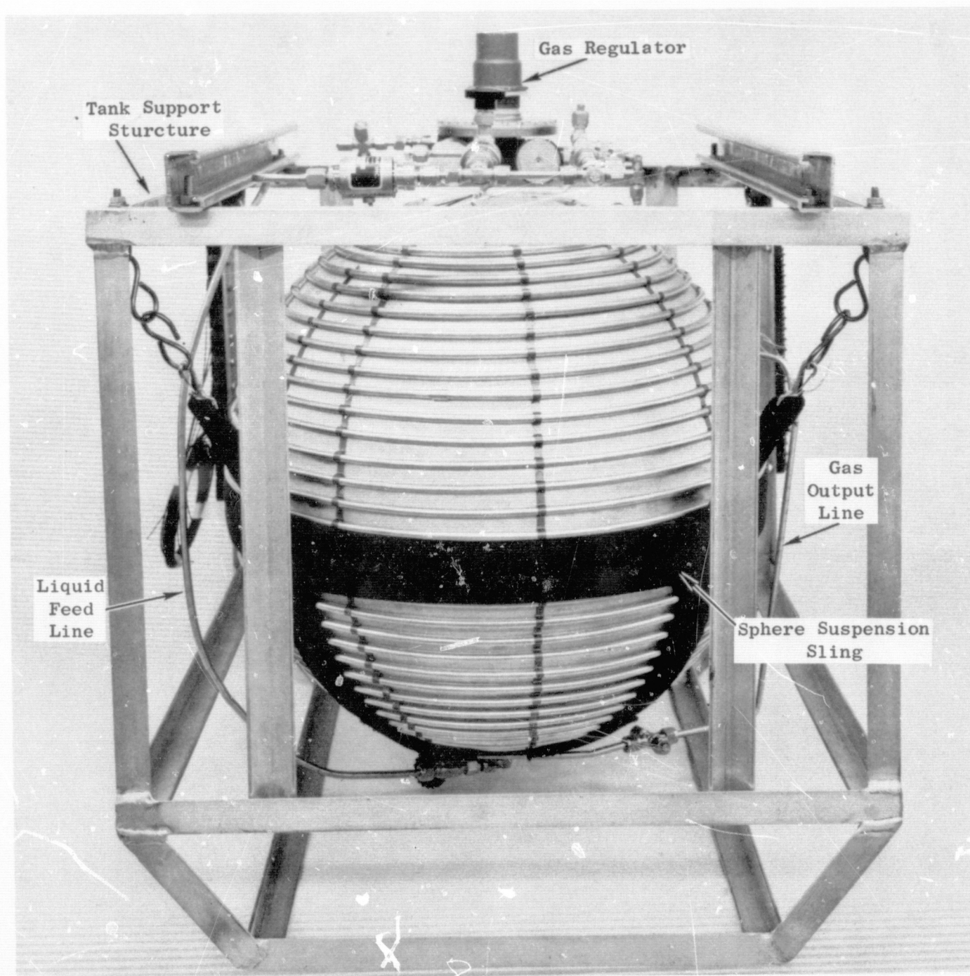
Figure 12. Feed System Components Mounted in Support Structure (End View).
