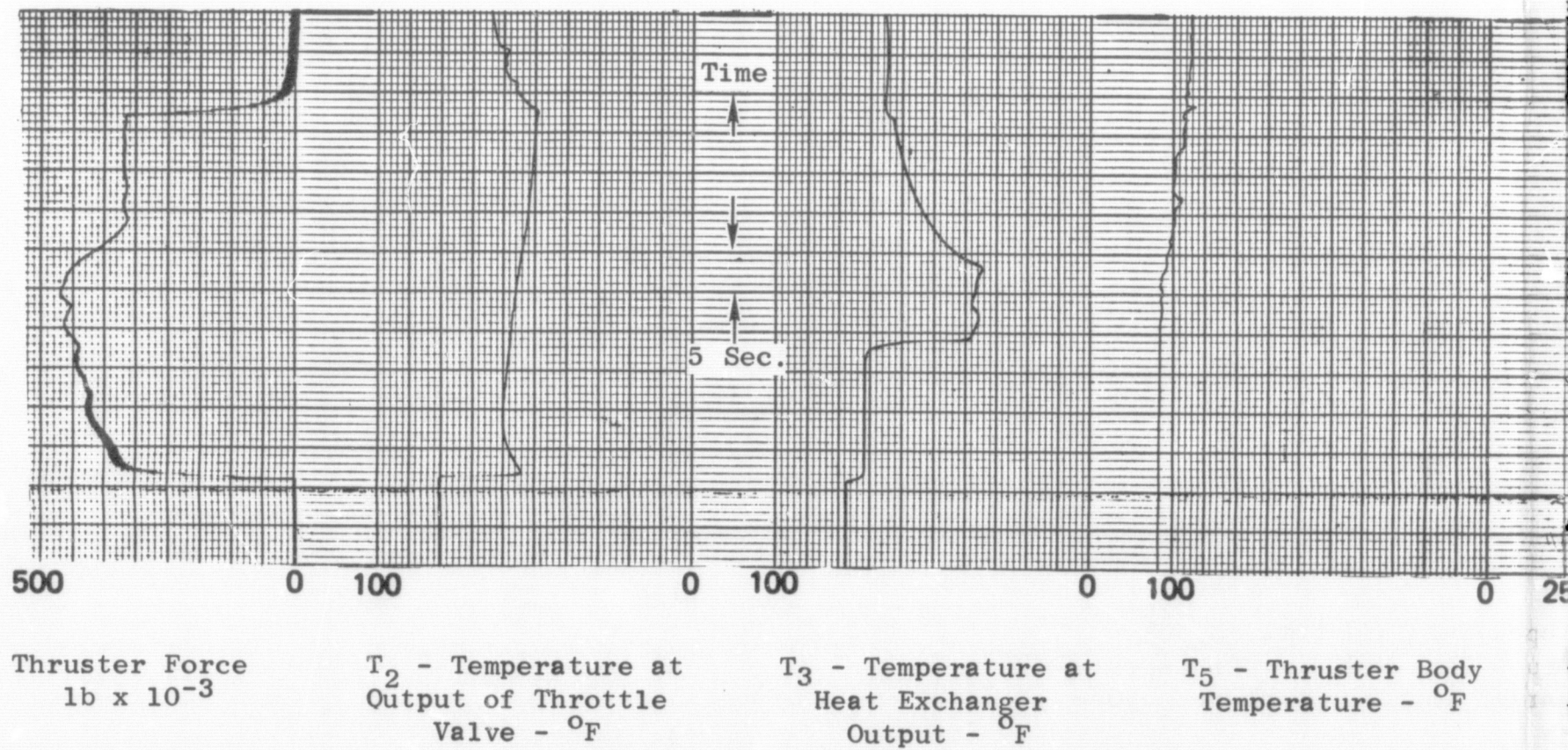
Liquid Feed Pulse Data
