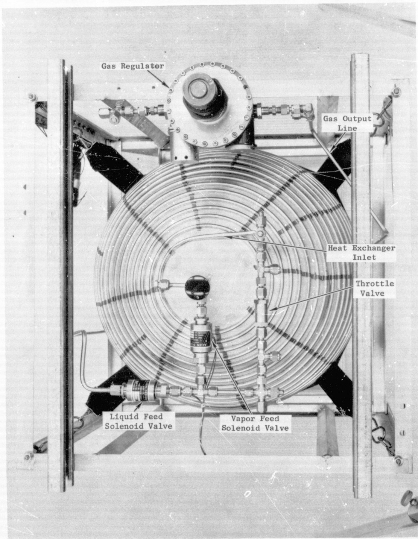
Figure 13. Feed System Components Mounted in Support Structure (Top View).
