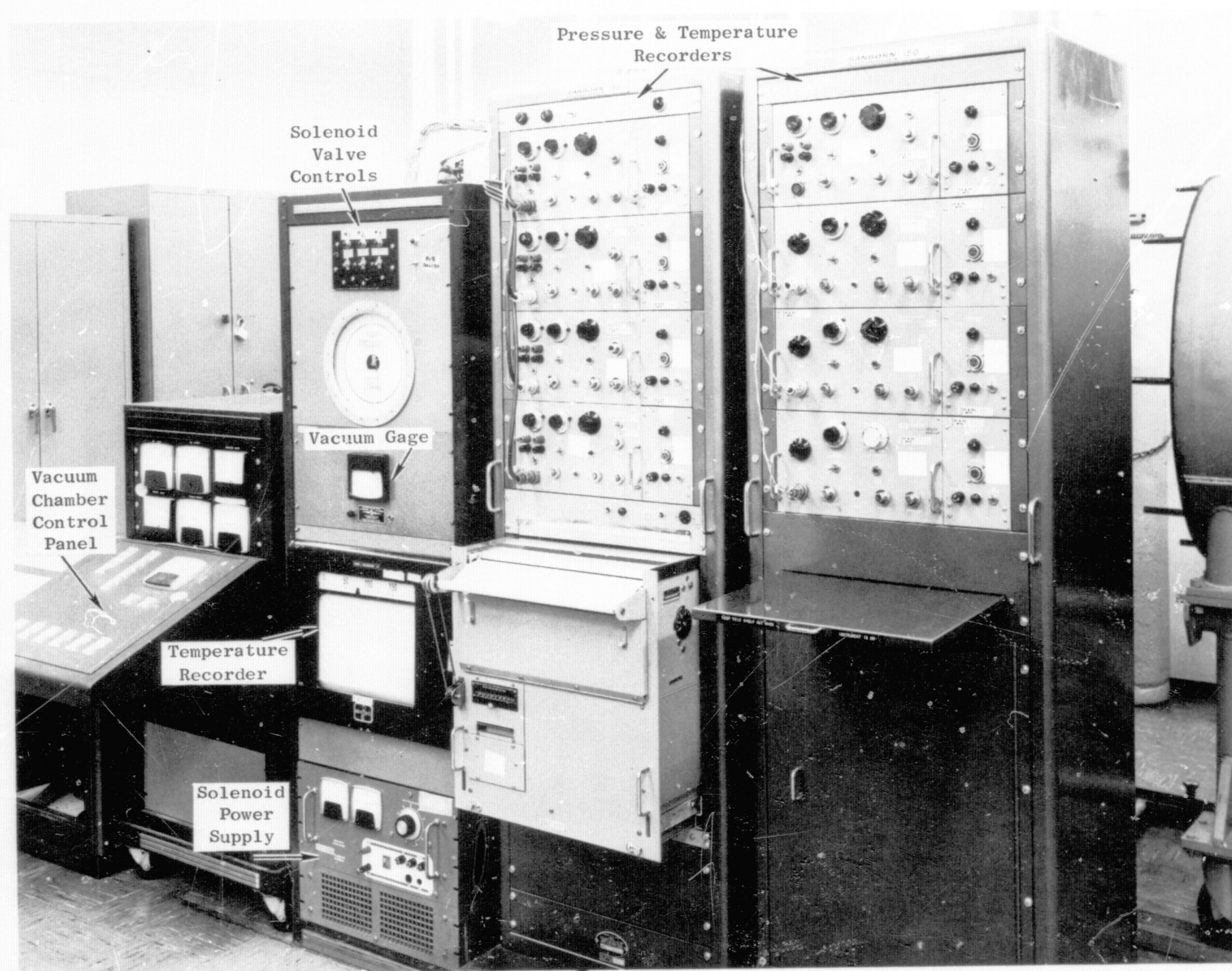
Figure 15. System Instrumentation Recorders.
