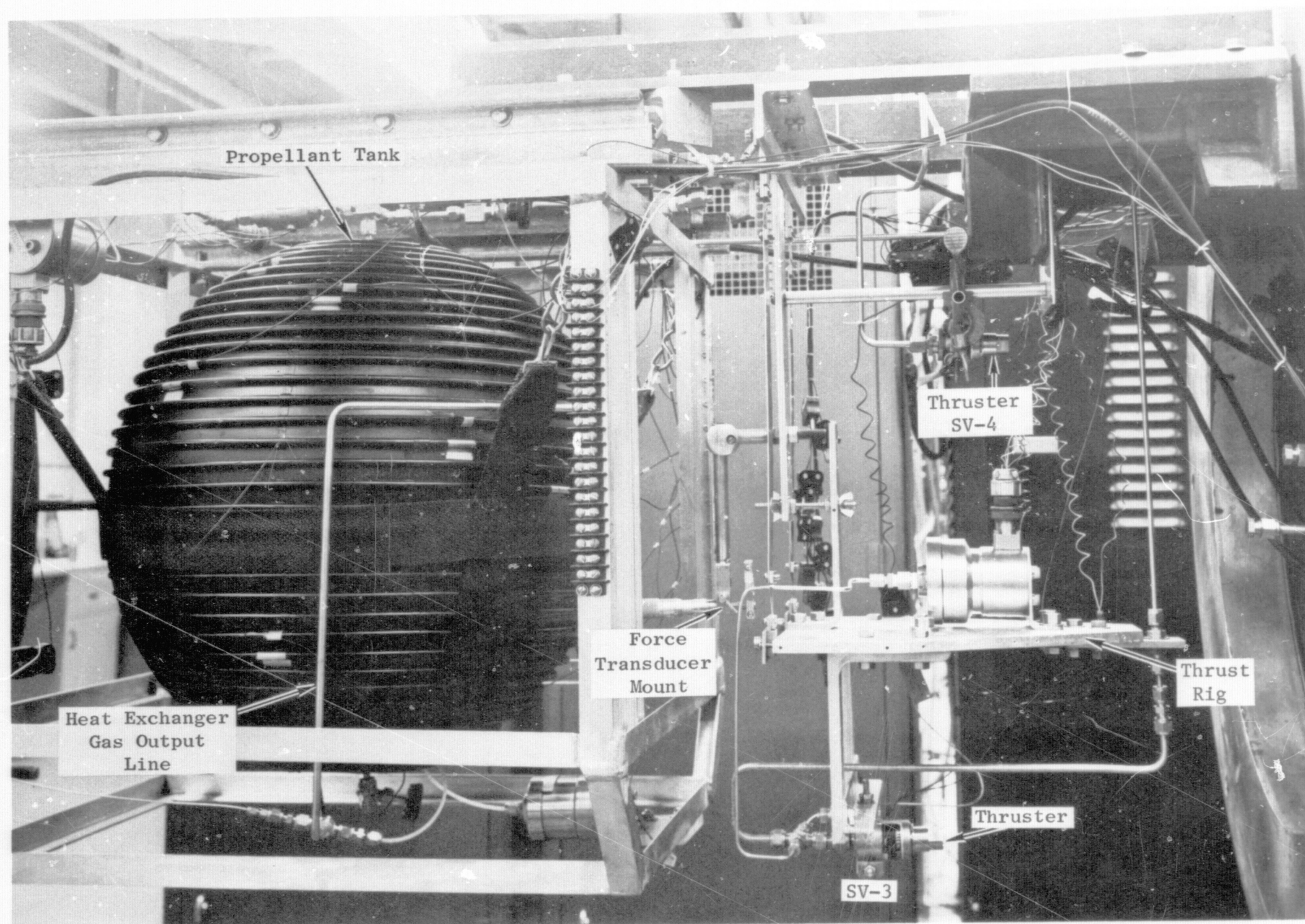
Figure 14. Side View of System.
