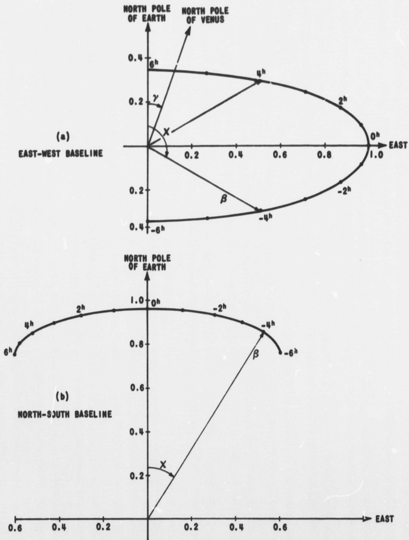
FIGURE 1. - LENGTH \beta AND POSITION ANGLE \chi OF INTERFEROMETER BASELINE, AS PROJECTED ON PLANE OF SKY AT VENUS
