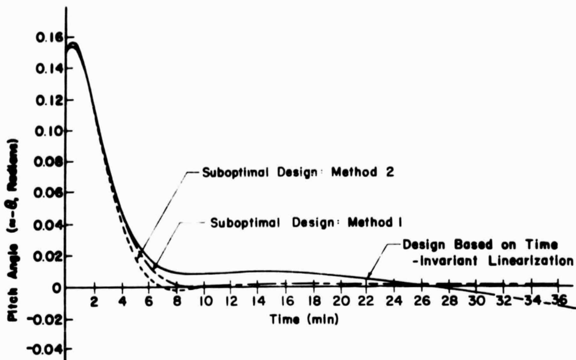
Fig. 4 Example I, Pitch Angle vs. Time; Initial Inertia Wheel Angular Momentum = 4 slug-ft 2 /sec
