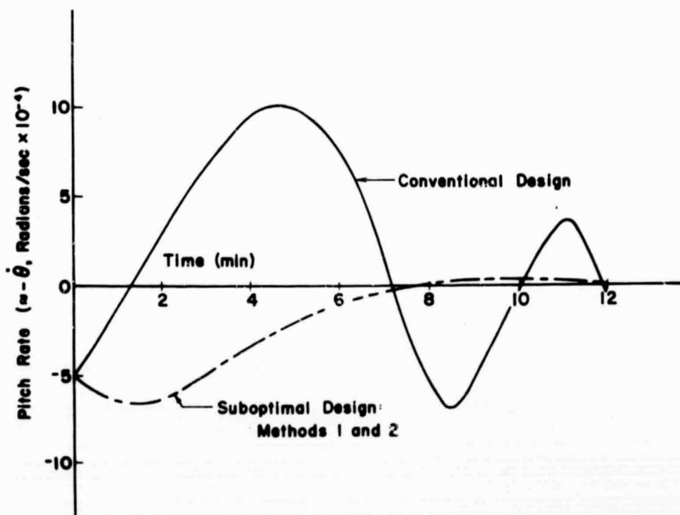
Fig. 9 Example I, Pitch Rate vs. Time, Conventional and Suboptimal Designs; Initial Inertia-Wheel Angular Momentum = 0
