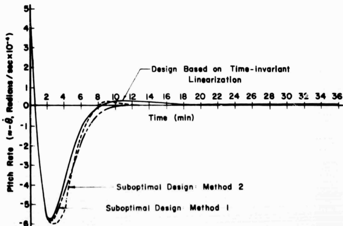
Fig. 5 Example I, Pitch Rate vs. Time; Initial Inertia-Wheel Angular Momentum = 4 slug-ft 2 /sec
