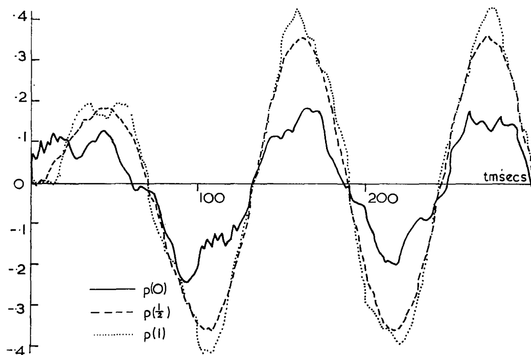
Fig 24(b) Displacement and Velocity responses at Plate Centre Pressure Responses \text{TAU} = 100 \text{ msecs} .
