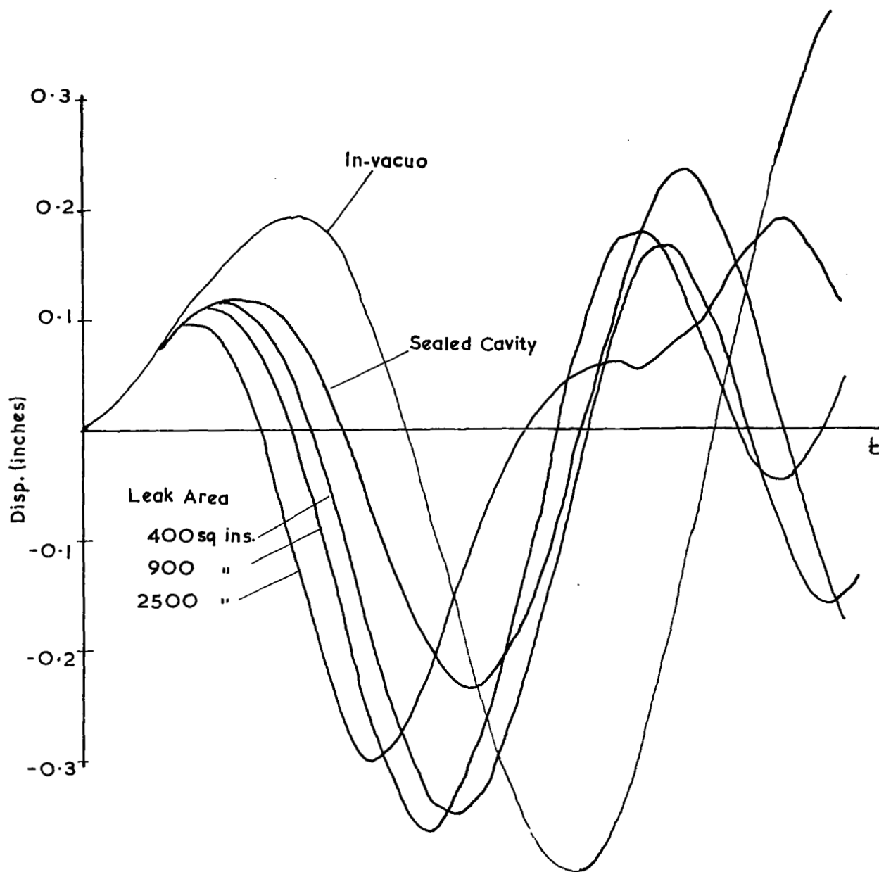
Fig 14 Displacement Response to ideal N wave \tau = 150 ms. under in-vacuo and various leak openings Plate dimensions 144x84x0.25 Cavity Volume 3.0 \times 10^3 ins. 3
