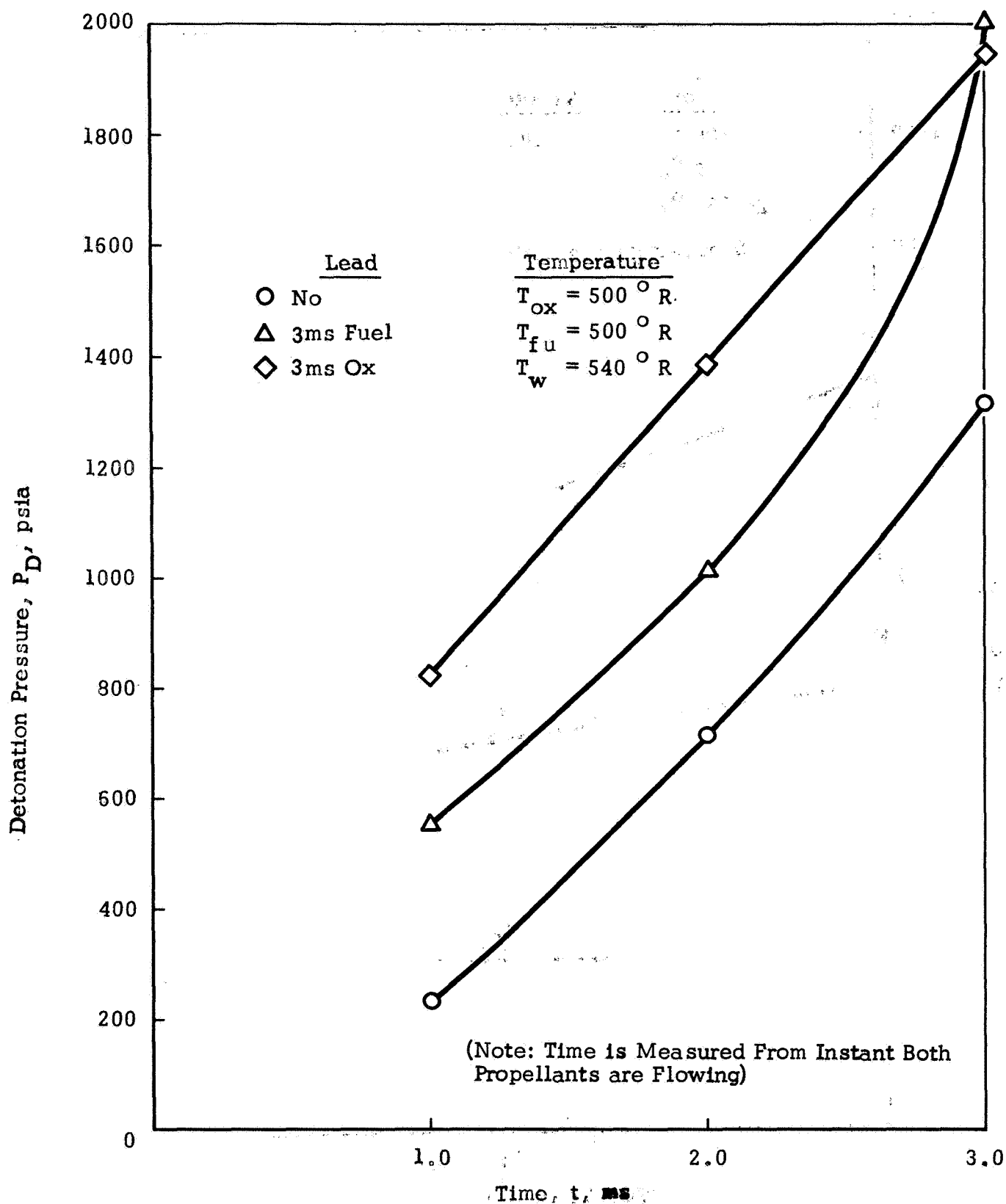
Figure 16. Effect of Propellant Leads and Initial Temperature on Detonation Pressure
