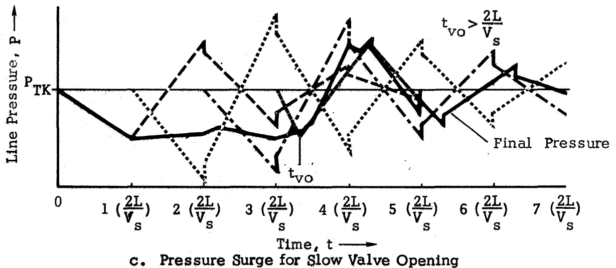
Figure 3. Pressure Transients Between Propellant Valve And Tank Caused By Valve Opening
