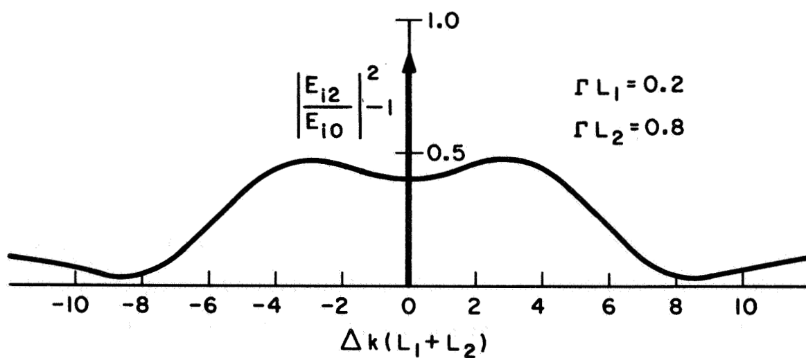
FIG. 2--Incremental power gain versus \Delta k (L_1 + L_2) .
