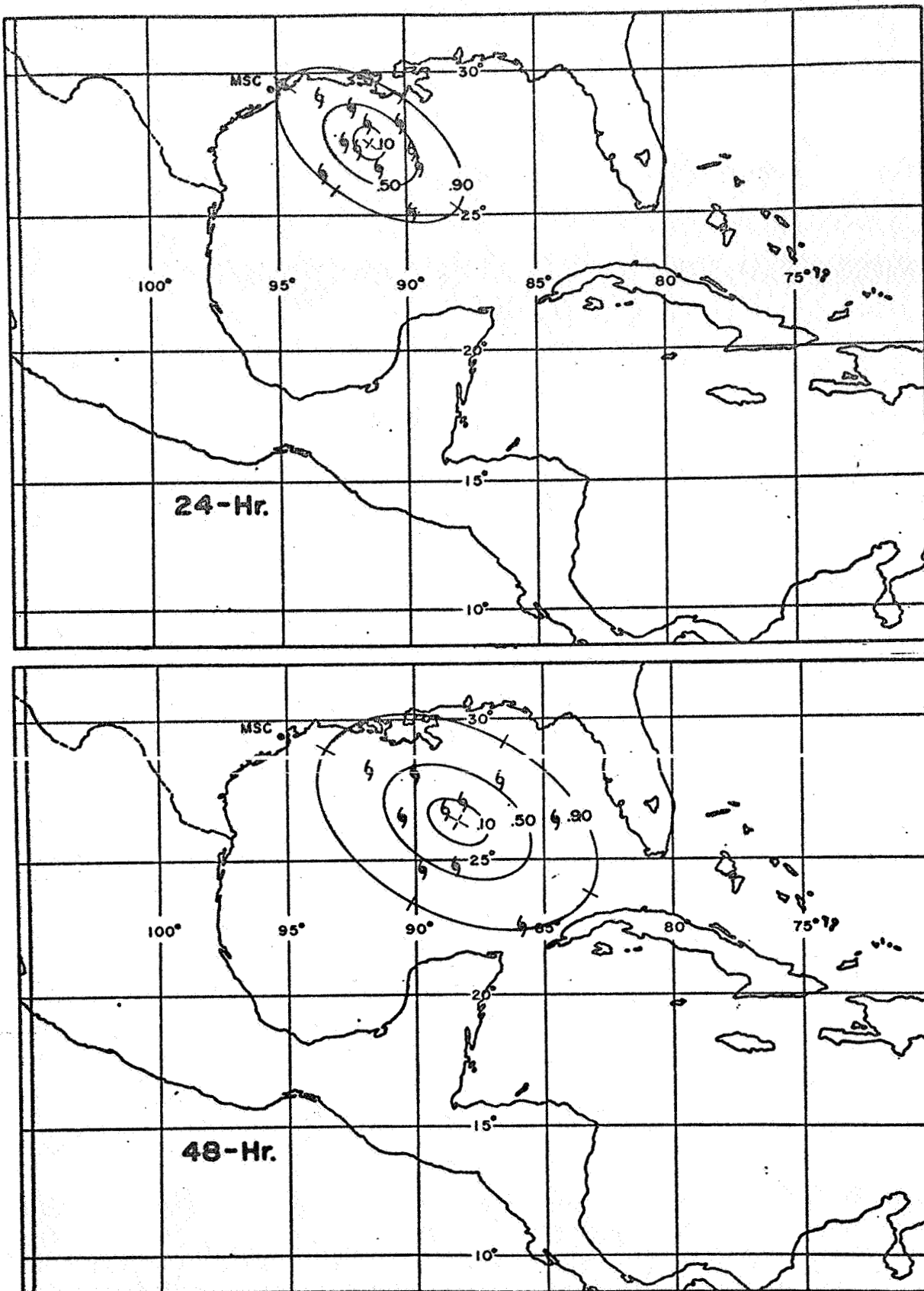
Figure 12. - Probability ellipses of the distribution of category 1 tropical storms or hurricanes 24 and 48 hours prior to producing critical winds at the Manned Spacecraft Center.
