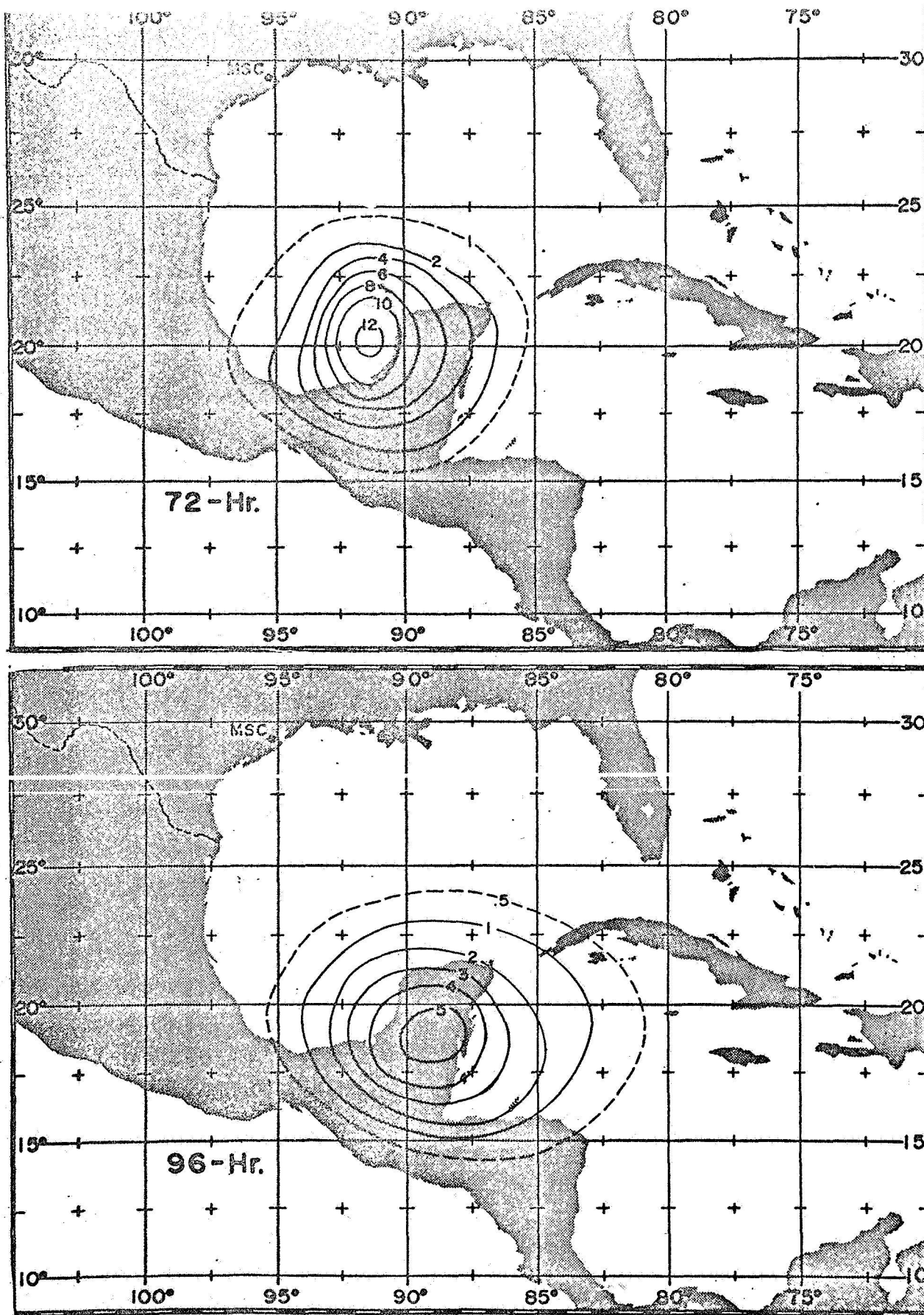
Figure 23. - Percent probability of category 2 tropical storms or hurricanes producing critical winds at the Manned Spacecraft Center in exactly 72 and 96 hours.
