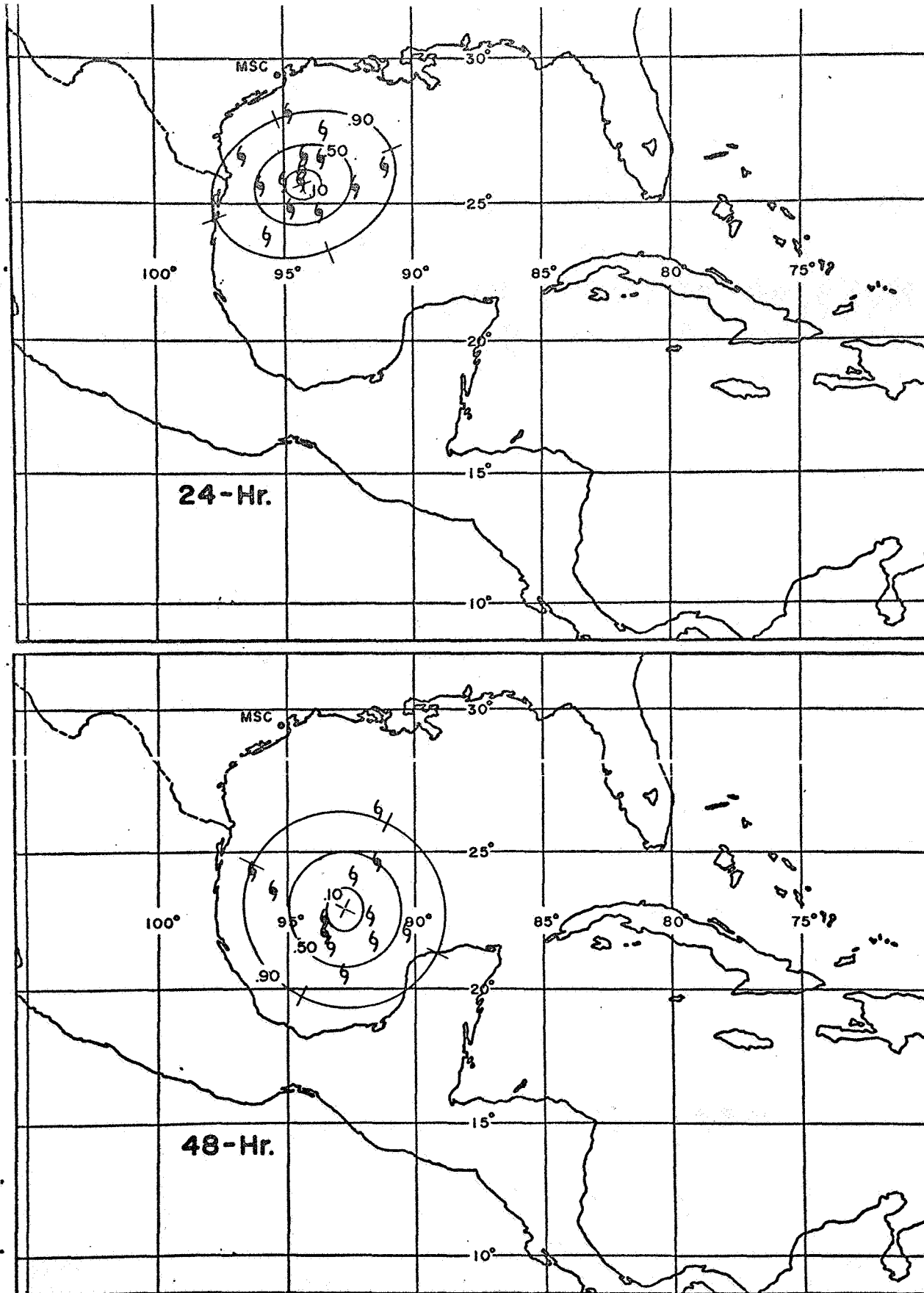
Figure 14. - Probability ellipses of the distribution of category 2 tropical storms or hurricanes 24 and 48 hours prior to producing critical winds at the Manned Spacecraft Center.
