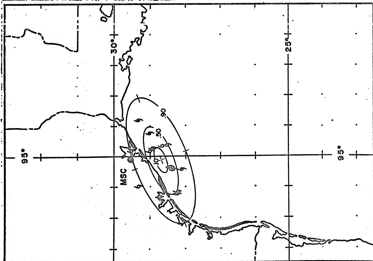
Figure 11. - Probability ellipses of the distribution of tropical storms or hurricanes, 1886-1967, when they first produced critical winds at MSC: Left , category 2 storms; right , category 1 storms.
