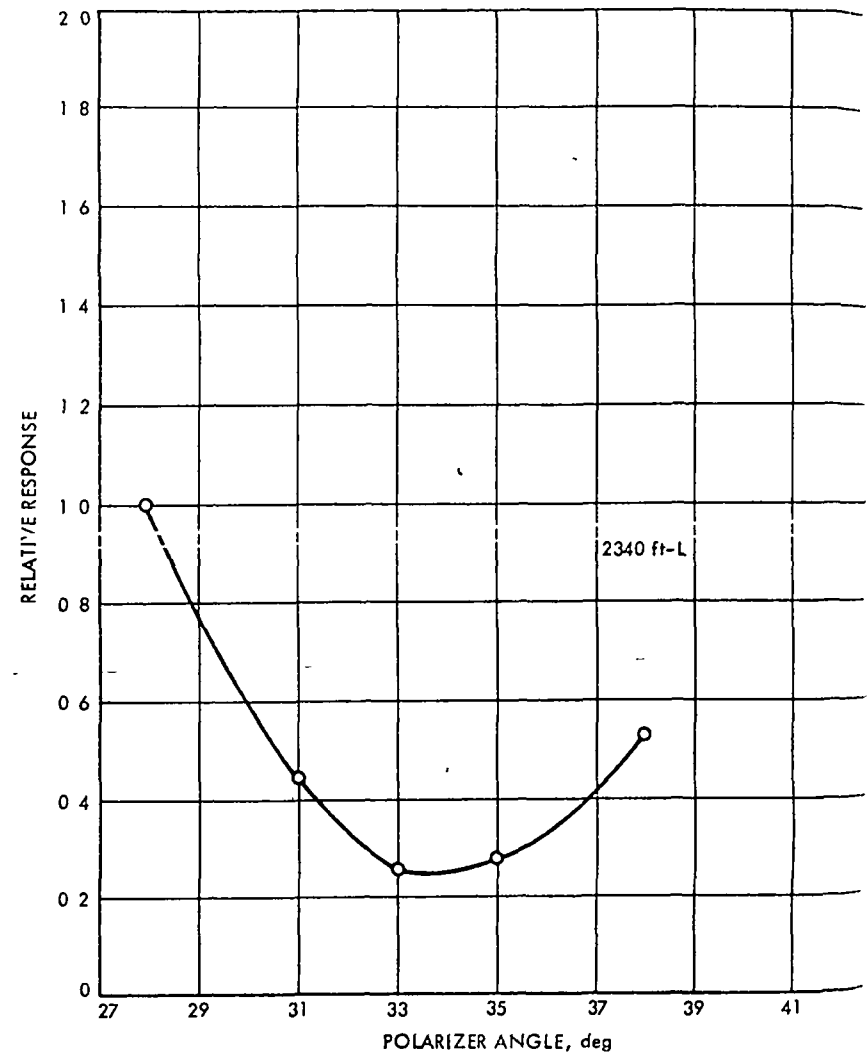
Figure 19. Polarization Null, N-Filter f/4 , Open Shutter, 600-Line Scan Mode, Transmitter
