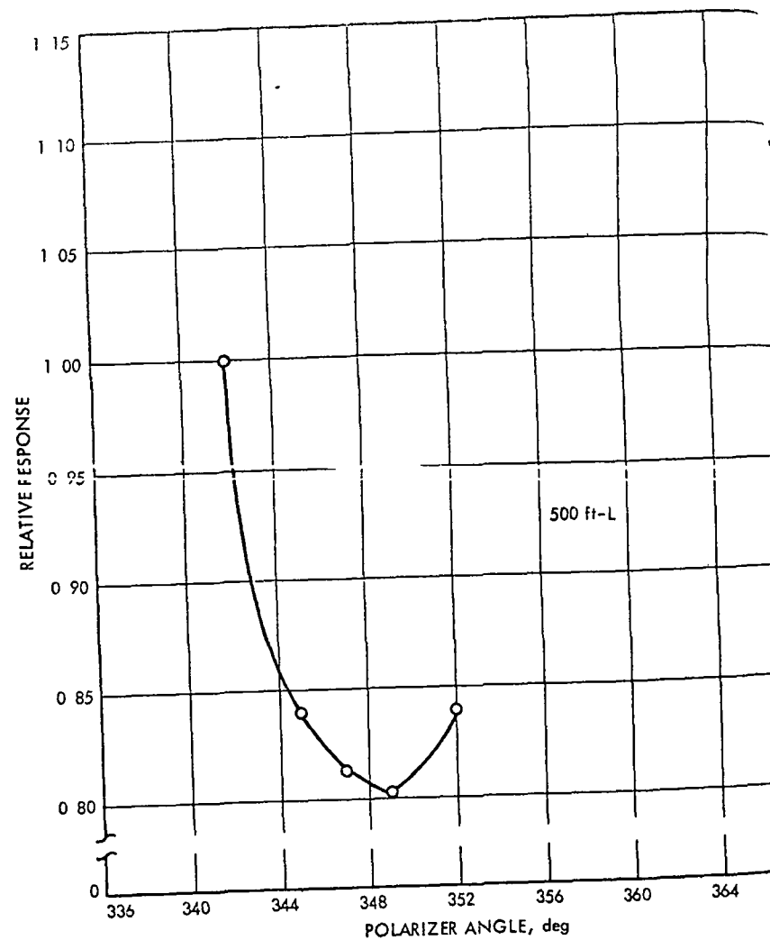
Figure 17 Polarization Null, P-Filter f/4, Open Shutter, 600-Line Scan Mode, Transmitter A
