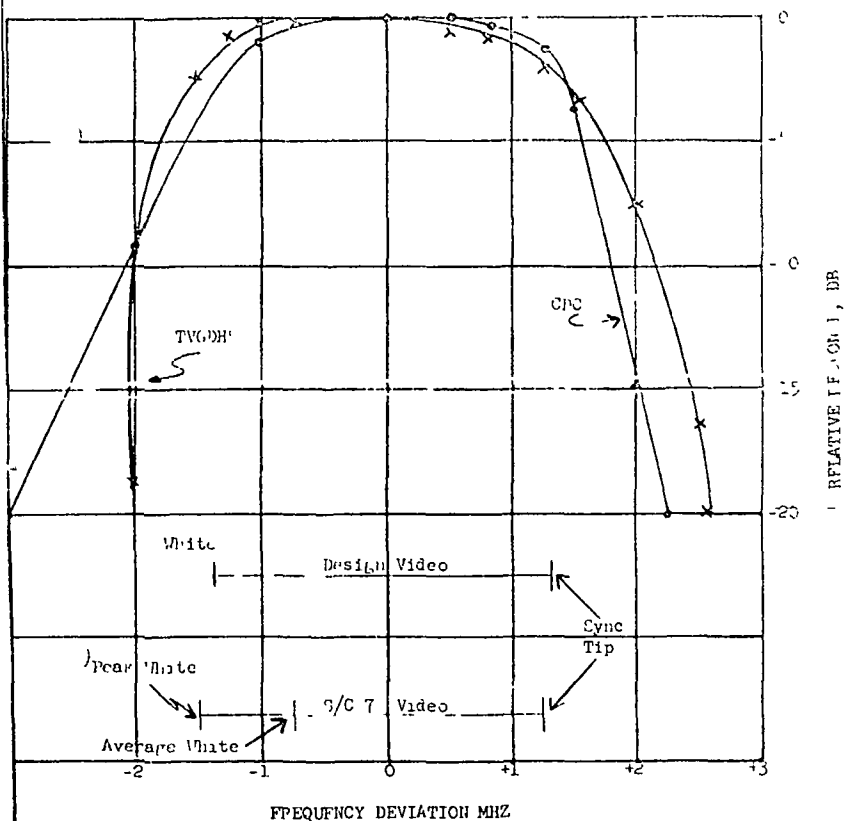
FIGURE I Ground System Filter Response and Video Frequency Deviations
