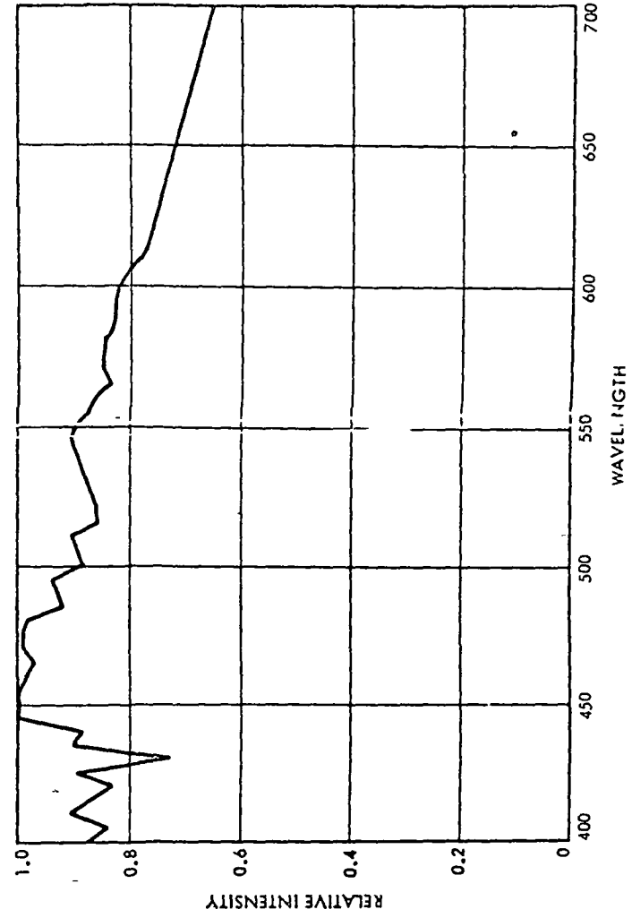
Figure 3 Solar Spectrum
