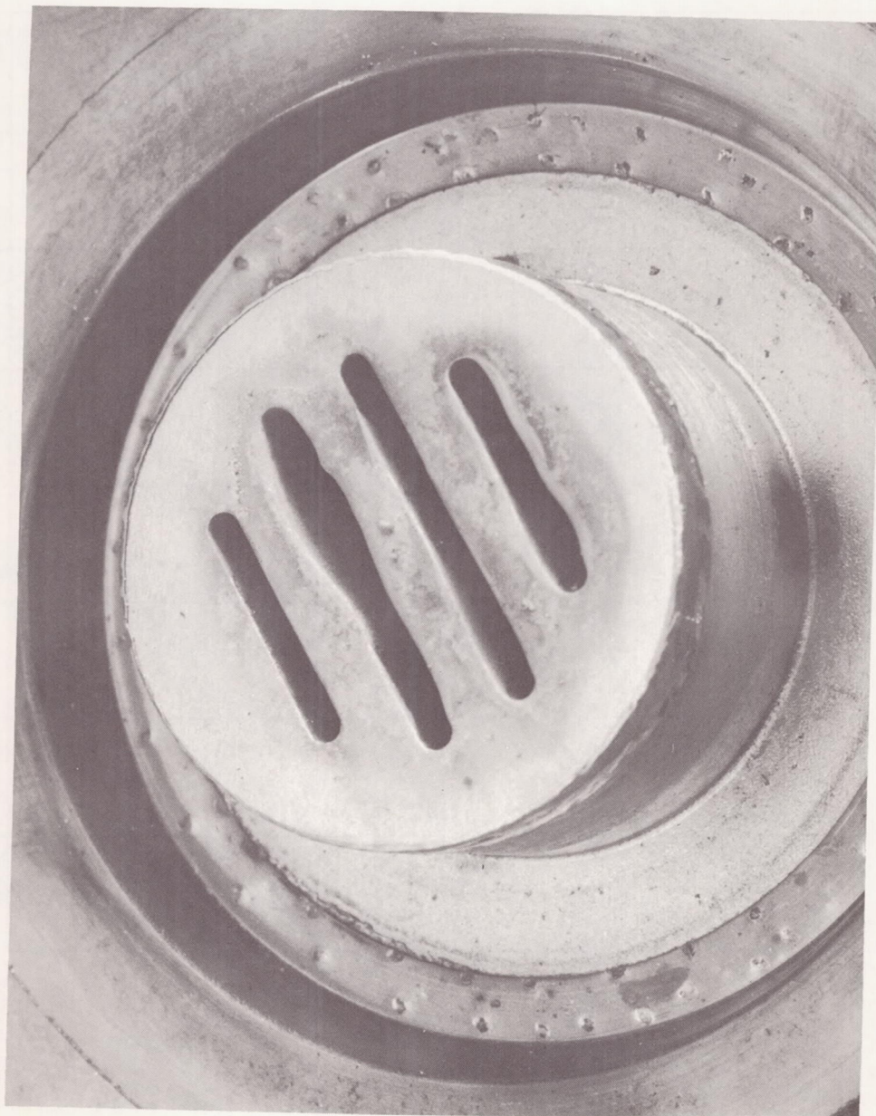
Figure 21 - Eroded Cathode Shield from Tube No. 31
