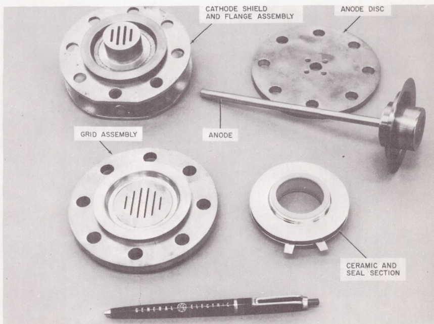
Figure 4 - Thyratron Subassemblies with Tungsten Strip Cathode and Shield in Place
