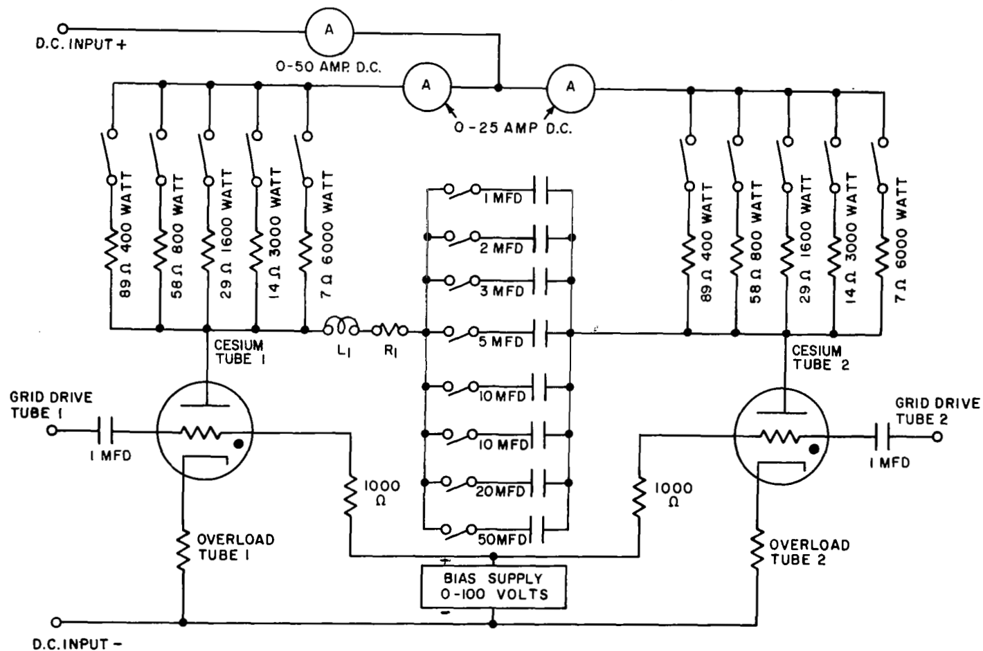
Figure 8 - Inverter Load and Commutating Circuitry
