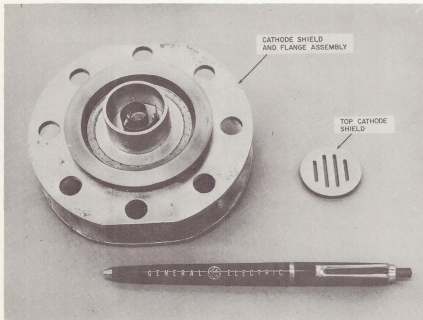
Figure 5 - Cathode Section of Cesium Thyratron
