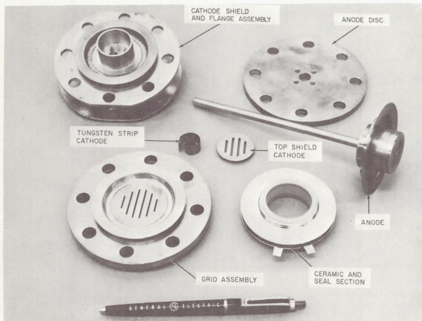
Figure 3 - Thyatron Subassemblies with Tungsten Strip Cathode Exposed
