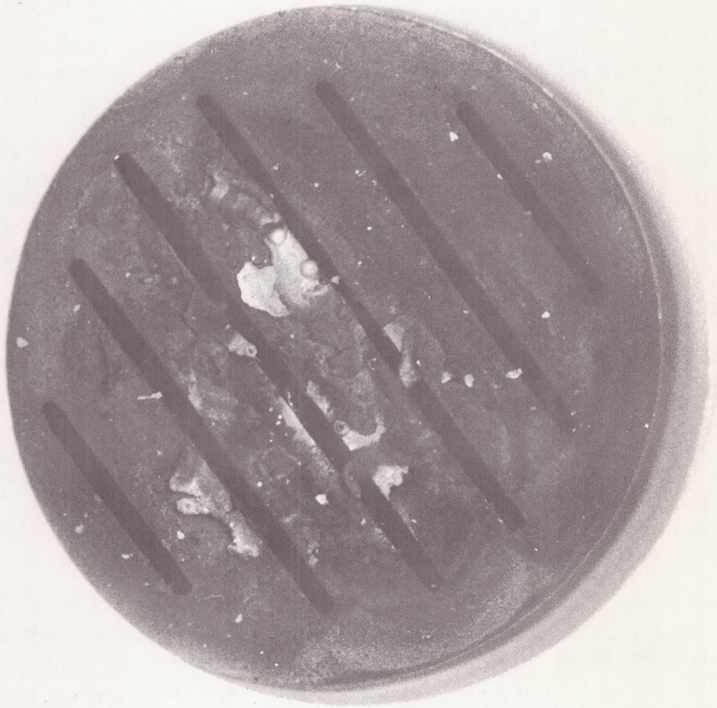
Figure 22 - Contaminated Grid from Tube No. 31
