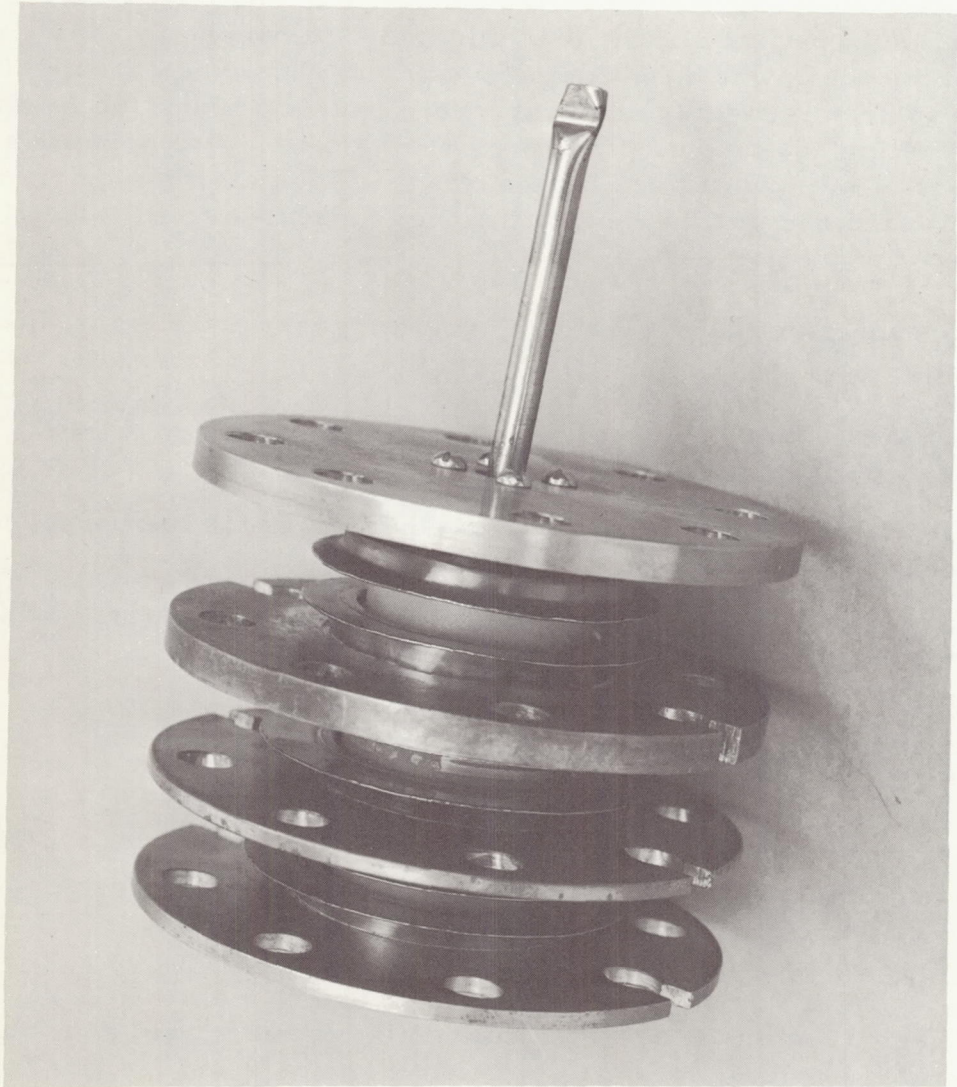
Figure 1 - Assembled Cesium Thyratron
