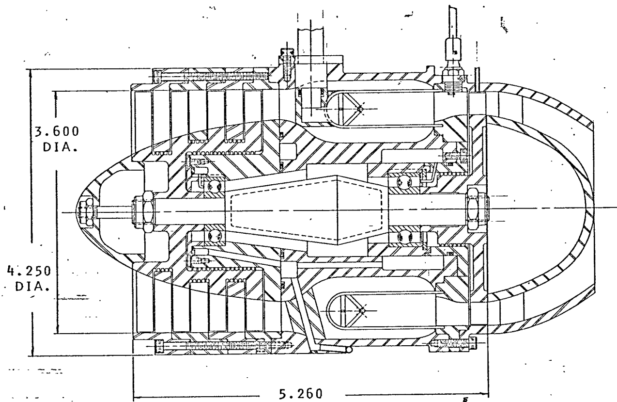
FIG. 24 - PROPOSED ENGINE ASSEMBLY
