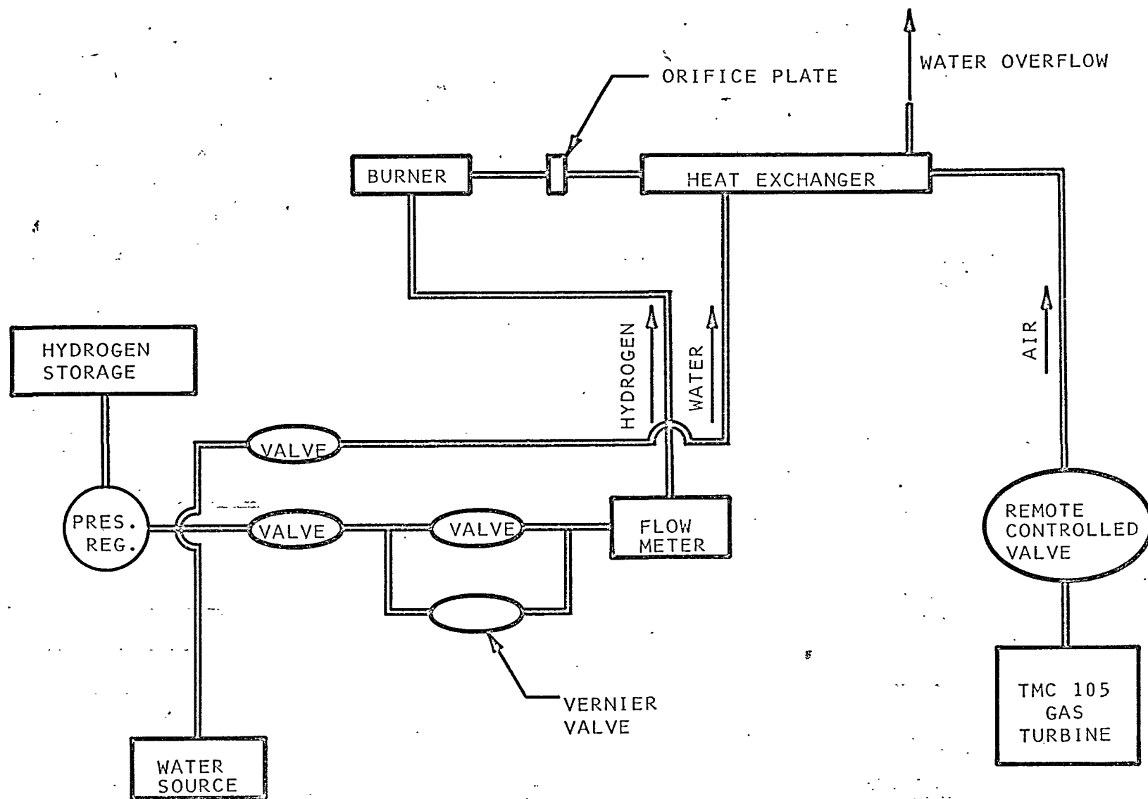
FIGURE 1 - TEST INSTALLATION SCHEMATIC
