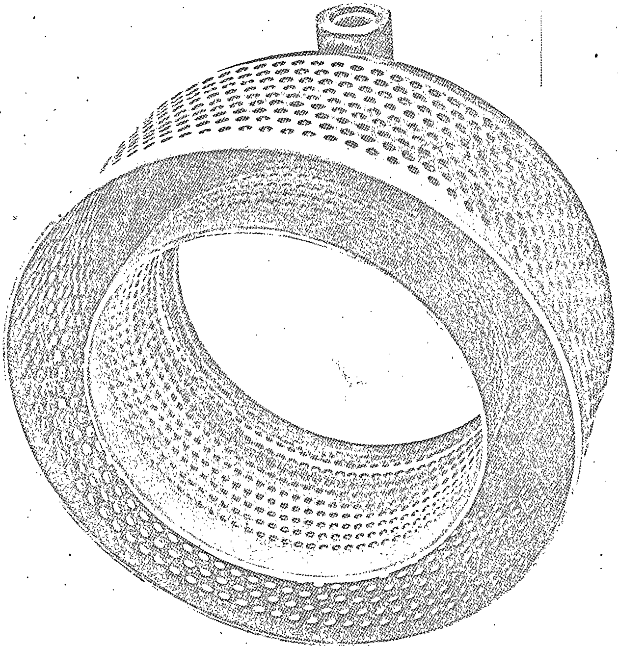
FIGURE 22 - FINAL COMBUSTOR LINER AFTER ENDURANCE RUN
