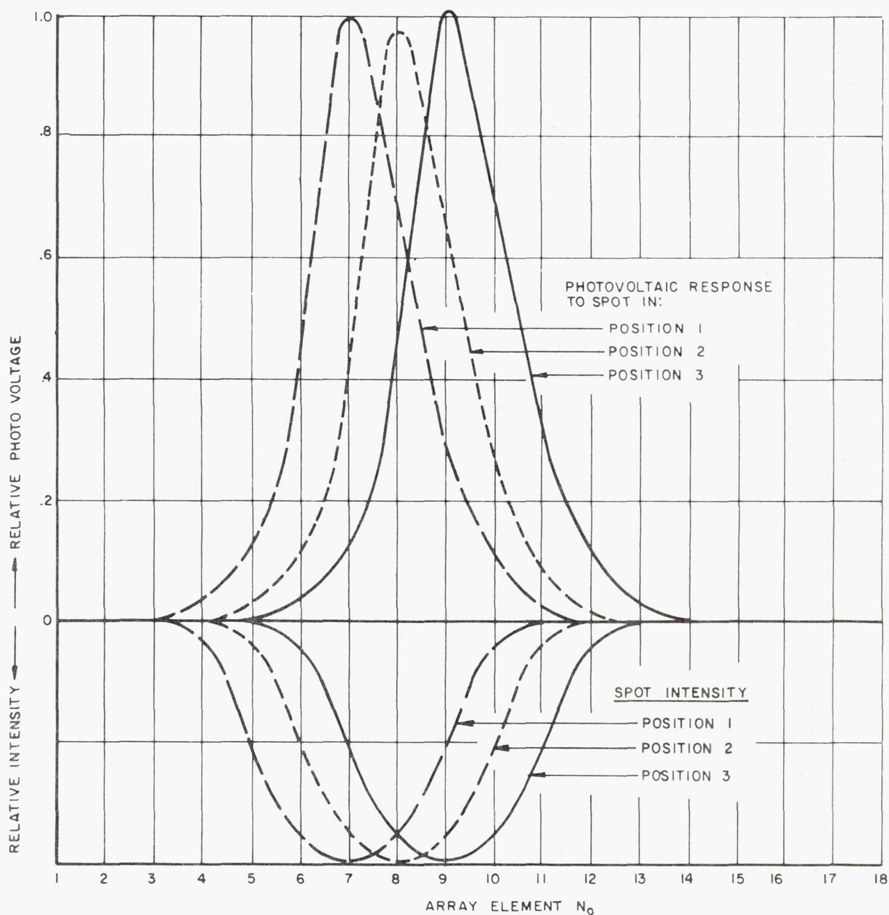
Figure 38. Array Element Isolation Measurement Results
