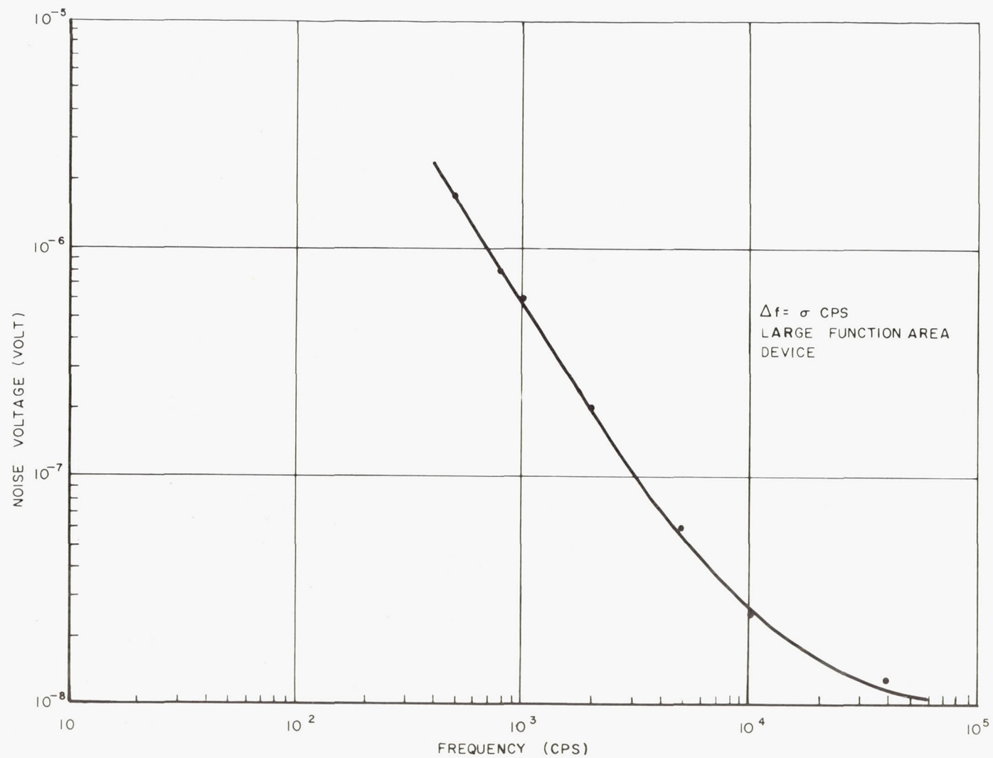
Figure 29. Noise Voltage as a Function of Frequency at 100°K for Sample #34-A
