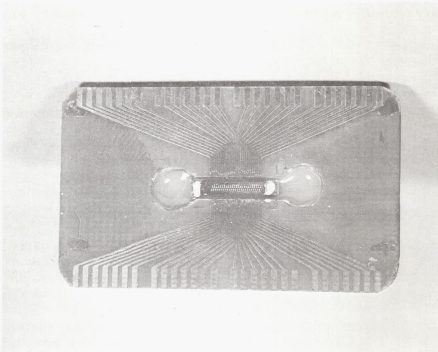
Figure 55. Electrical Connection from Array to Fanout Pattern
