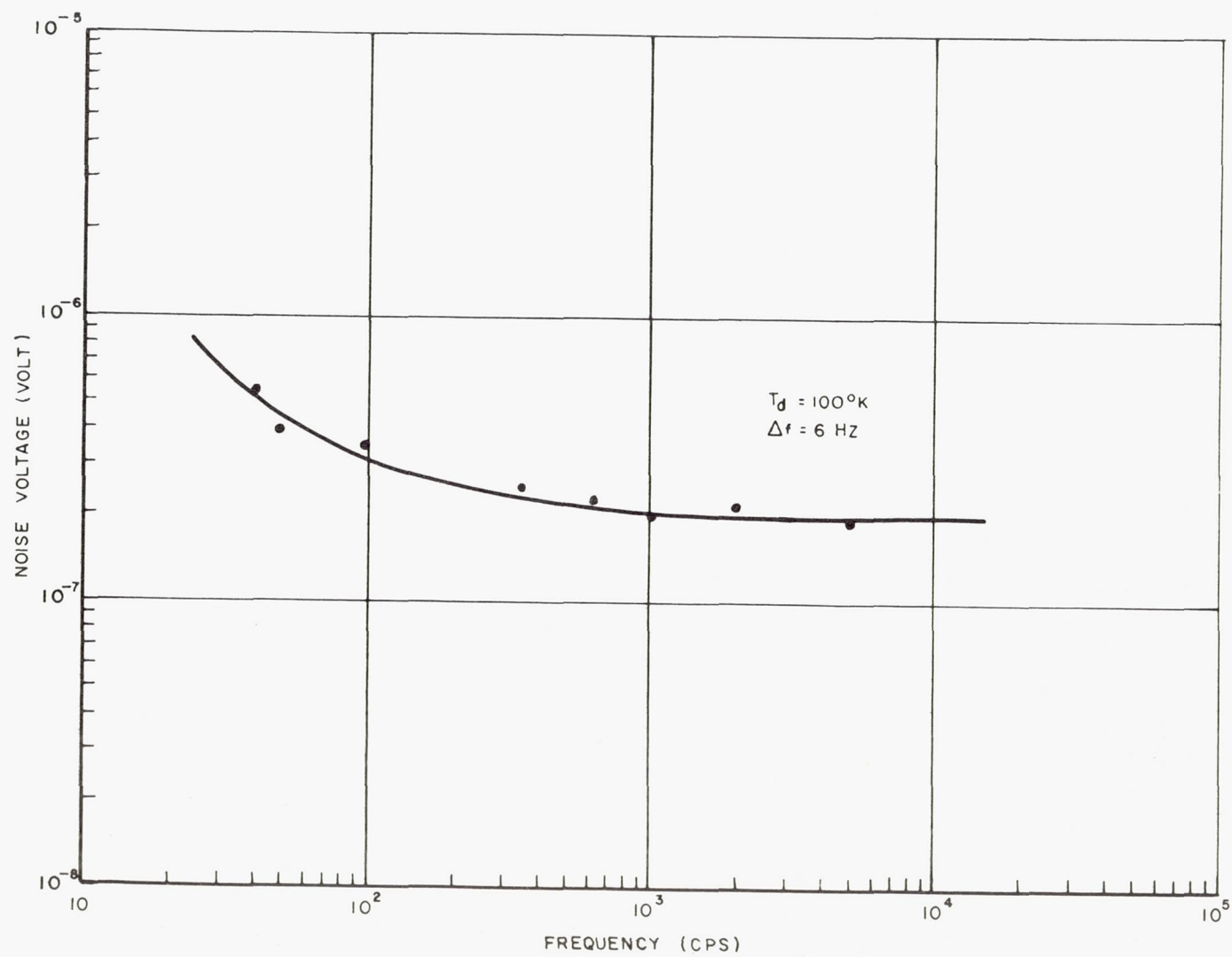
Figure 31. Noise Voltage versus Frequency for an Array Element Detector
