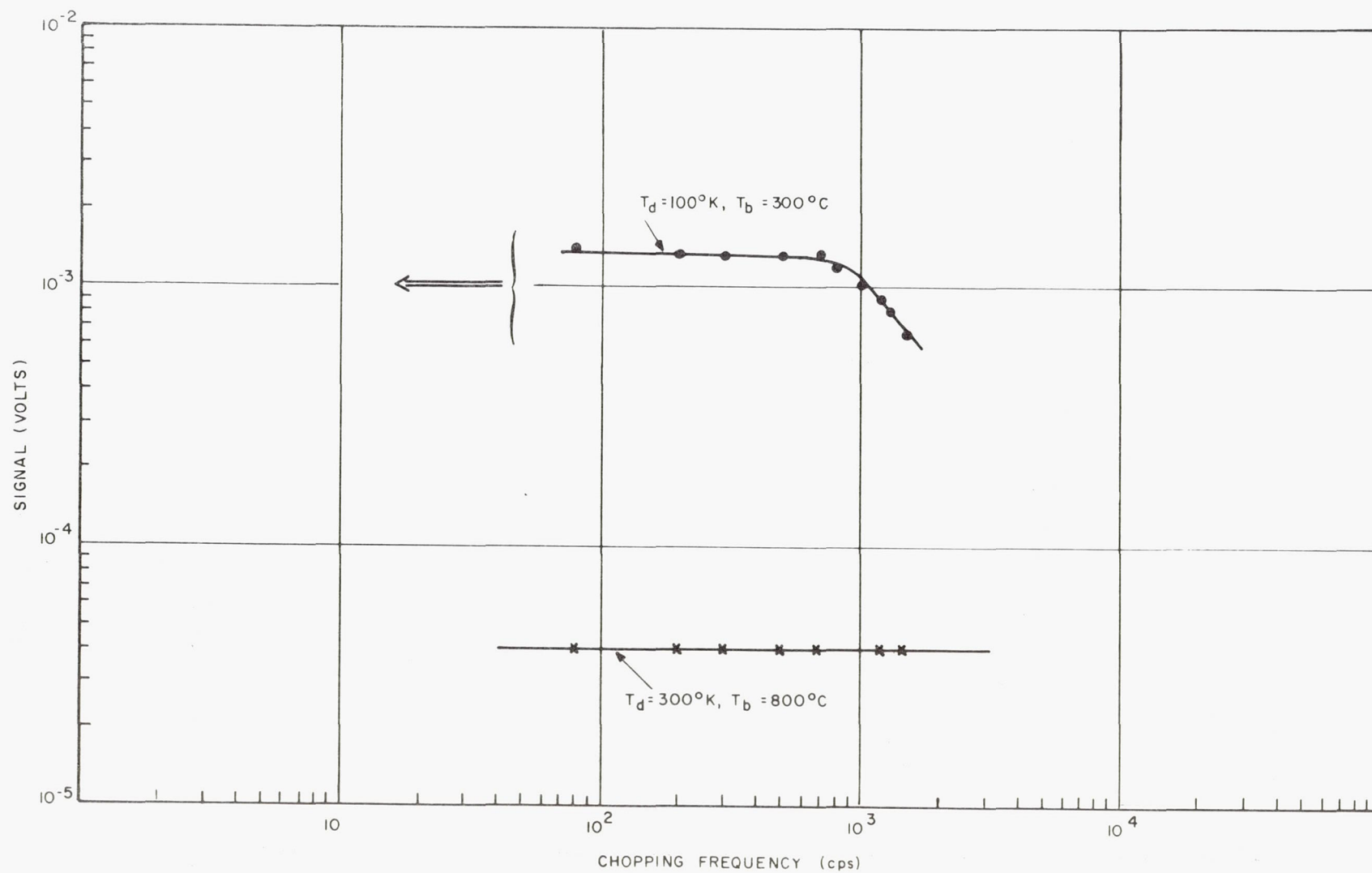
Figure 34. Signal Voltage versus Chopping Frequency
