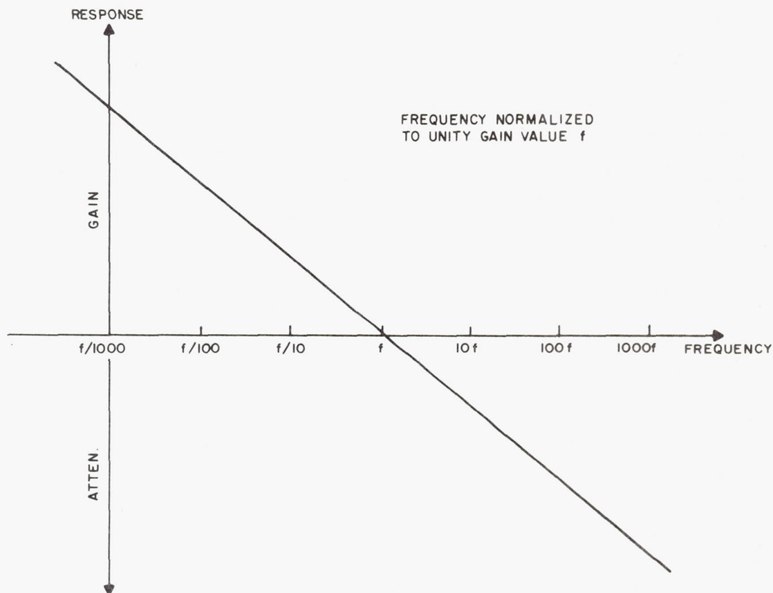
Figure 49. Frequency Response of Integrating Scheme
