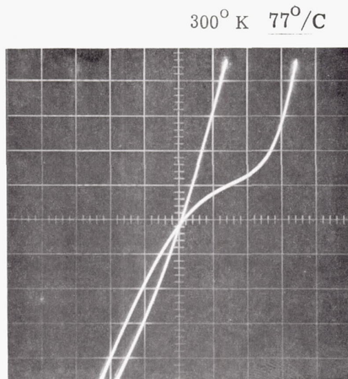
Figure 8. V-I Characteristic of Diode Diffused With Straight Cd. (Scale: V=20\text{ ma/div.} H=0.1\text{ volt/div.} )
