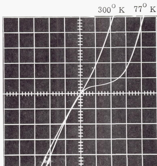
Figure 9. V-I Characteristic of Diode Diffused With 50% Cd. (Scale: V=10\text{ ma/div.} H=0.1\text{ volt. div.} )
