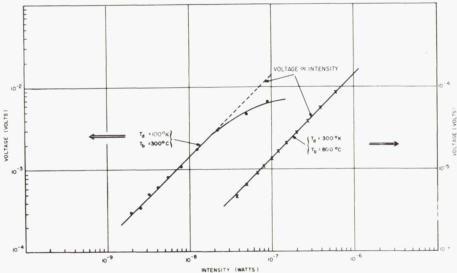
Figure 33. Photoresponse versus Radiation Intensity ( T_d = detector temperature; T_b = blackbody temperature)
