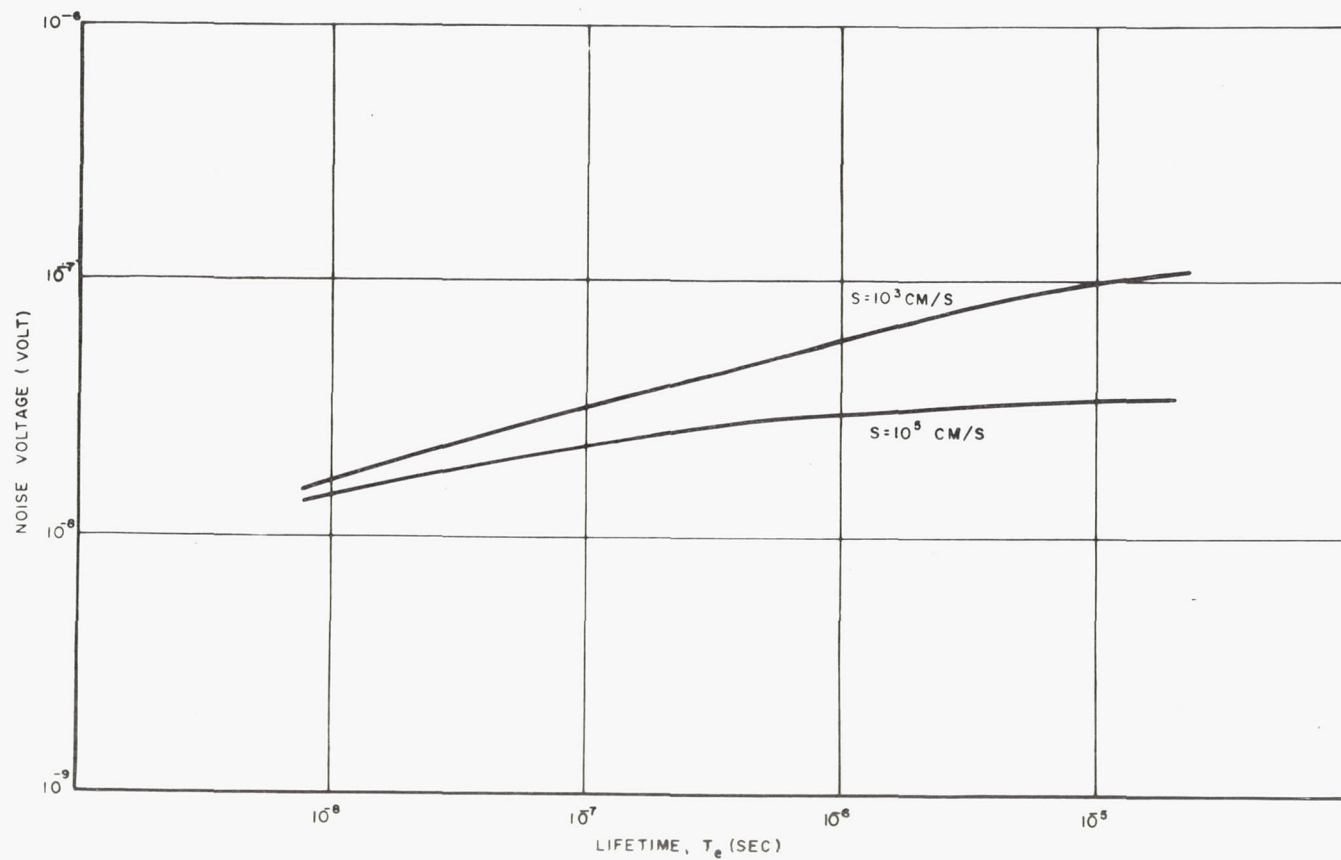
Figure 4. Noise Voltage versus Lifetime for the Optimum Junction Depth
