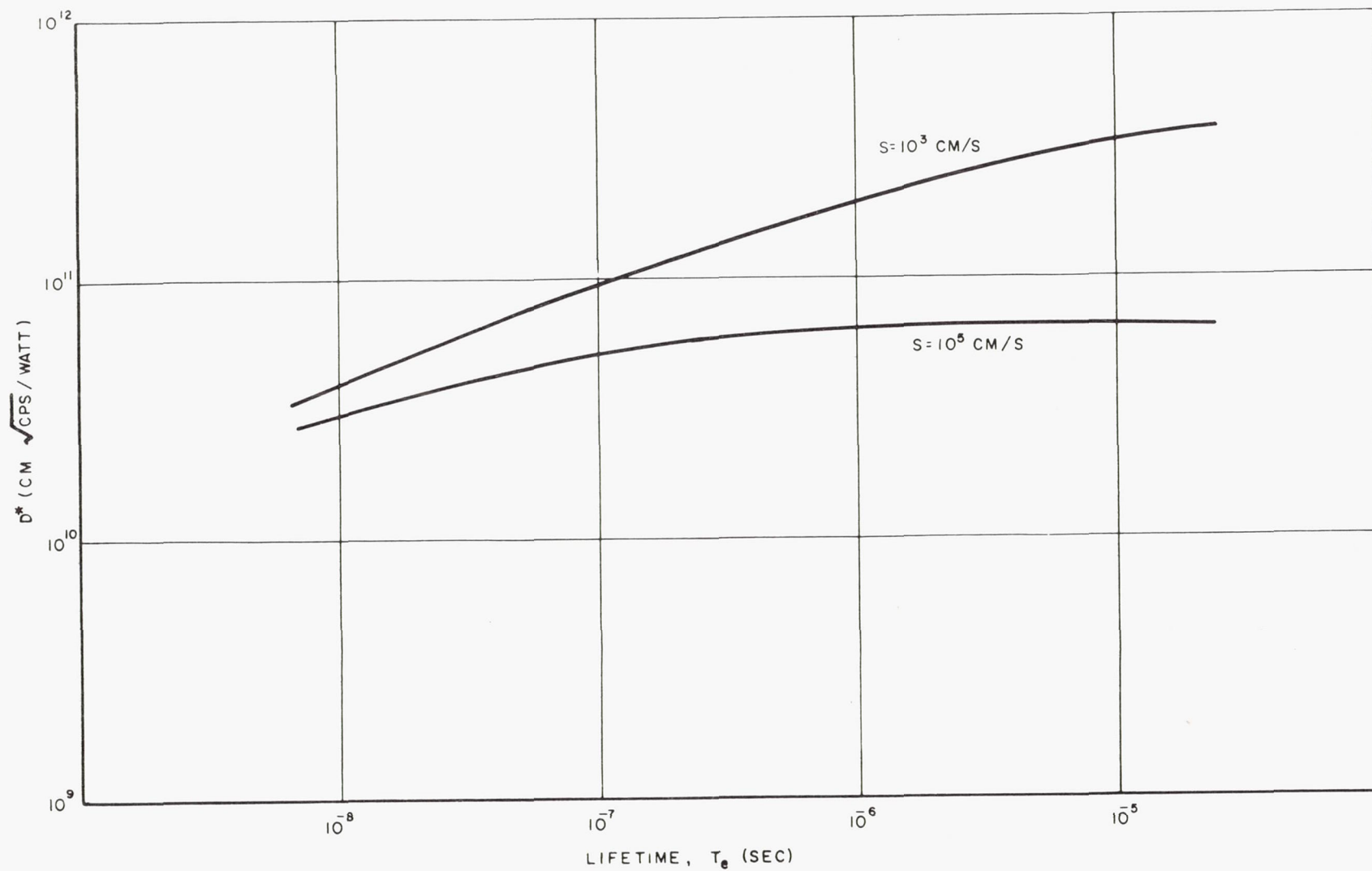
Figure 5. D^* versus Lifetime for Optimum Junction Depth
