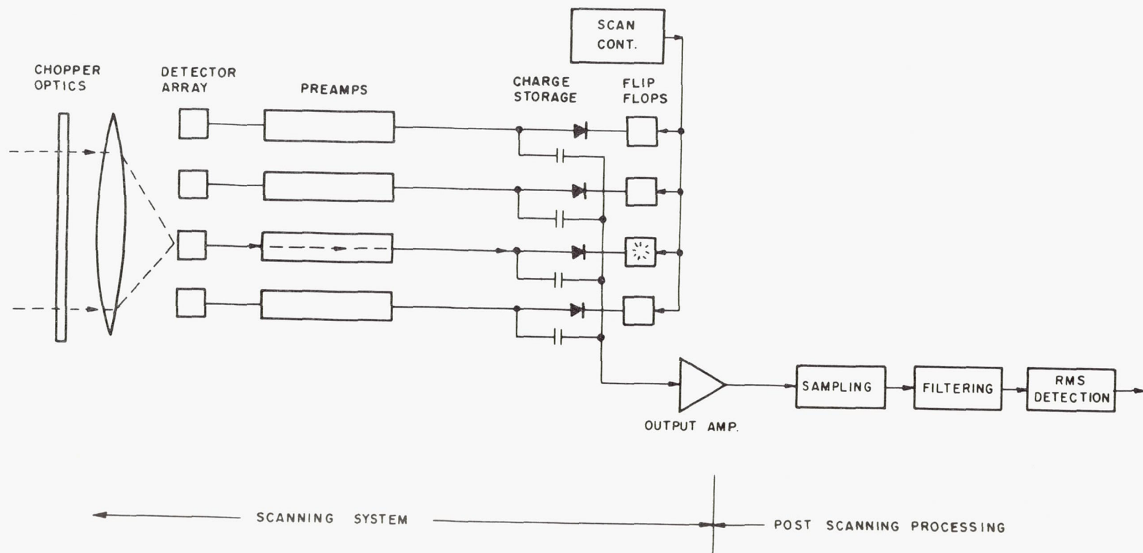
Figure 48. Operating System Diagram
