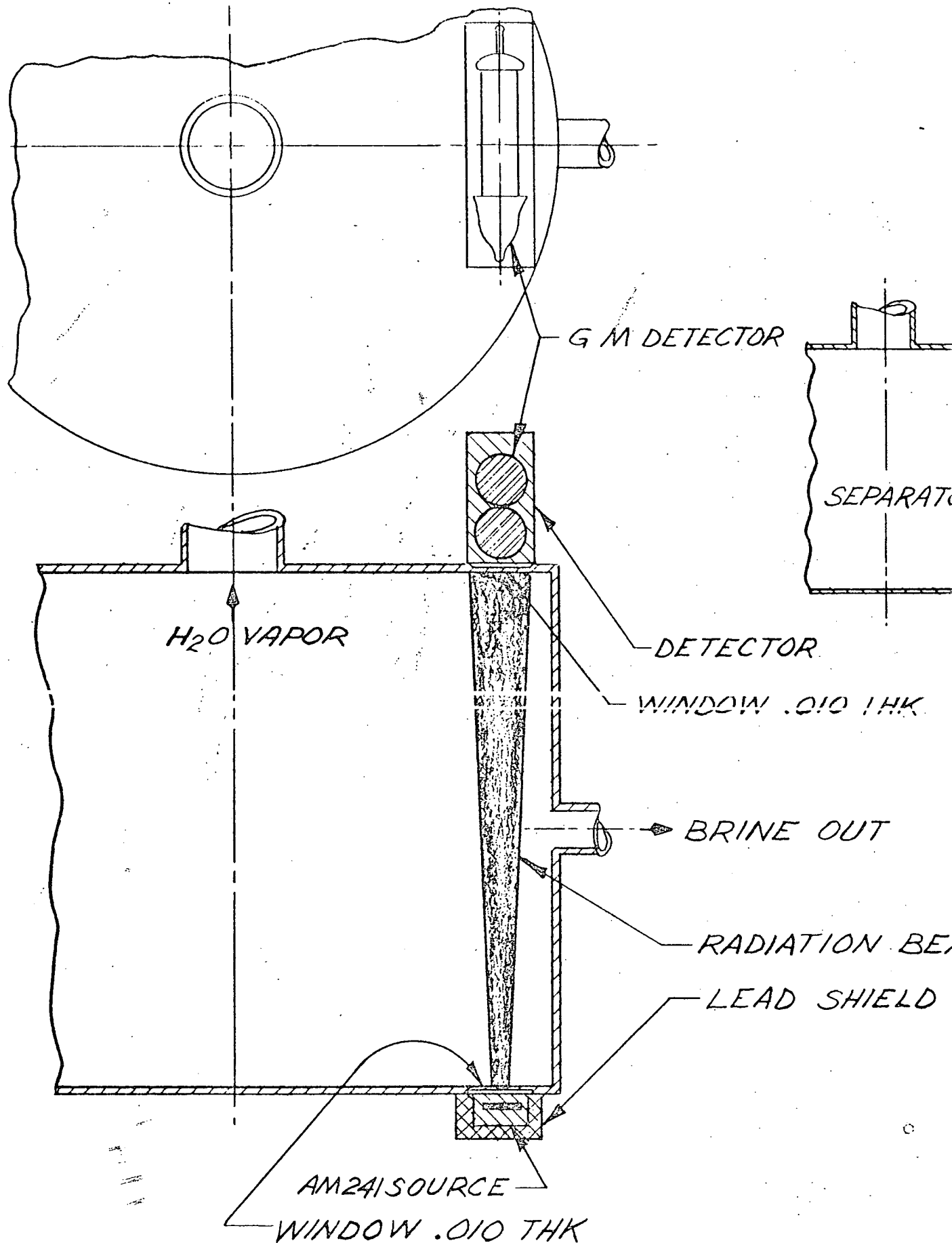
SEPARATOR CONFIGURATION
