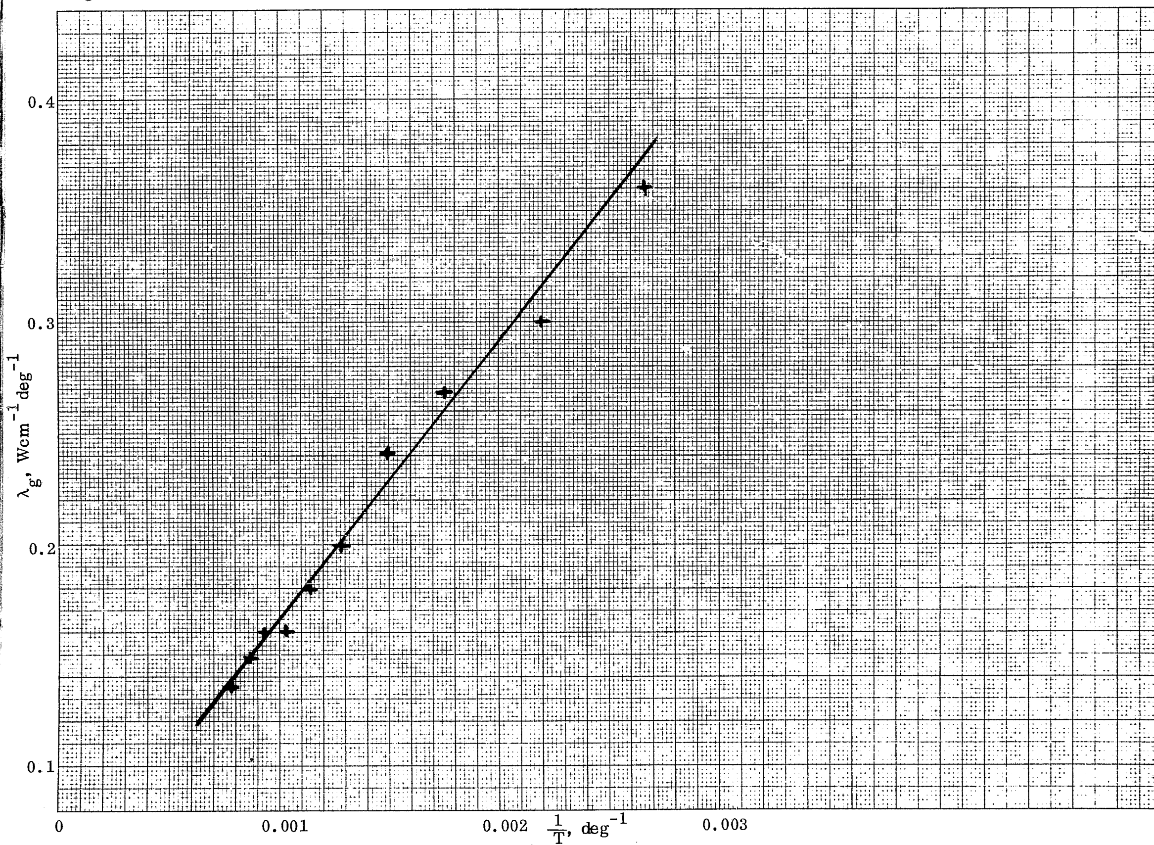
Figure 4. Lattice Component of Thermal Conductivity \gamma Reciprocal of Absolute Temperature for Hot Pressed Beryllium
