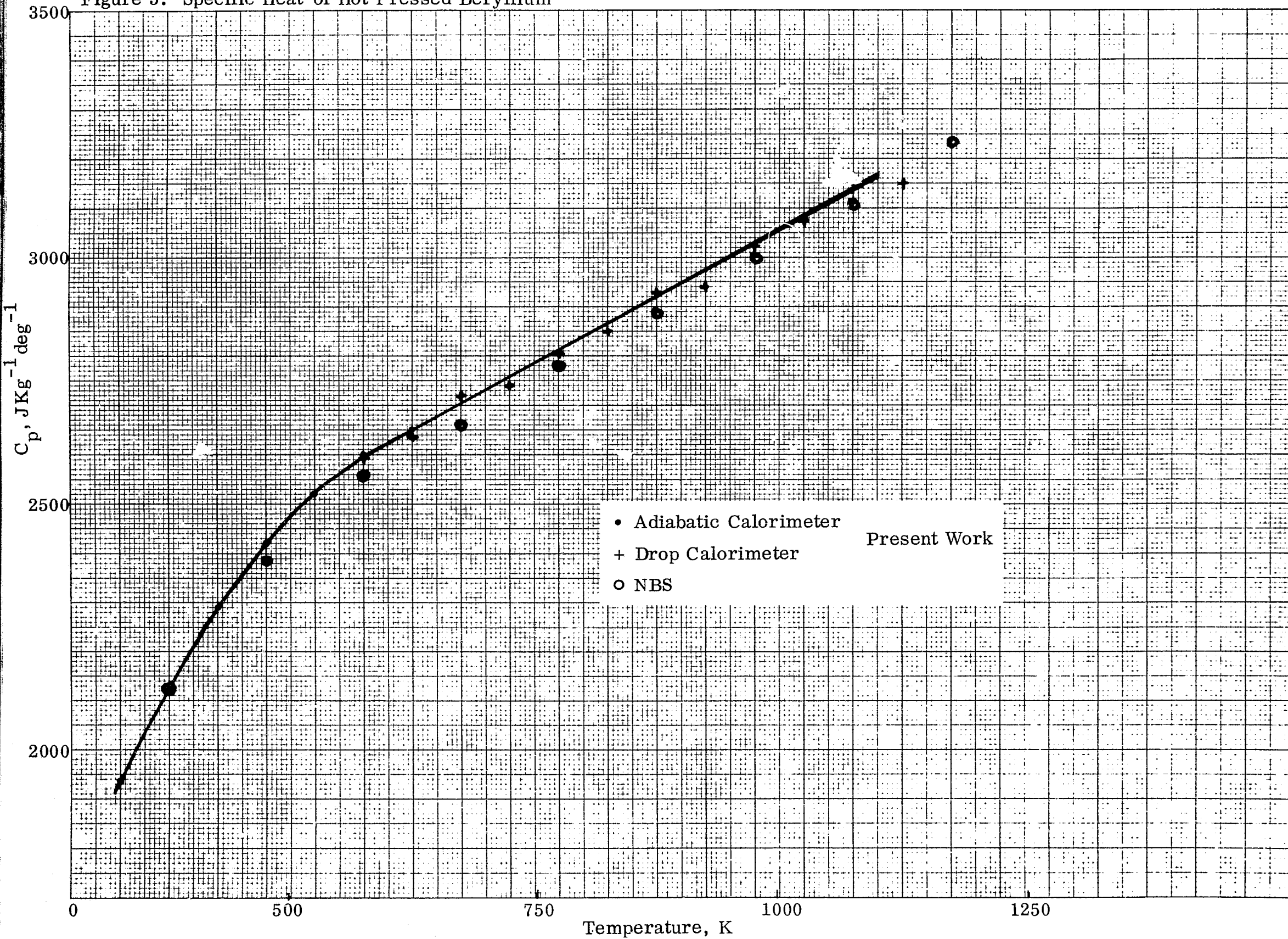
Figure 5. Specific Heat of Hot Pressed Beryllium
