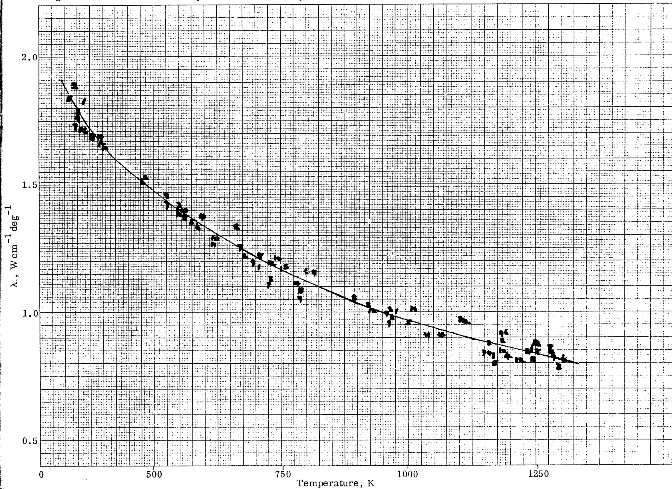
Figure 2. Thermal Conductivity of Hot Pressed Beryllium
