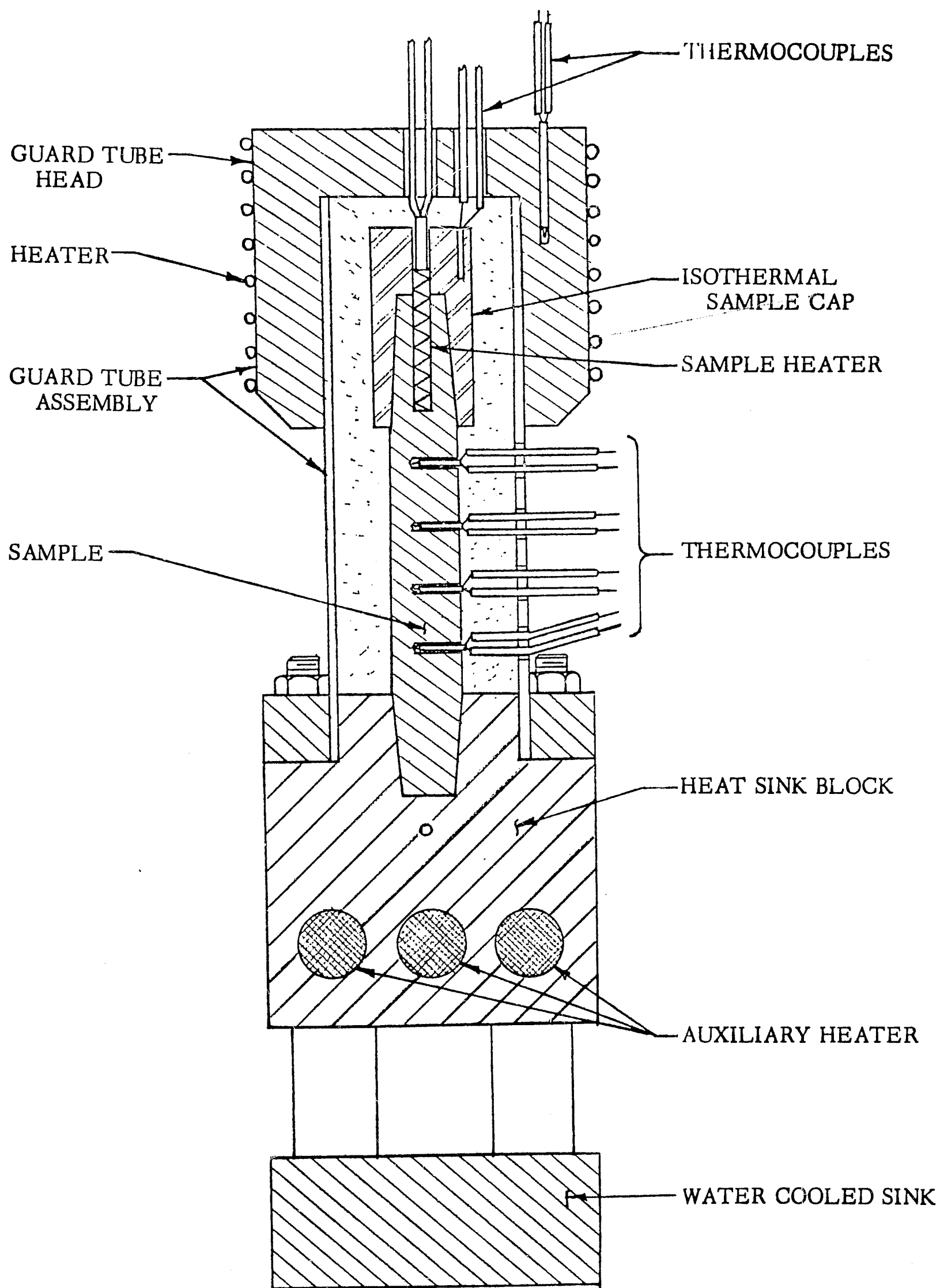
DYNATECH ABSOLUTE AXIAL ROD TESTER THERMAL CONDUCTIVITY APPARATUS
