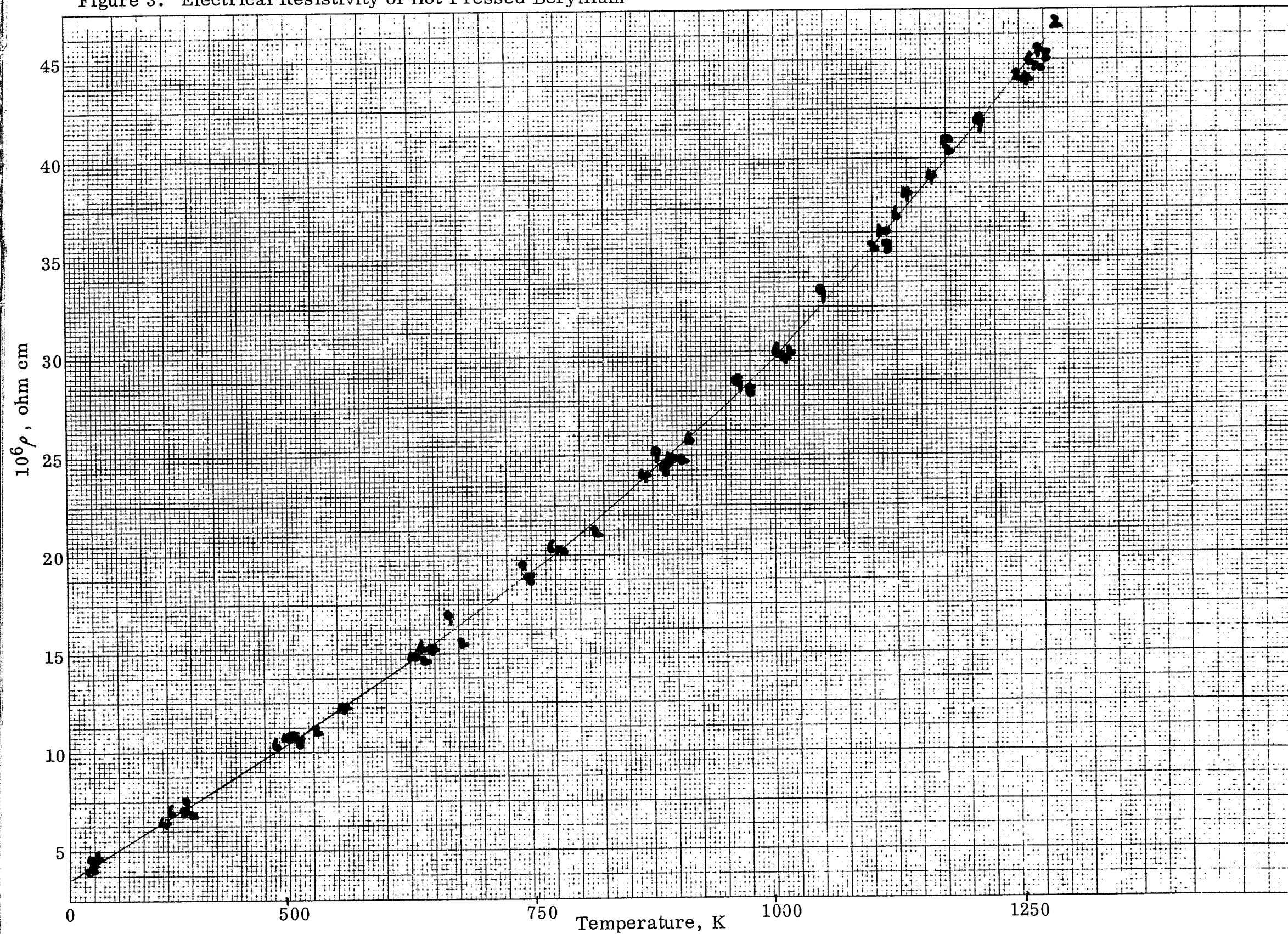
Figure 3. Electrical Resistivity of Hot Pressed Beryllium
