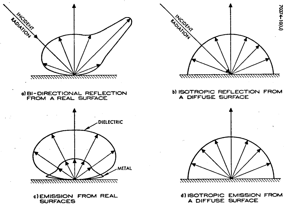
Figure 2. Schematic Comparison of Reflection and Emission From Real and Ideal (Diffuse) Surfaces
