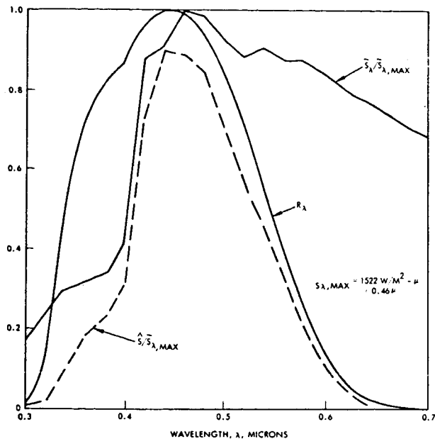
Figure 6. Approximate Solar Spectrum \tilde{S}_\lambda for Air Mass \approx 1.2 ; Spectral Response, R_\lambda , of S-11 Photomultiplier; Apparent Solar Spectrum, \hat{S}_\lambda = \tilde{S}_\lambda R_\lambda , for Photometric Tests
