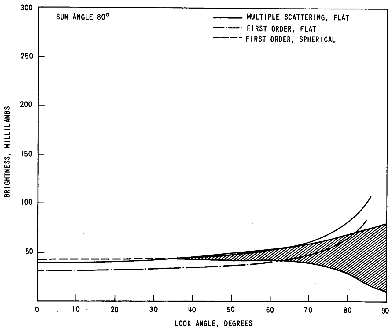
FIGURE 17 - THE BRIGHTNESS AS A FUNCTION OF LOOK ANGLE FOR A FIXED SUN ANGLE OF 80°. THE CROSS-HATCHED AREA REPRESENTS THE RANGE OF VALUES ARISING FROM THE AZIMUTHAL DEPENDENCE IN THE FIRST ORDER SPHERICAL CALCULATIONS.
