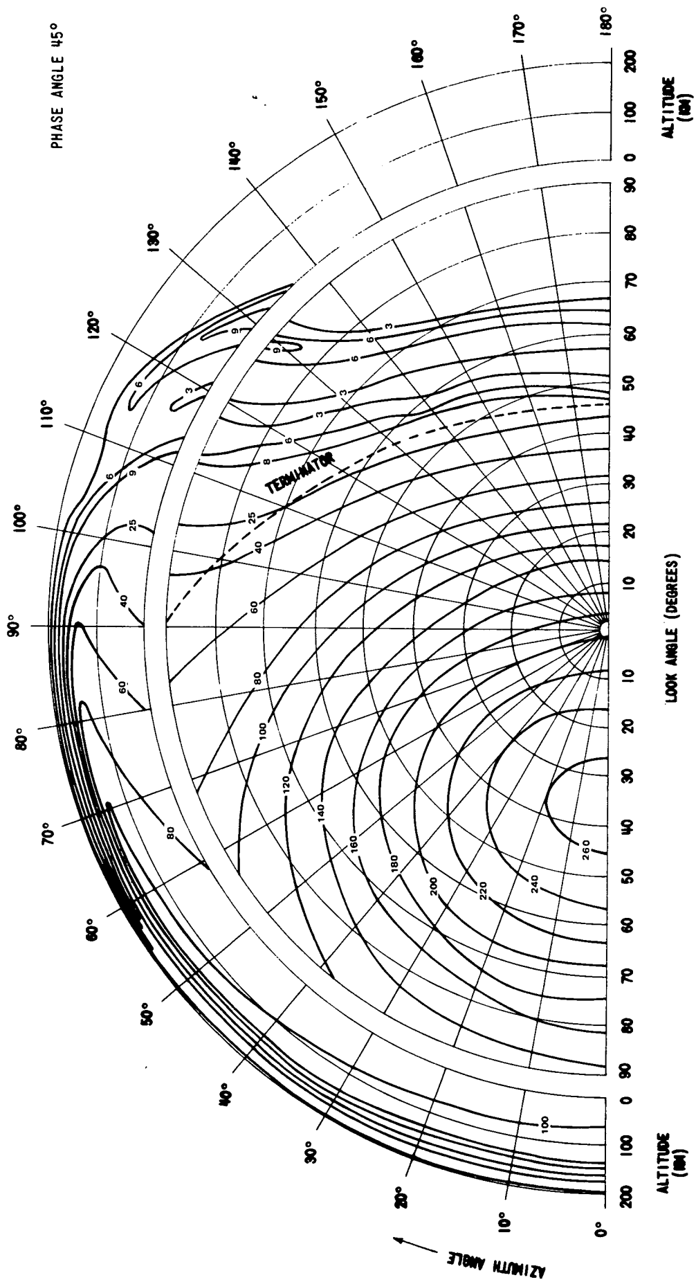
FIGURE 20 - ISO-BRIGHTNESS CONTOURS. THE UNITS OF BRIGHTNESS ARE MILLILAMBS
