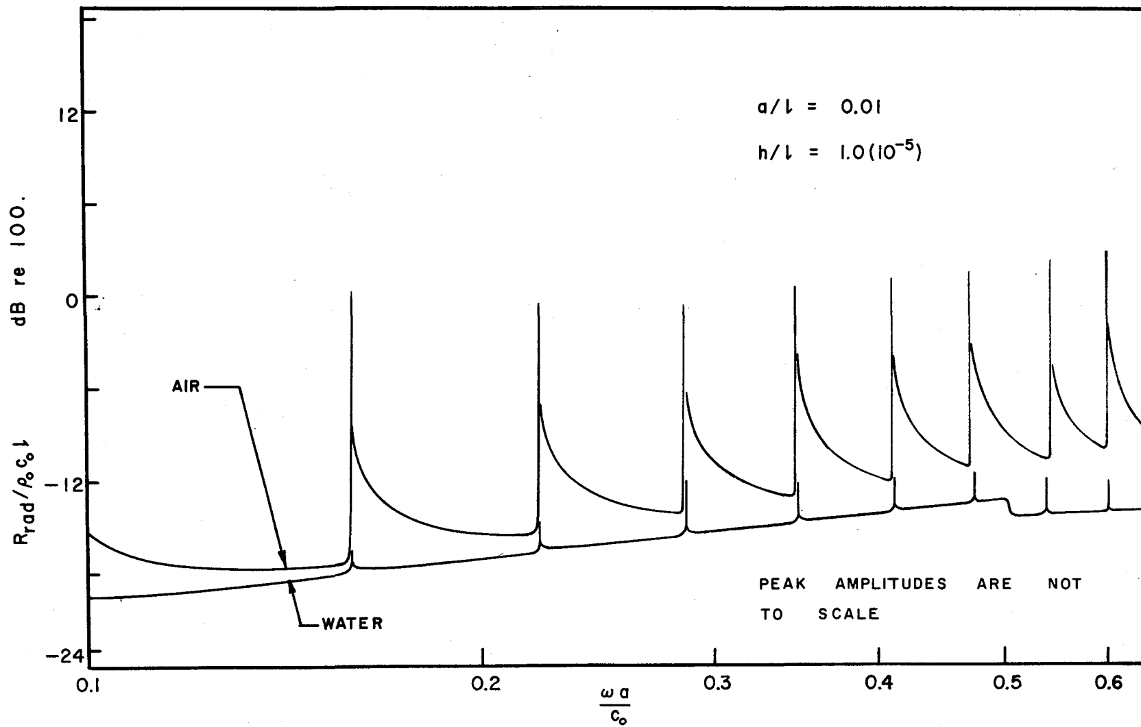
FIGURE 5.3 DIMENSIONLESS RADIATION RESISTANCE VS (\frac{\omega a}{c_0})
