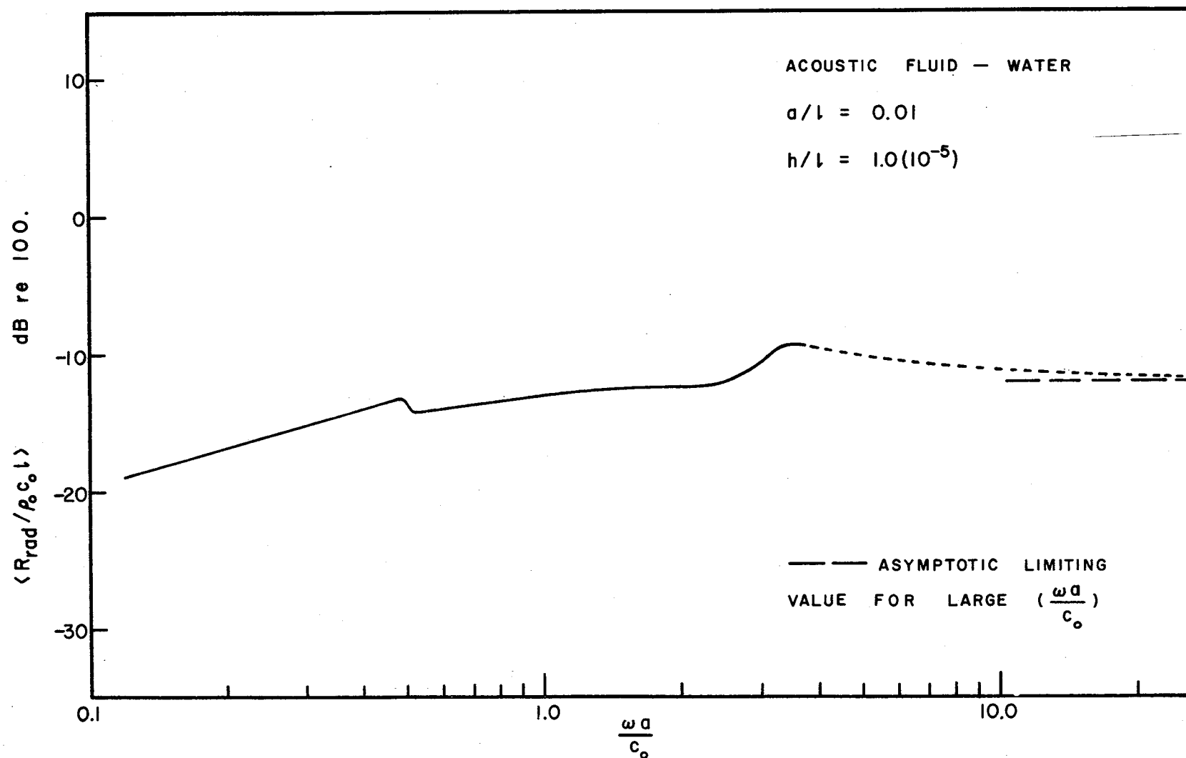
FIGURE 5.4 AVERAGED DIMENSIONLESS RADIATION RESISTANCE VS (\frac{\omega a}{c_0})
