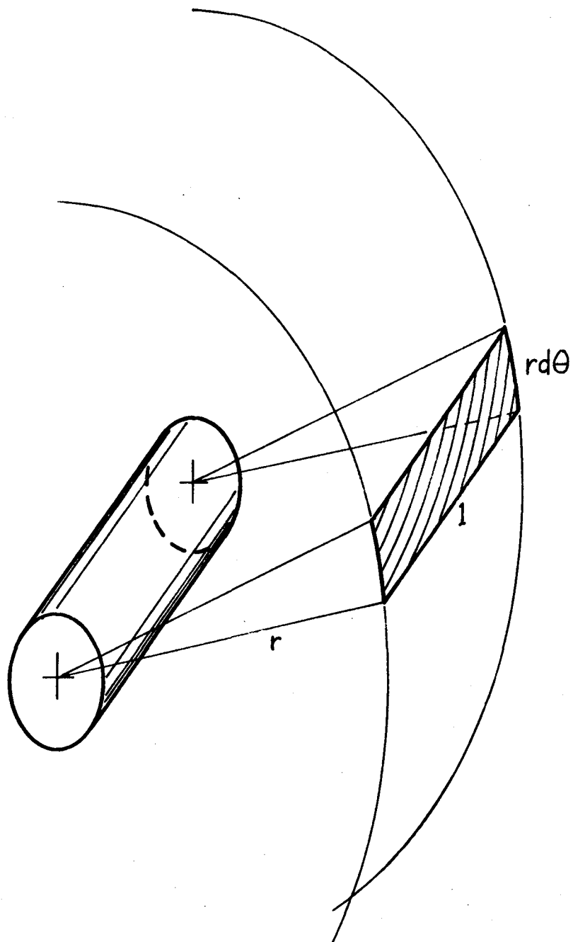
FIGURE 4.2 SCHEMATIC OF ACOUSTIC FIELD AREA INTO WHICH VIBRATORY ENERGY IS RADIATED BY THE CYLINDER
