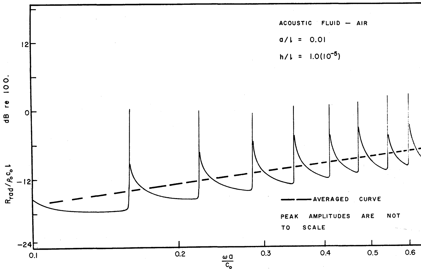
FIGURE 5.1 DIMENSIONLESS RADIATION RESISTANCE VS (\frac{\omega a}{c_0})
