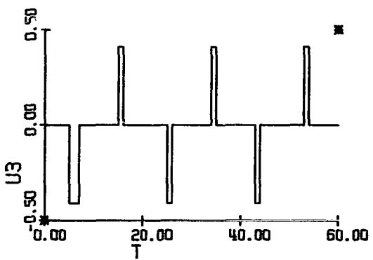
Figure 5-2b Response to 18-Pulse Nominal Control Applied to Initial Conditions of Run R-1
