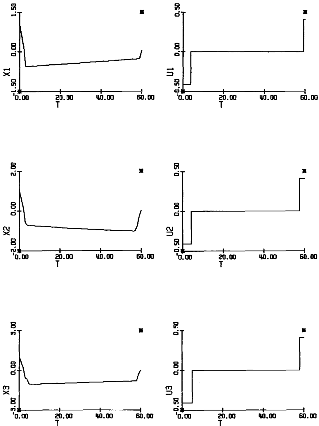
Figure 5-3b Optimal Response For Initial Conditions of Run R-1; U_i = .412 \text{ deg./sec}^2 ; t_f = 60 \text{ sec}
