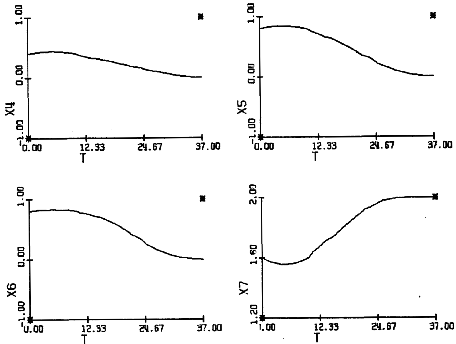
Figure 6-2a Approximate Time Optimal; t_F = 37 sec
