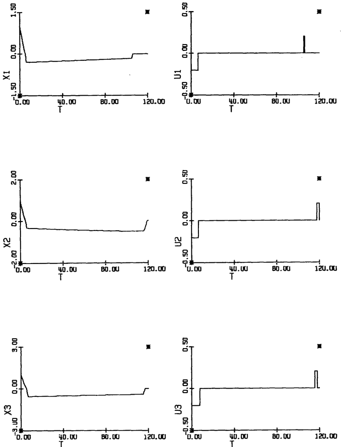
Figure 5-6b Optimal Response for Run R-1 with U_i = .206 \text{ deg./sec}^2 and with t_f = 120 \text{ sec}
