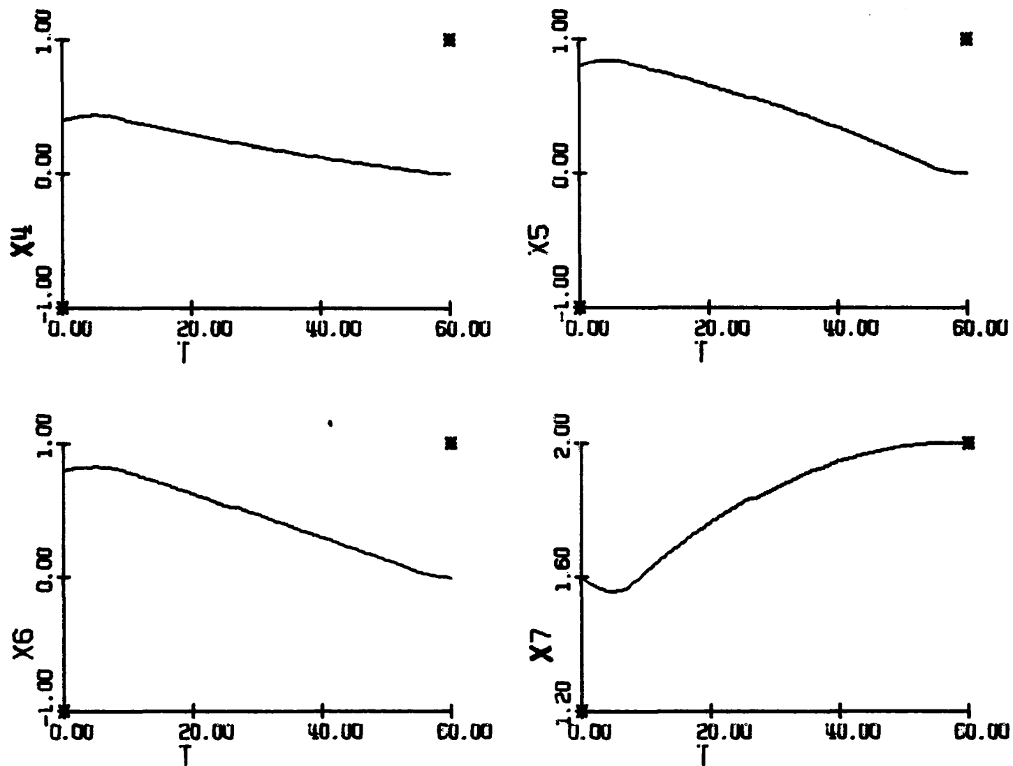
Figure 5-4a. Optimal Response For Initial Conditions of Run R-1; U_1 = .206 \text{ deg./sec}^2 ; t_f = 60 \text{ sec} .
