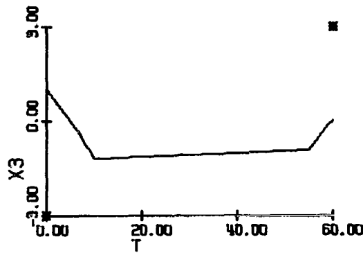
Figure 5-4b Optimal Response For Initial Conditions of Run R-1; U_i = .206 \text{ deg./sec}^2 ; t_f = 60 \text{ sec}
