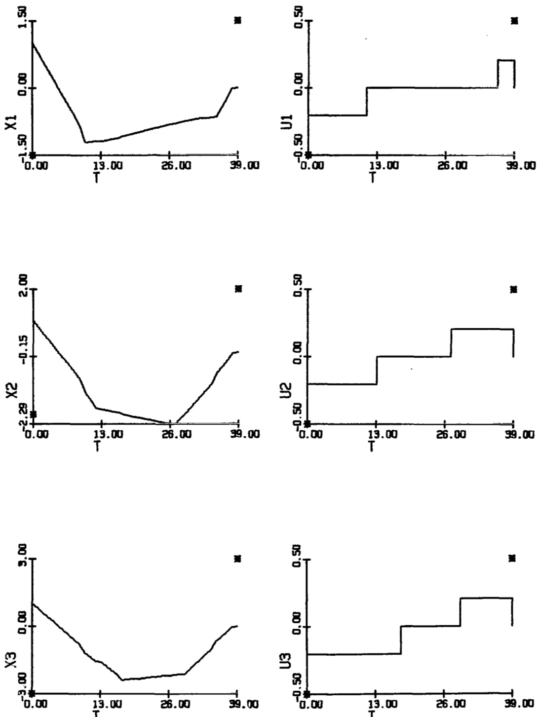
Figure 6-1b Optimal Response for Run R-1 with U_i = .206 \text{ deg./sec}^2 and t_f = 39 \text{ sec}
