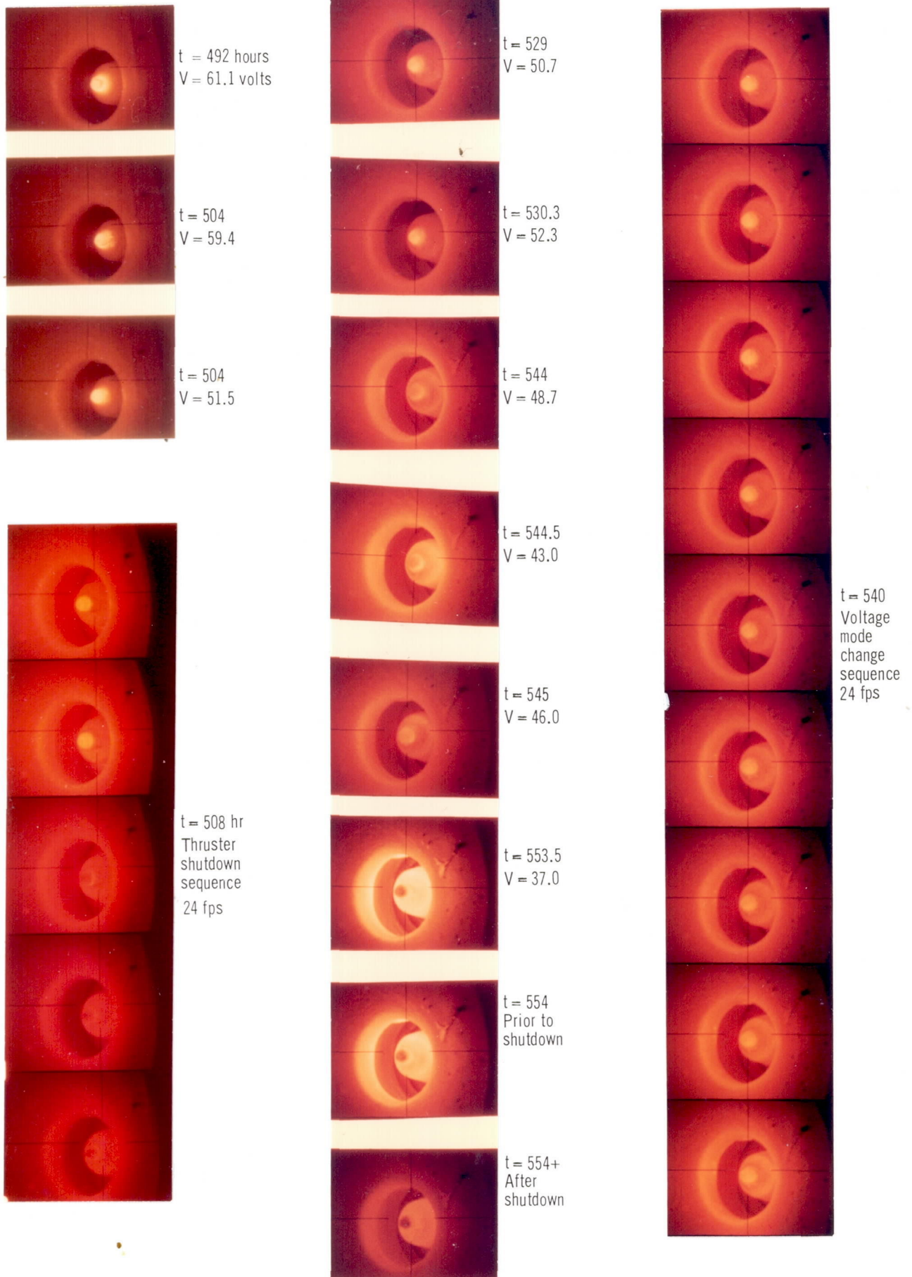
Fig. 3.16 Photographs of arc discharge during lifetest MCDONNELL DOUGLAS
