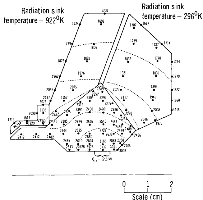
Fig. 2.2 Calculated temperature distribution in X-6 thruster for Q_{in} = 12.5 kW
