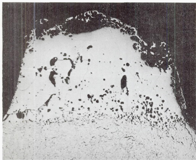
Cathode Tip
