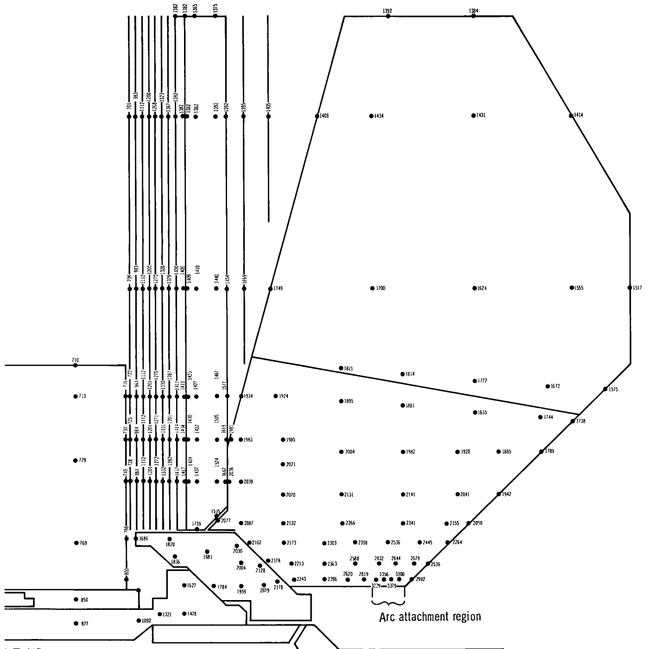
Fig. 2.8 Complete calculated temperature distribution for X-7 thruster Q_{in} = 16 kW (Continued)
