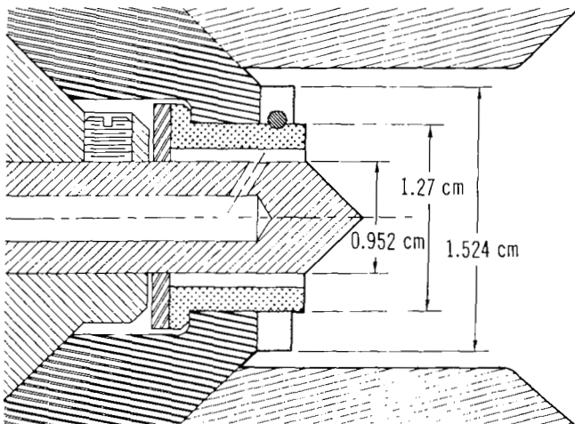
Fig. 3.8 X-7 Thruster gas shield design modification
