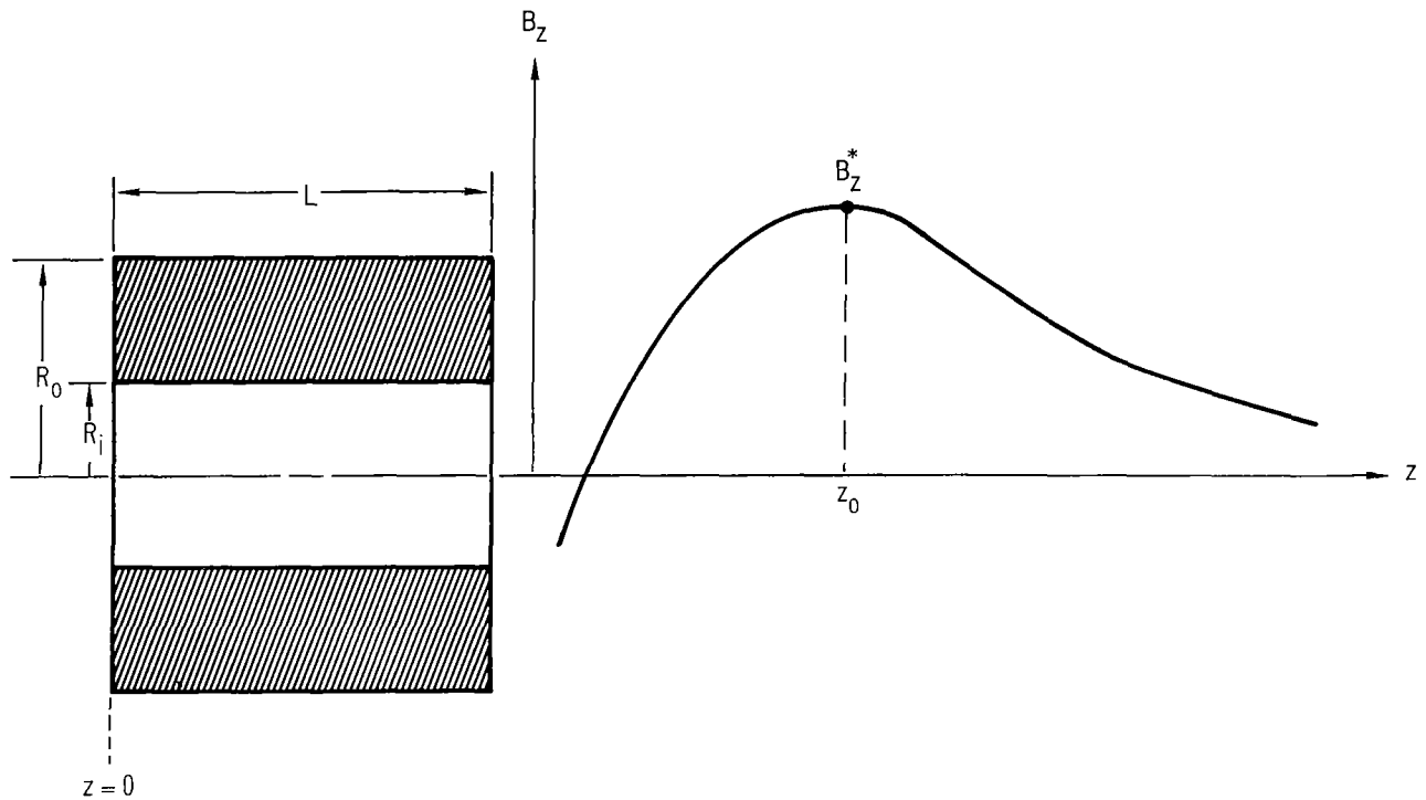
Fig. C-1 Permanent magnet geometry and centerline field distribution
