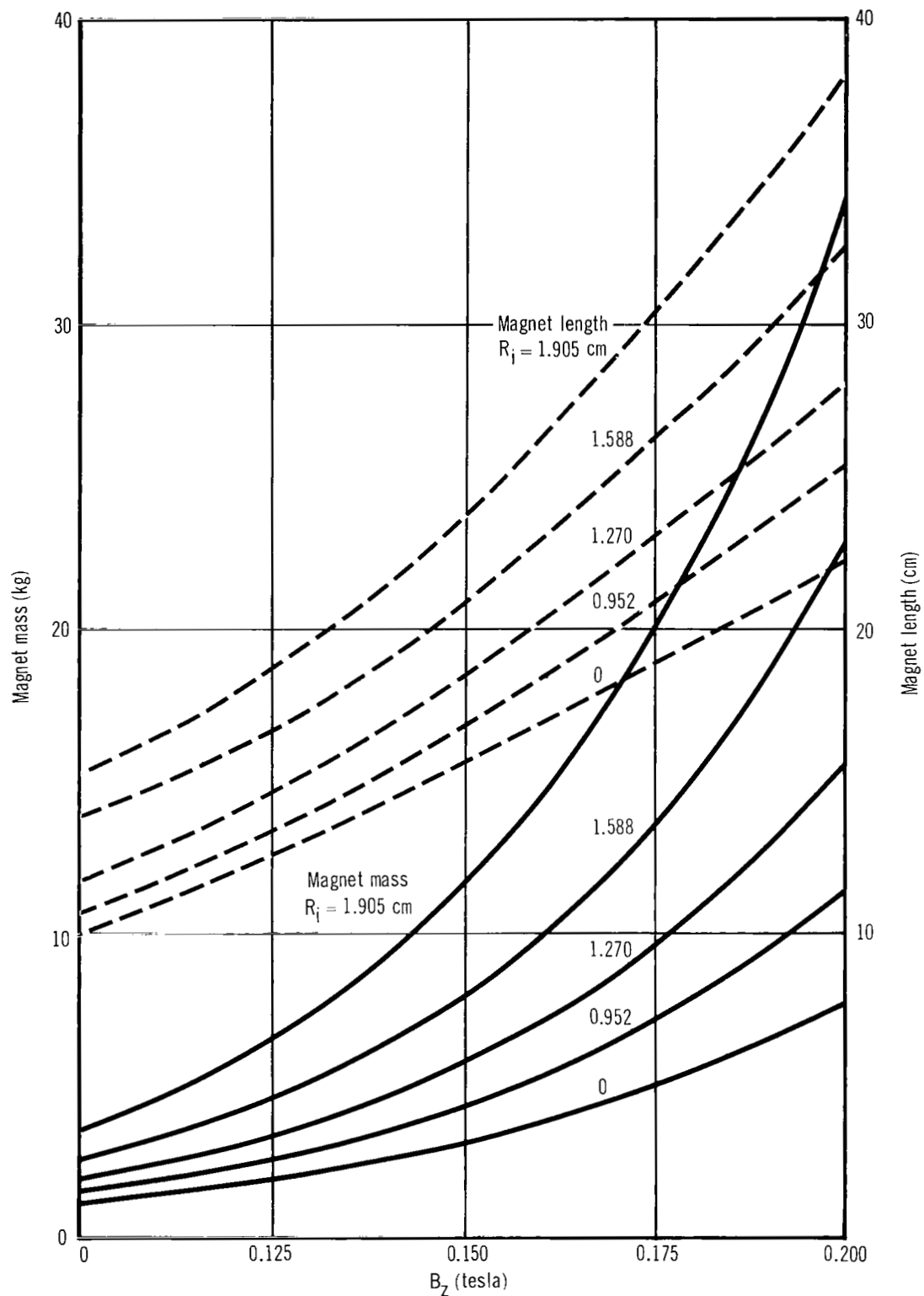
Fig. C-3 Optimum magnet mass for z = 2.54 cm (Columax-9)
