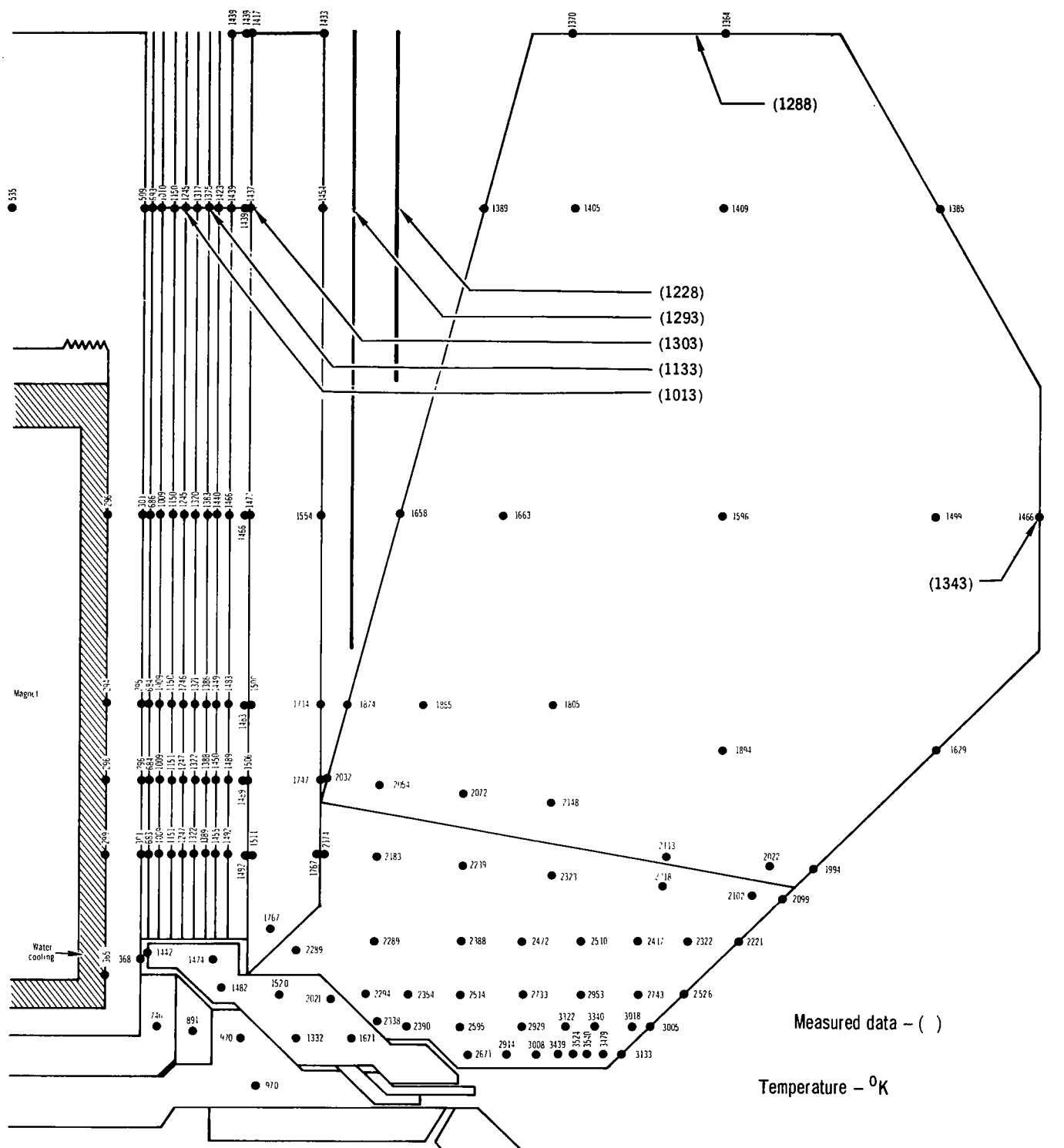
Fig. 2.7 Measured and calculated temperature distribution in X-7 thruster for Q_{in} = 16 kW
