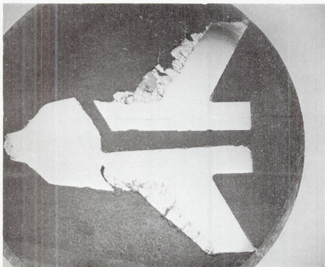
Sectioned Cathode
