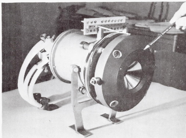
Fig. 3.3 X-7 thruster assembled
