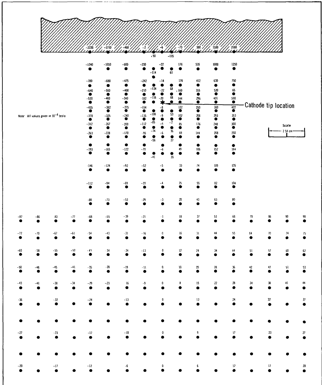
Fig. 3.5 Radial magnetic field of X-7 electromagnet ( I_{mag} = 400 amperes)
