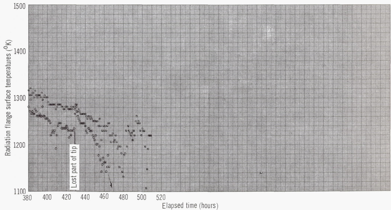
Fig. 3.27 Radiation flange temperature histogram (continued)
