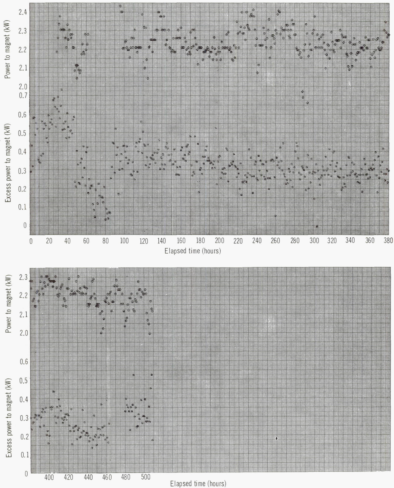
Fig. 3.28 Magnet power and excess power histogram
