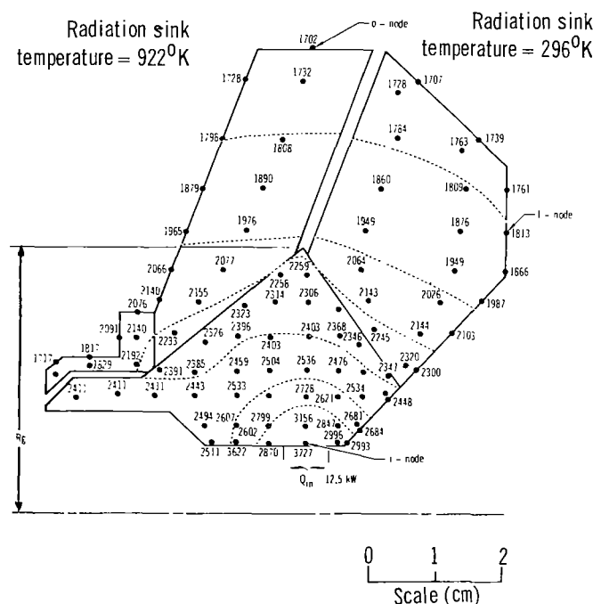
Fig. 2.3 Calculated temperature distribution in X-6 thruster for Q_{in} = 12.5 kW
