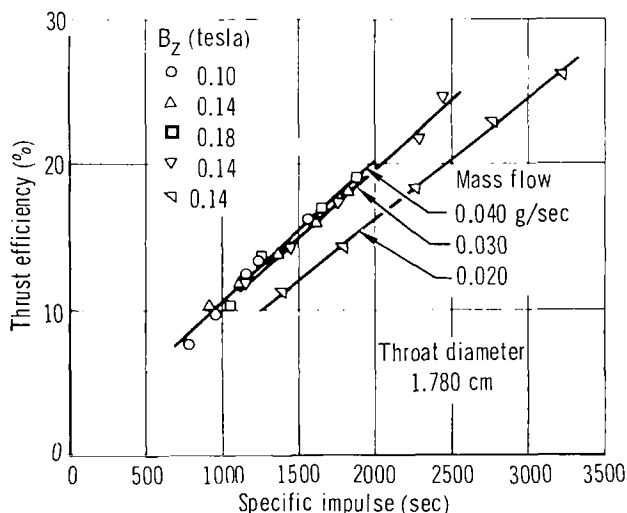
Fig. 3.7 X-7 Thrust performance
