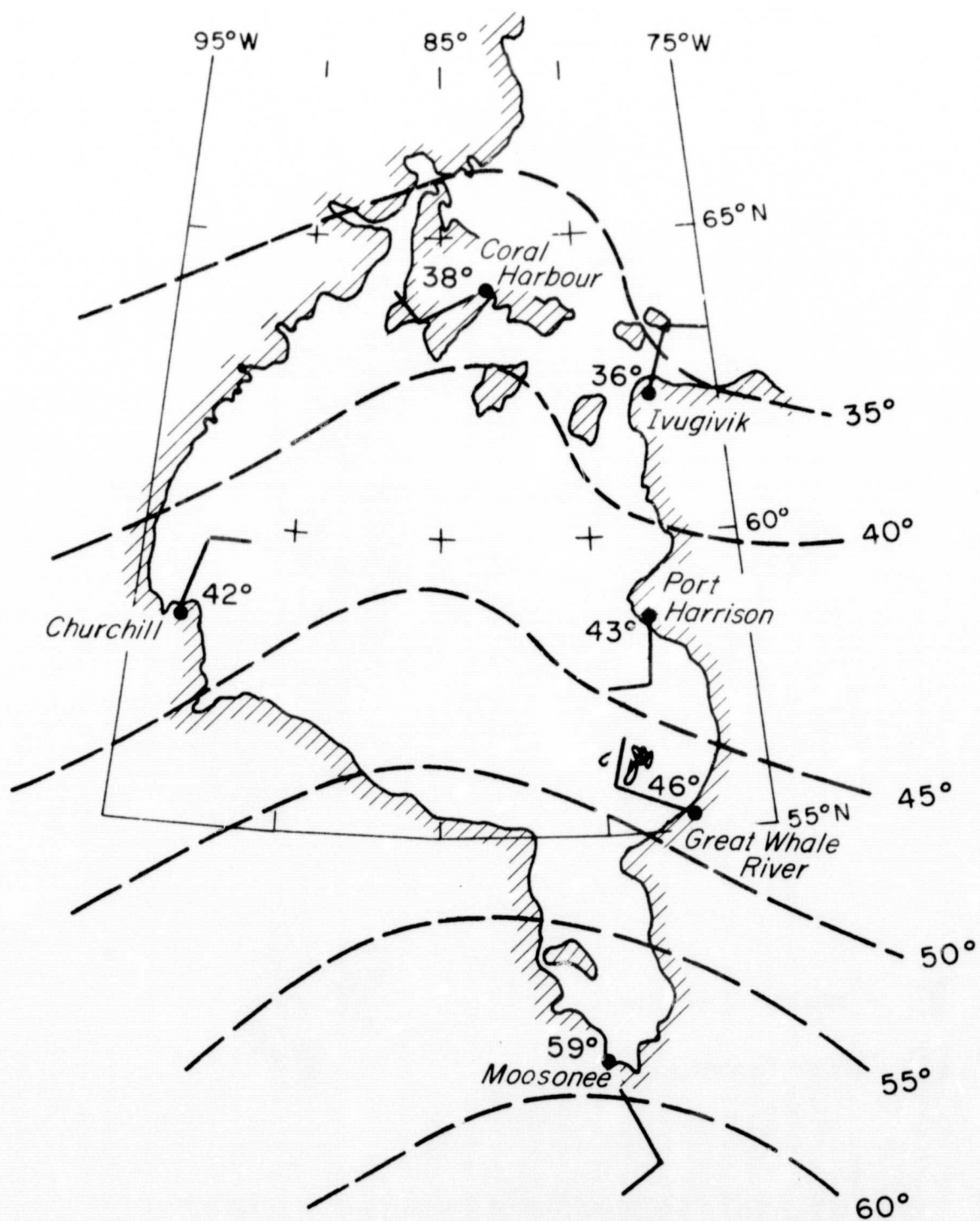
Fig. 8 Mean 1800 GMT Surface Winds and Temperatures, 1 - 15 June 1966.
