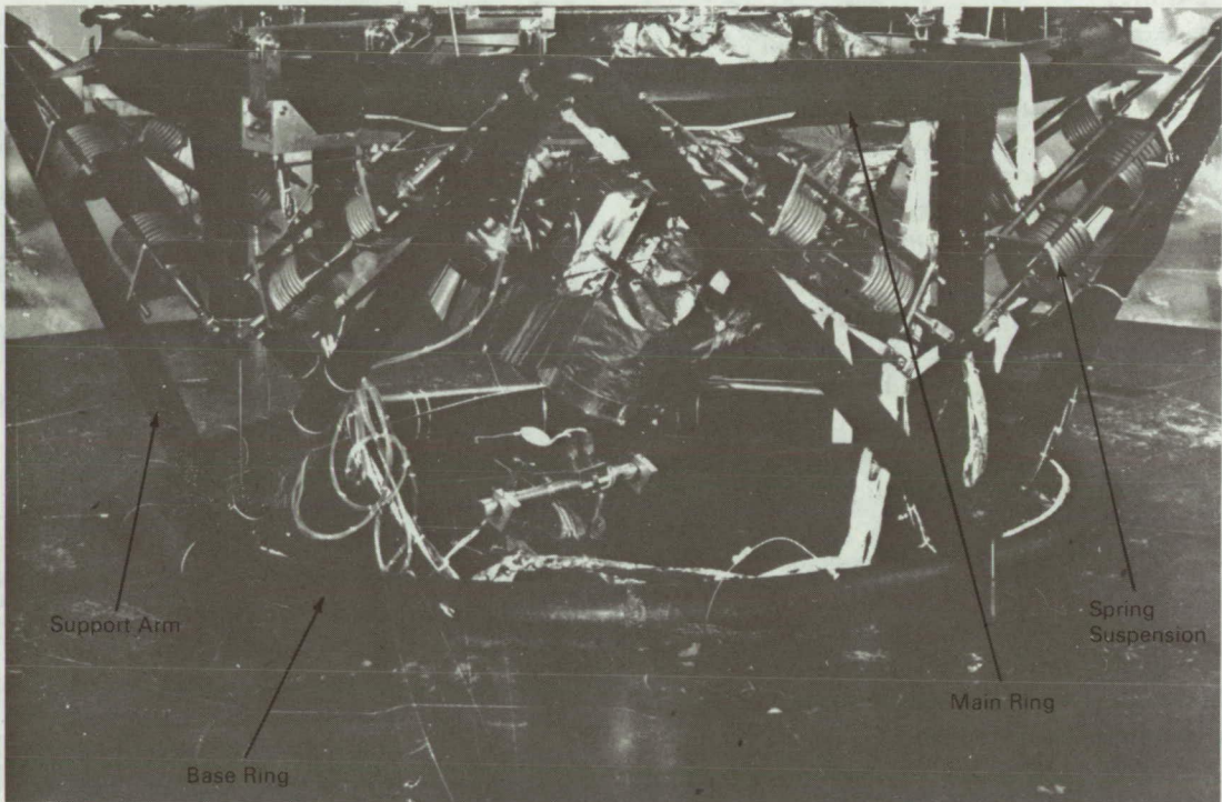
Figure 1. Test Item on Vibration Isolator
