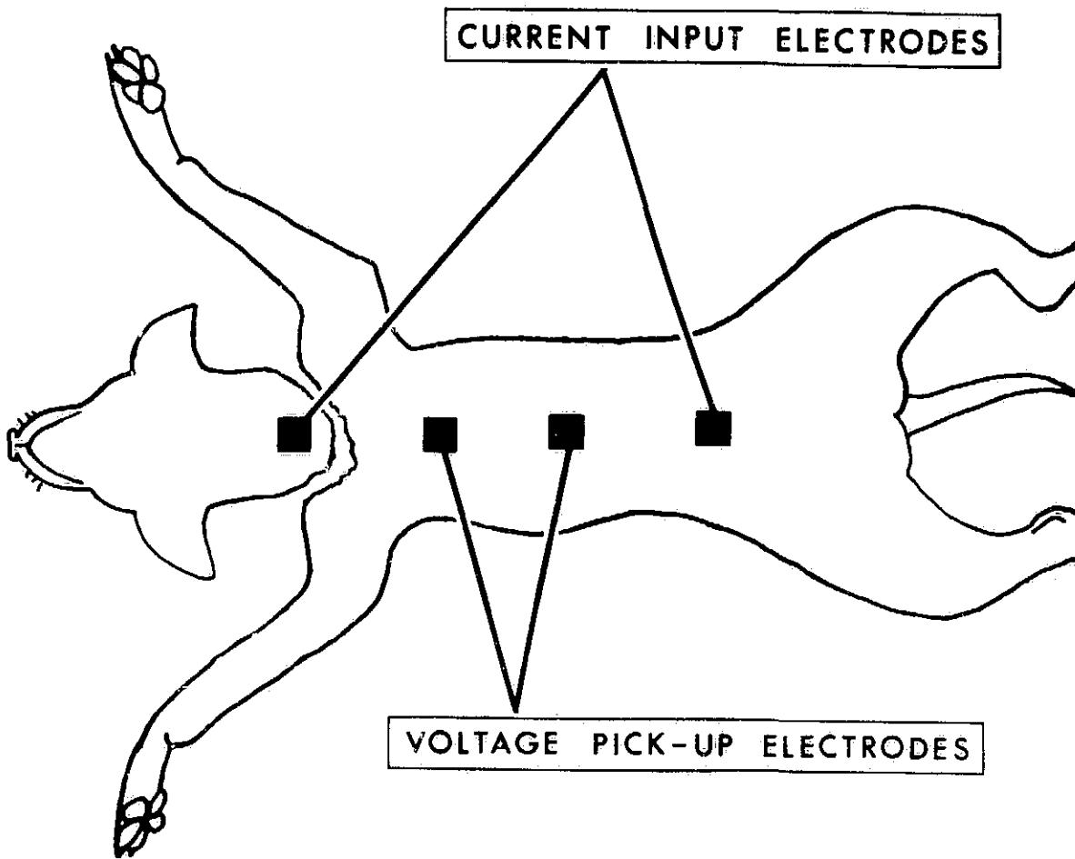
Figure 1 Electrode placement
