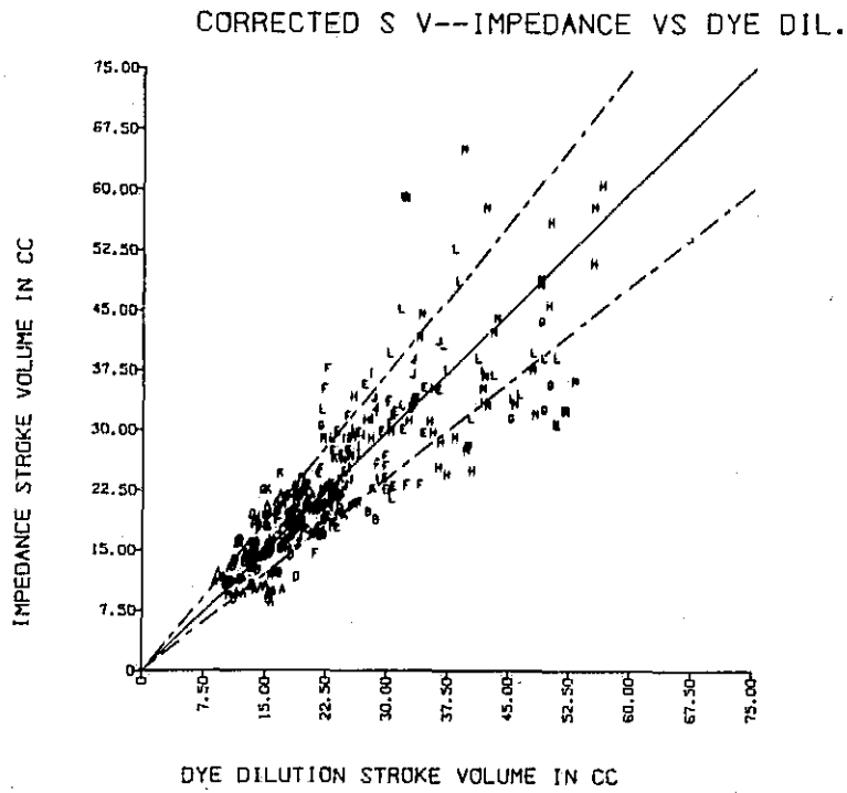
Figure 4 Comparison of simultaneous impedance and dye dilution stroke volume on 14 dogs with 45° identity time and ±20% difference band (see text for correction method of impedance data)
