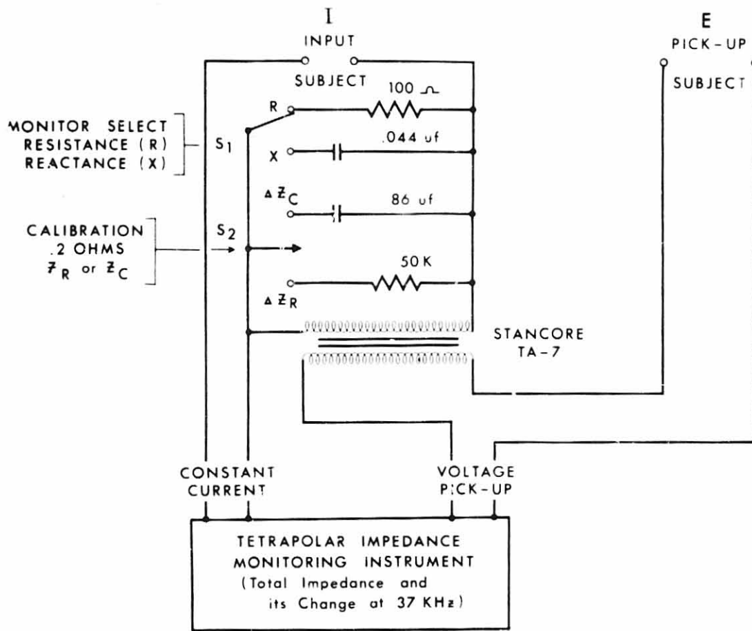
Figure 3 Circuit for monitoring resistive or reactive impedance changes
