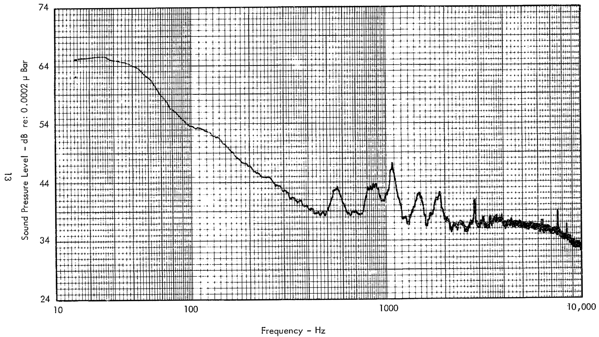
Figure 3e. Modified Fan Assembly 3 Feet to Side of Inlet (Azimuth 90^{\circ} ). Fan 4-1/2 In. Behind Inlet.
