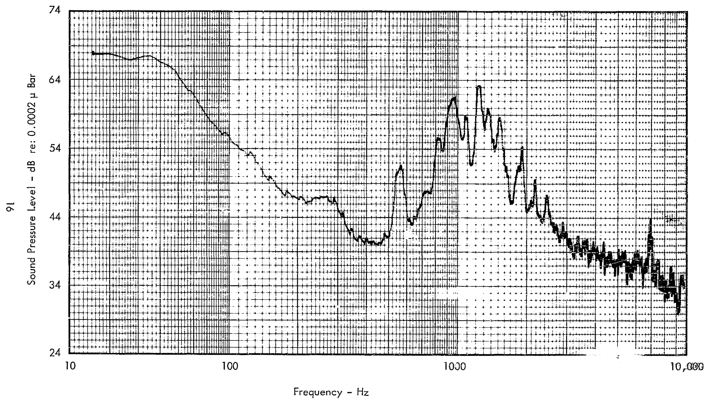
Figure 3h. Standard Fan Assembly 3 Feet to Side of Inlet (Azimuth 90^{\circ} ).
