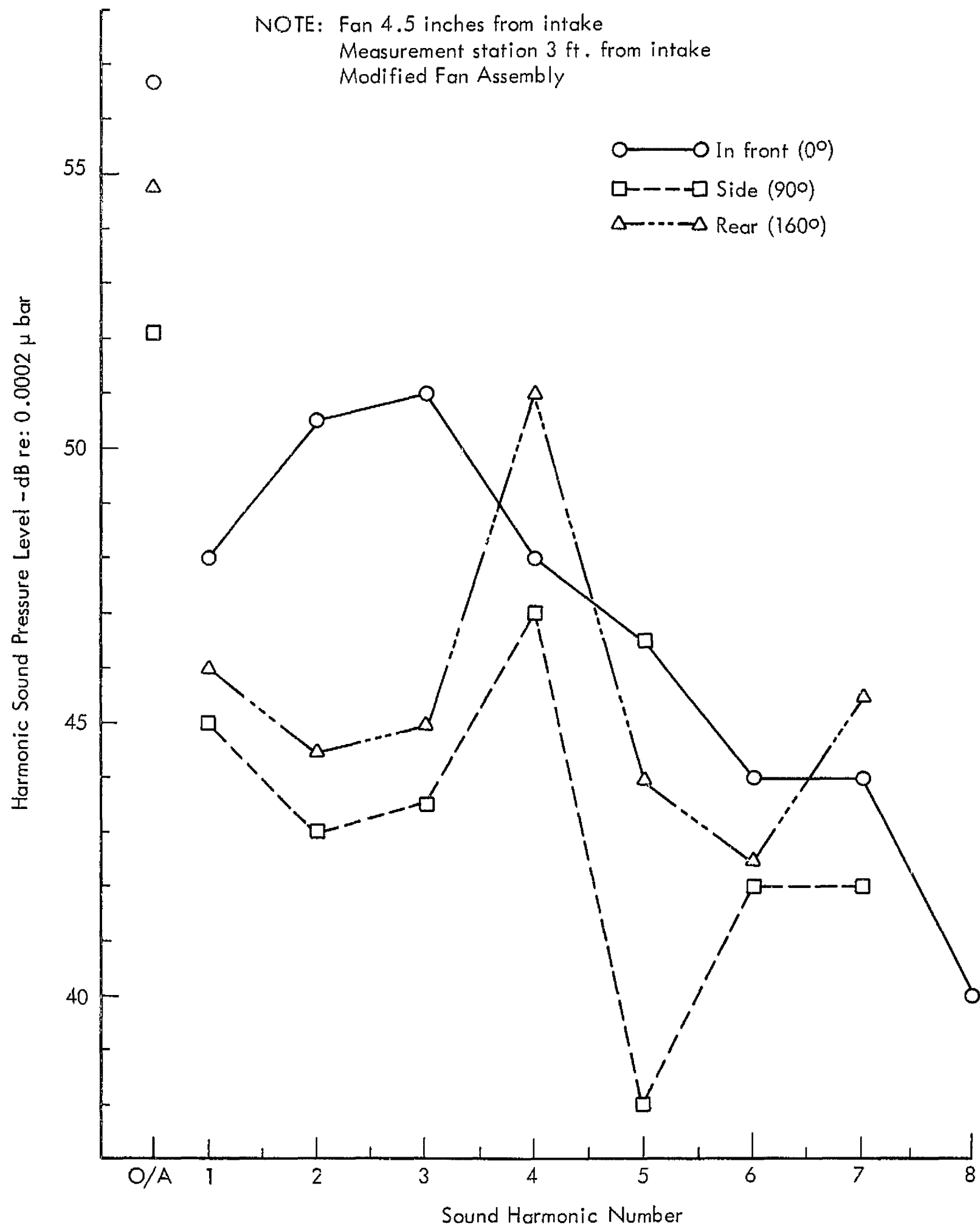
Figure 7. Effect on Harmonic Levels of Measurement Station Azimuth Location
