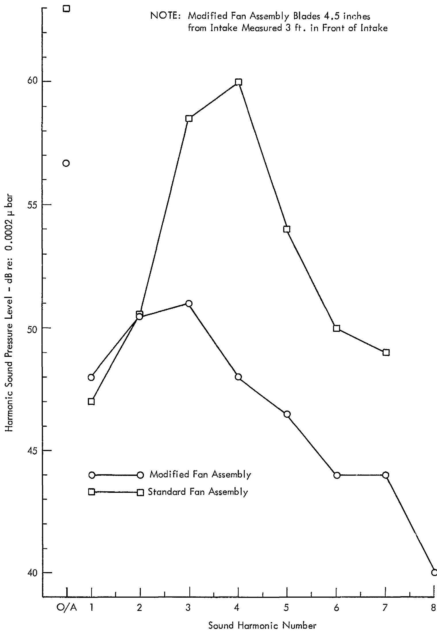
Figure 8. Comparison of Standard Fan Assembly with Modified Fan Assembly - Azimuth 0^\circ
