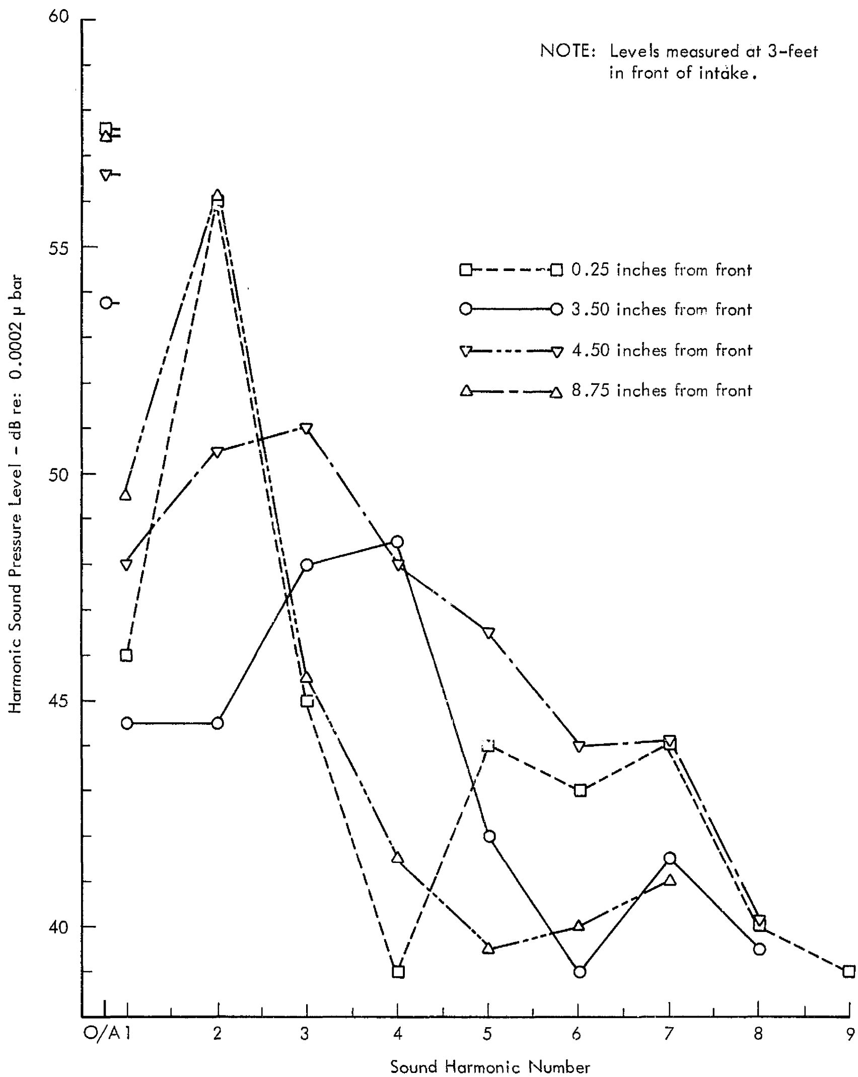
Figure 4. Effect on Harmonic Levels of Fan Position in Duct - Modified Fan Assembly
