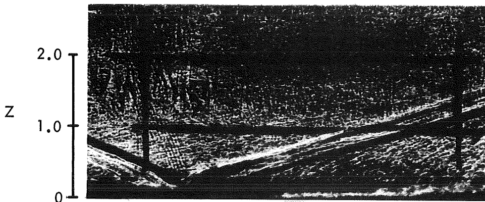
Figure 20 PLATE STATIC PRESSURE AND SHOCK WAVE PATTERN IN THE INTERACTION REGION.
