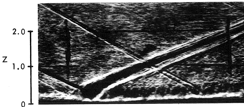
Figure 7 PLATE STATIC PRESSURE AND SHOCK WAVE PATTERN IN THE INTERACTION REGION.
