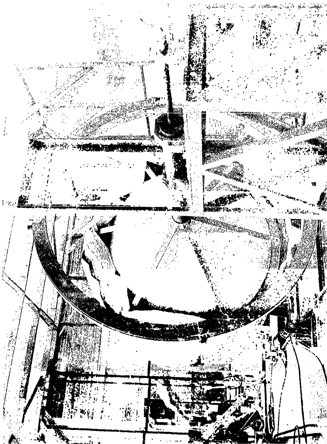
FIGURE 40 - BOTTOM END SUPPORT
