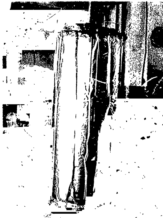
FIGURE 36B CYLINDRICAL PORTION
