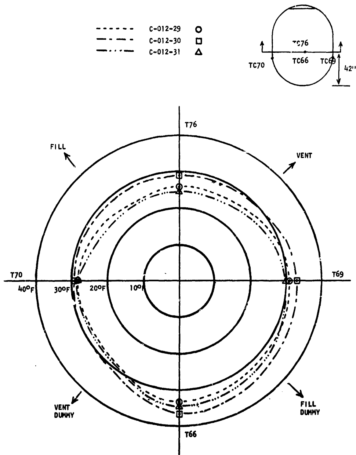
FIGURE 91 CIRCUMFERENTIAL SURFACE TEMP. PROFILE OF INSULATION BETWEEN 42 AND 40 INCH LEVEL (FROM BOTTOM)
