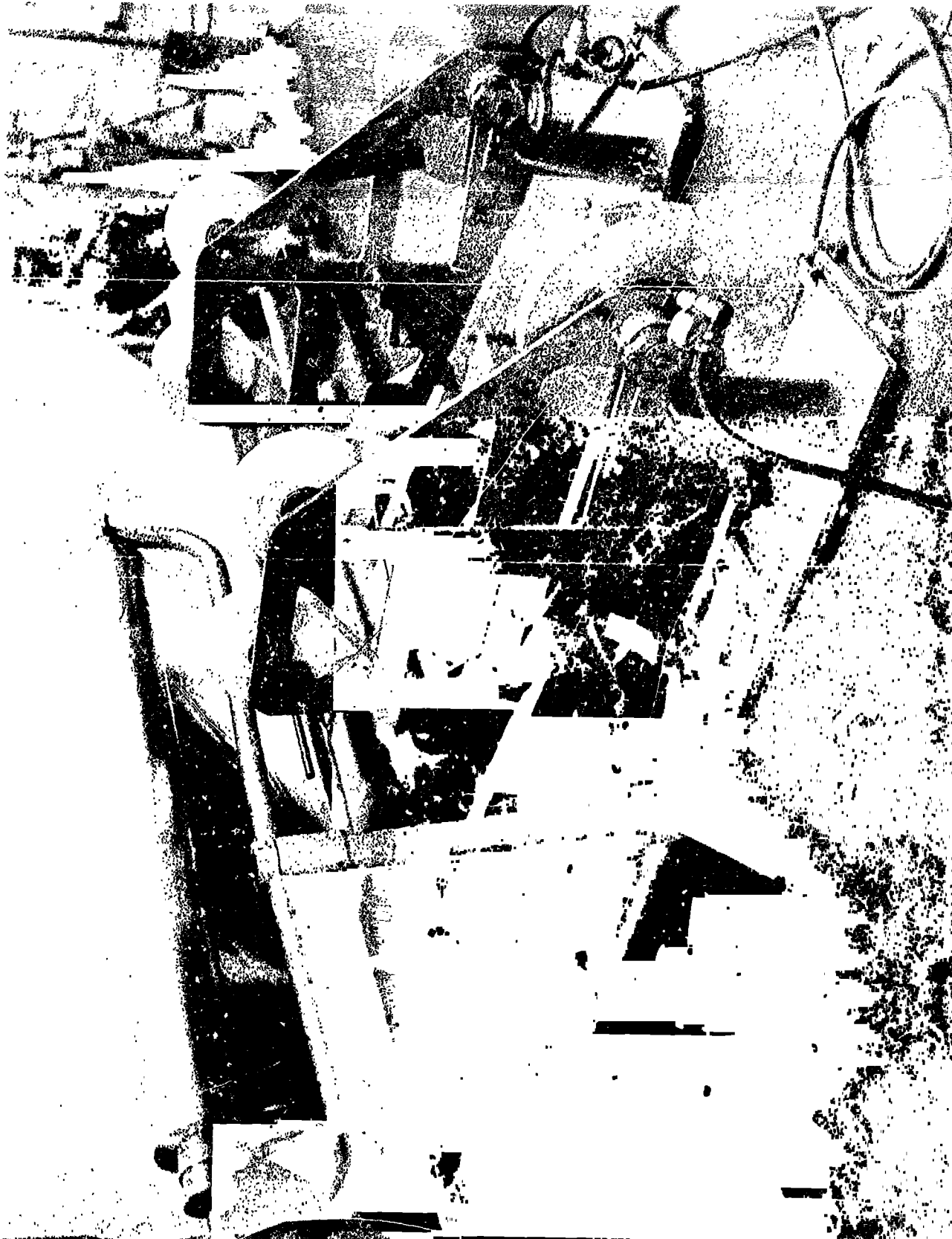
FIGURE 41 - ALUMINUM FOIL AND TENSION BAND APPARATUS
