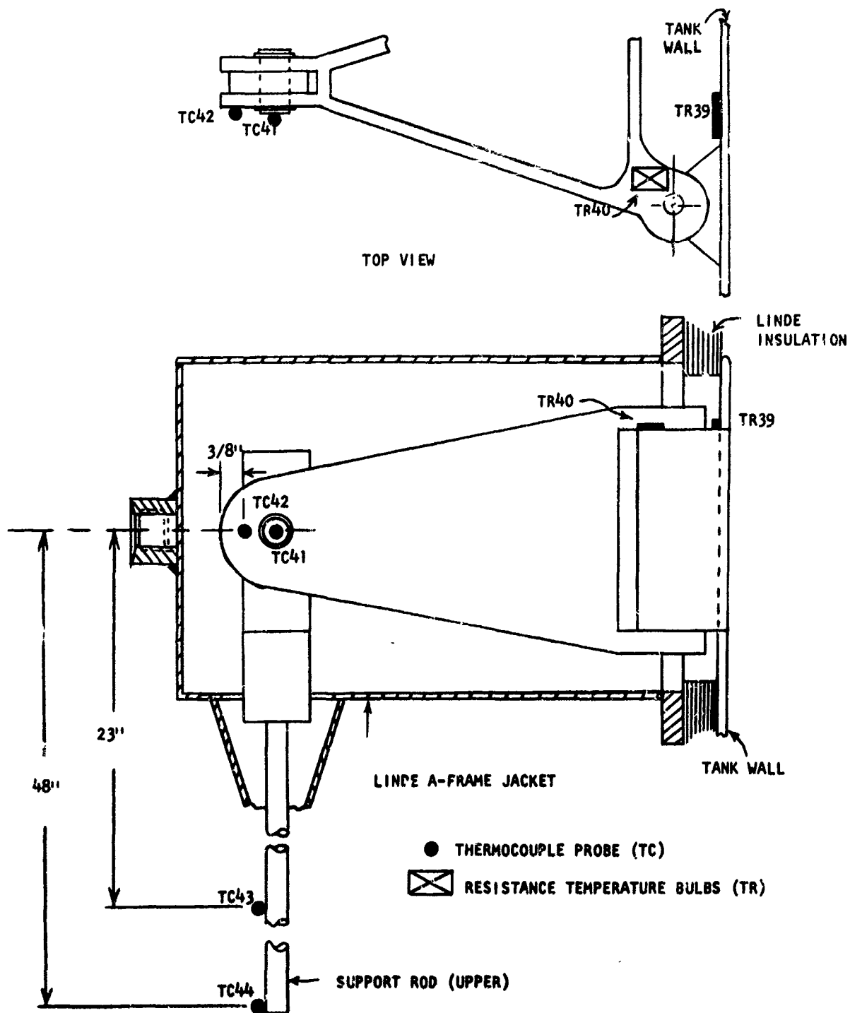
FIGURE 82 - A-FRAME INSTRUMENTATION
