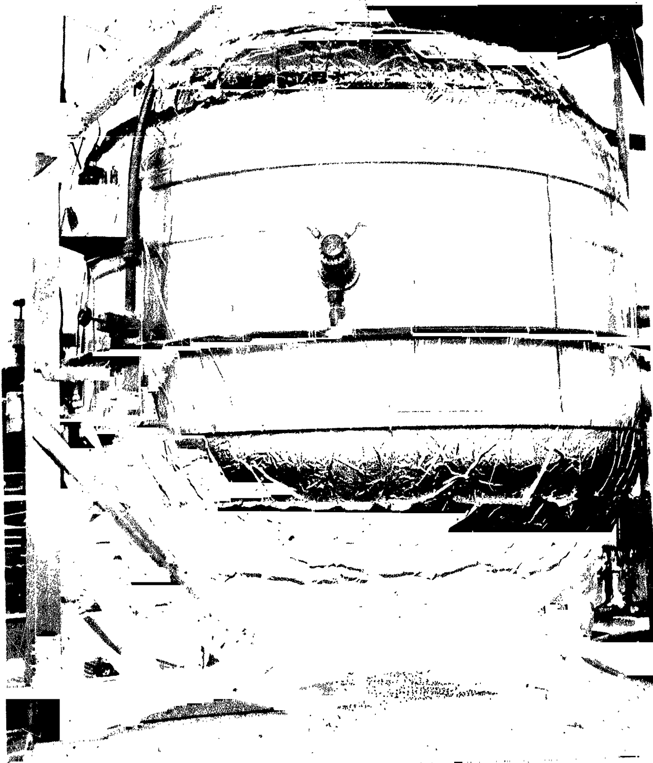
FIGURE 76 - Test Tank Ready for Admission to the Vacuum Chamber
