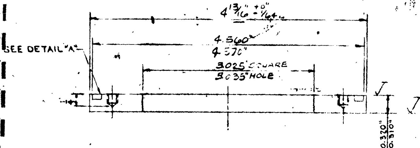
PLAN VIEW SCALE 48" = 1'-0"
