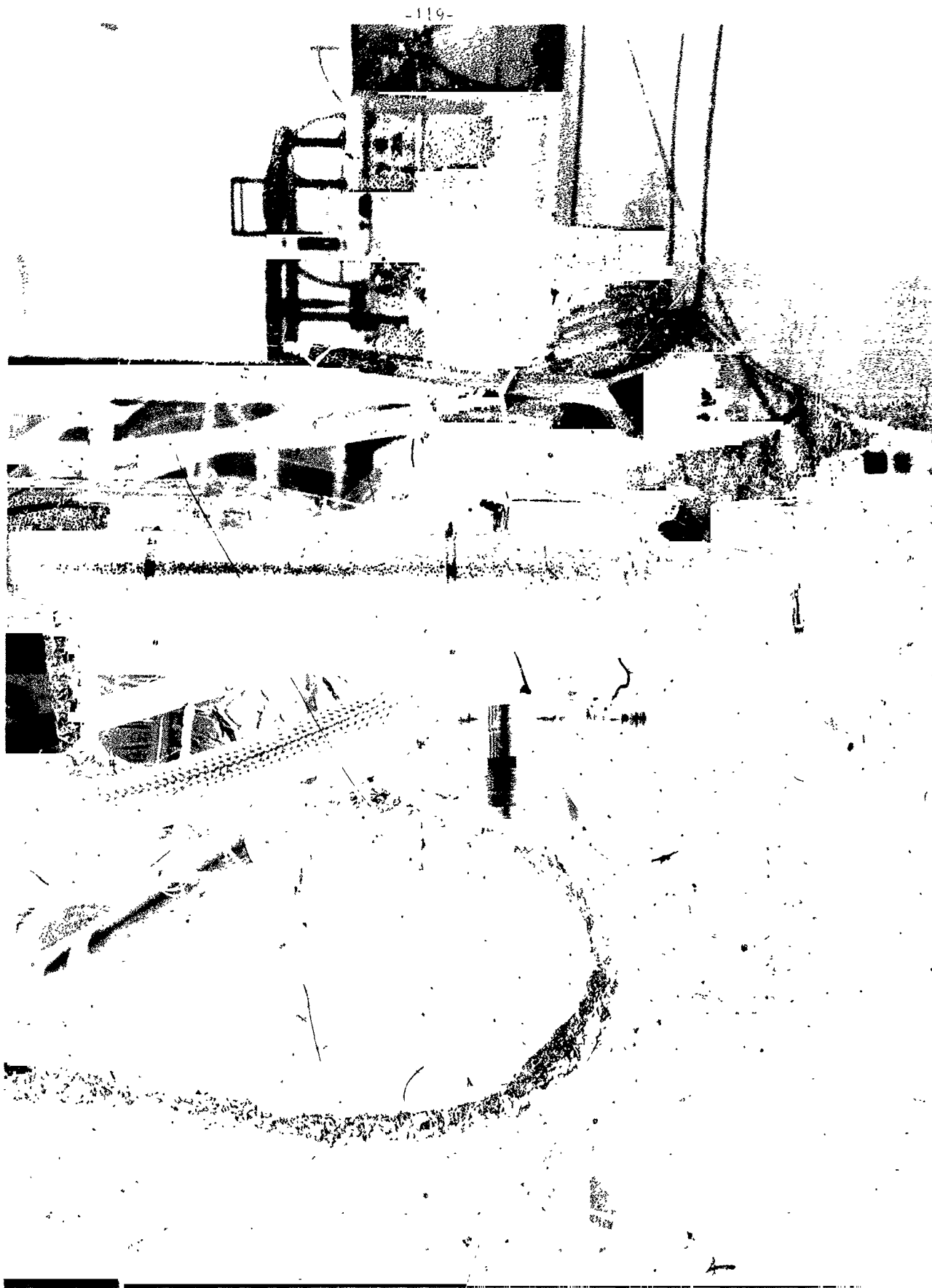
FIGURE 65 - Air Heater for Tank Purge
