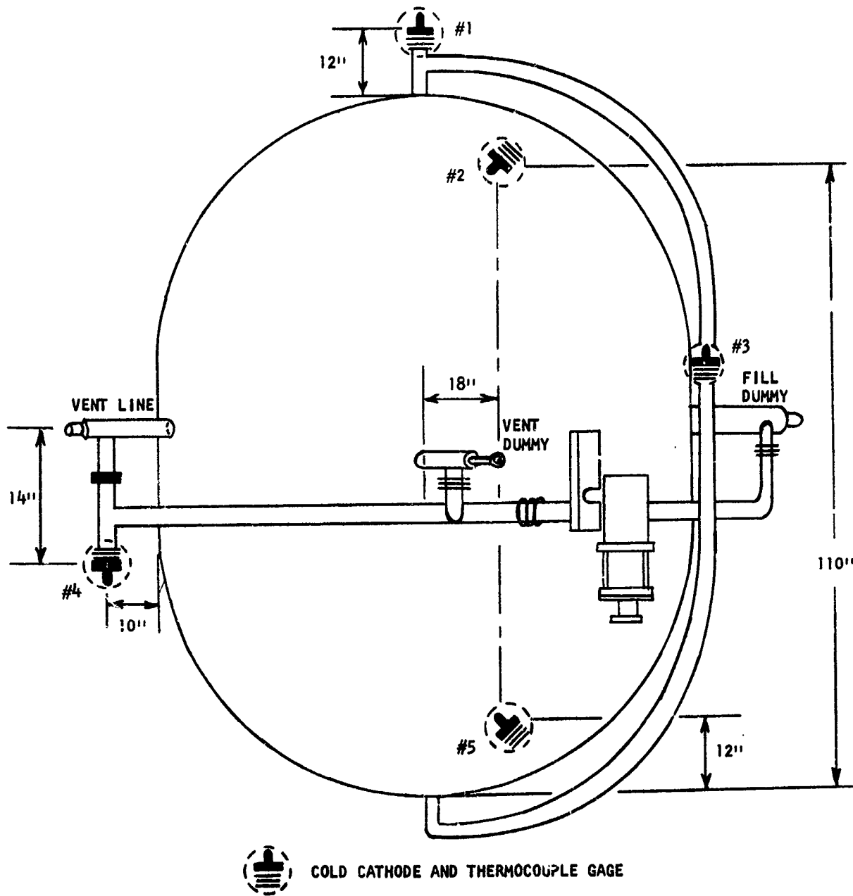
FIGURE 77 - Tank Insulation Pressure Measurements
