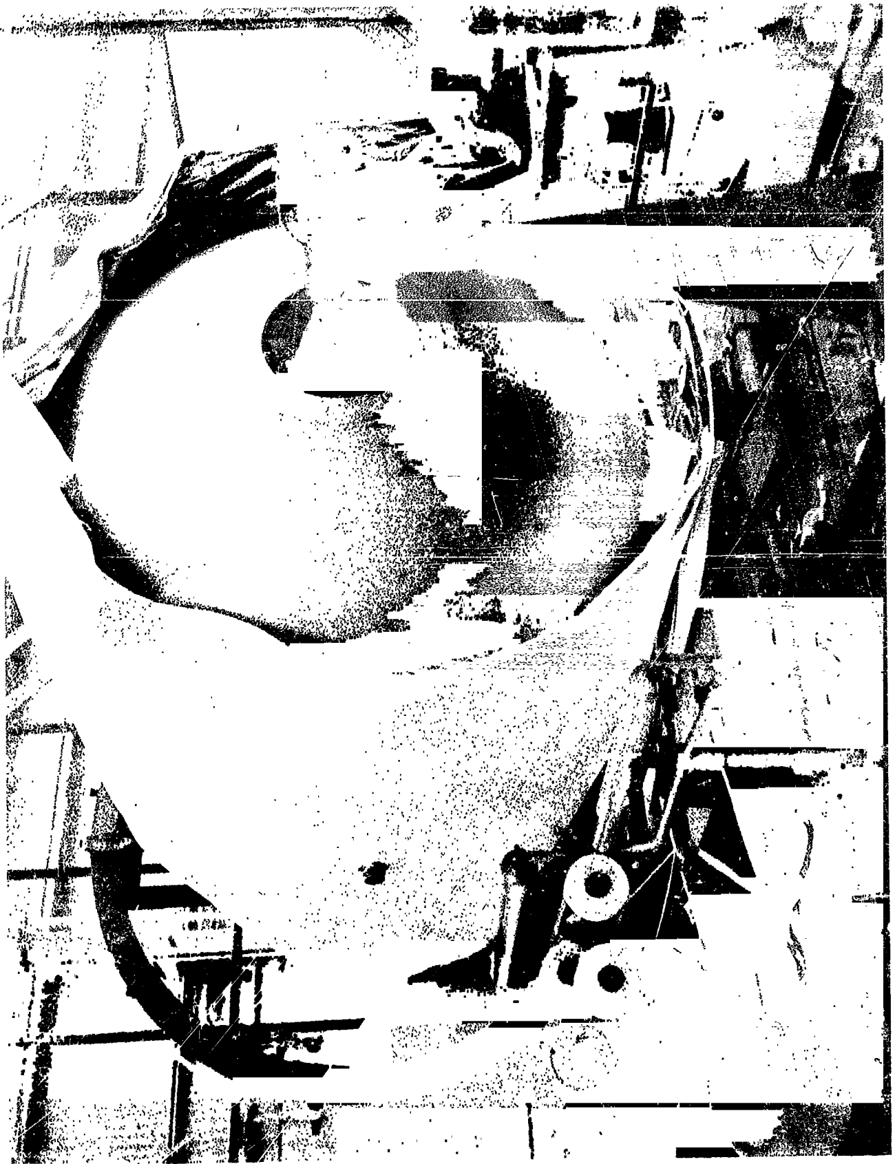
FIGURE 39 - CYLINDRICAL WRAP - TOP END
