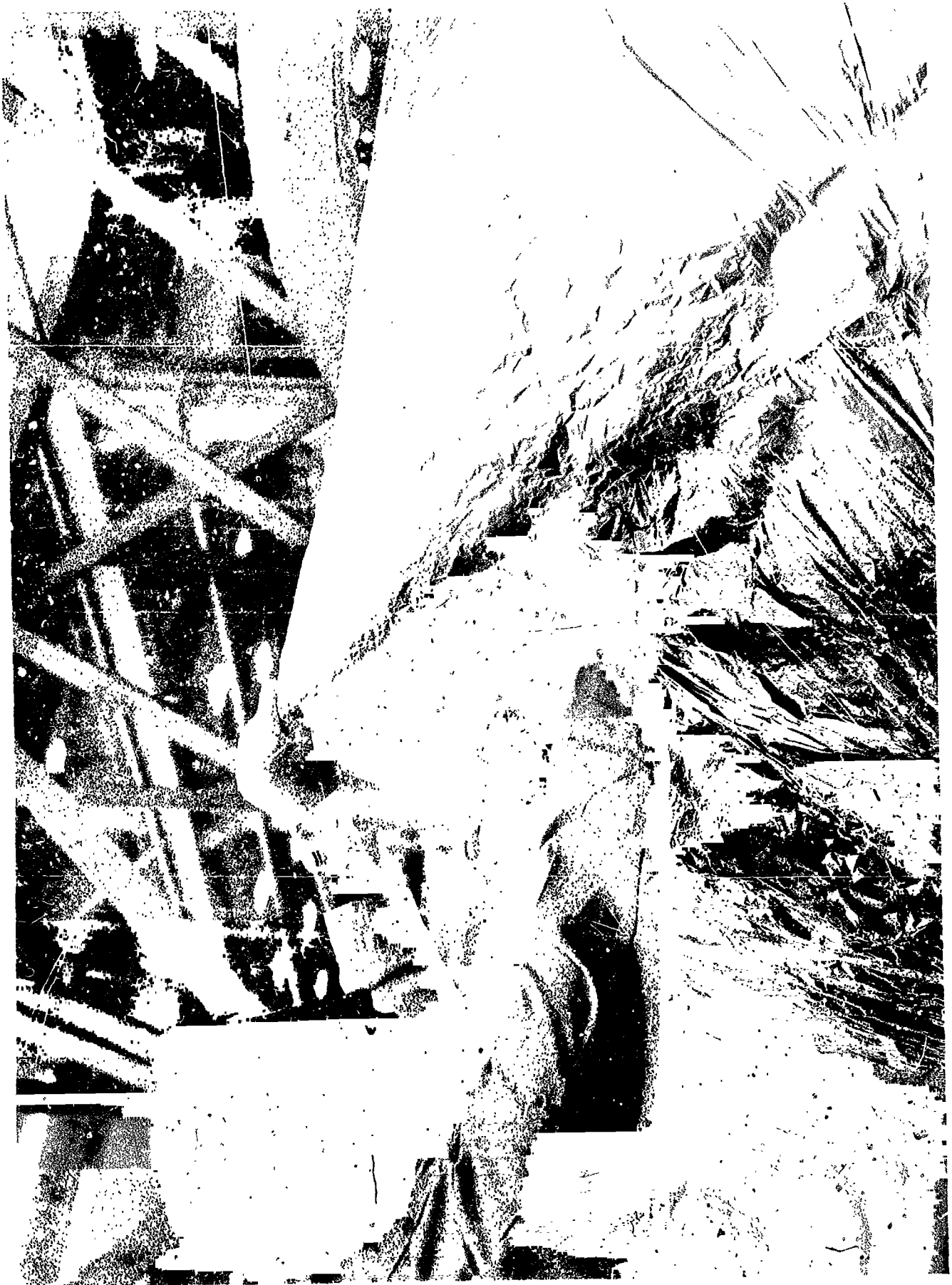
FIGURE 45 - APPLICATION OF BOTTOM BULKHEAD DISCS
