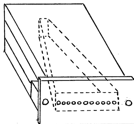
Fig. 5.2 Single-hole coupler
