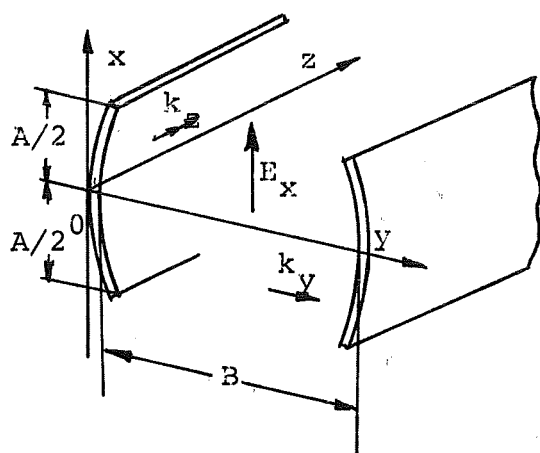
Fig. 3.1 Confocal Resonator
