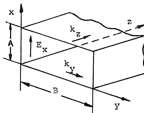
Fig. 3.2 Rectangular-cavity resonator
