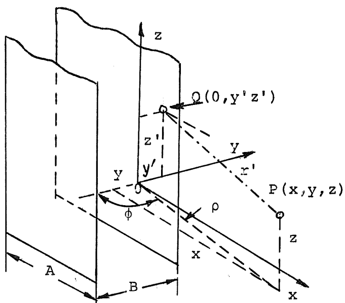
Fig. 3.3 Field intensity at observing point P
