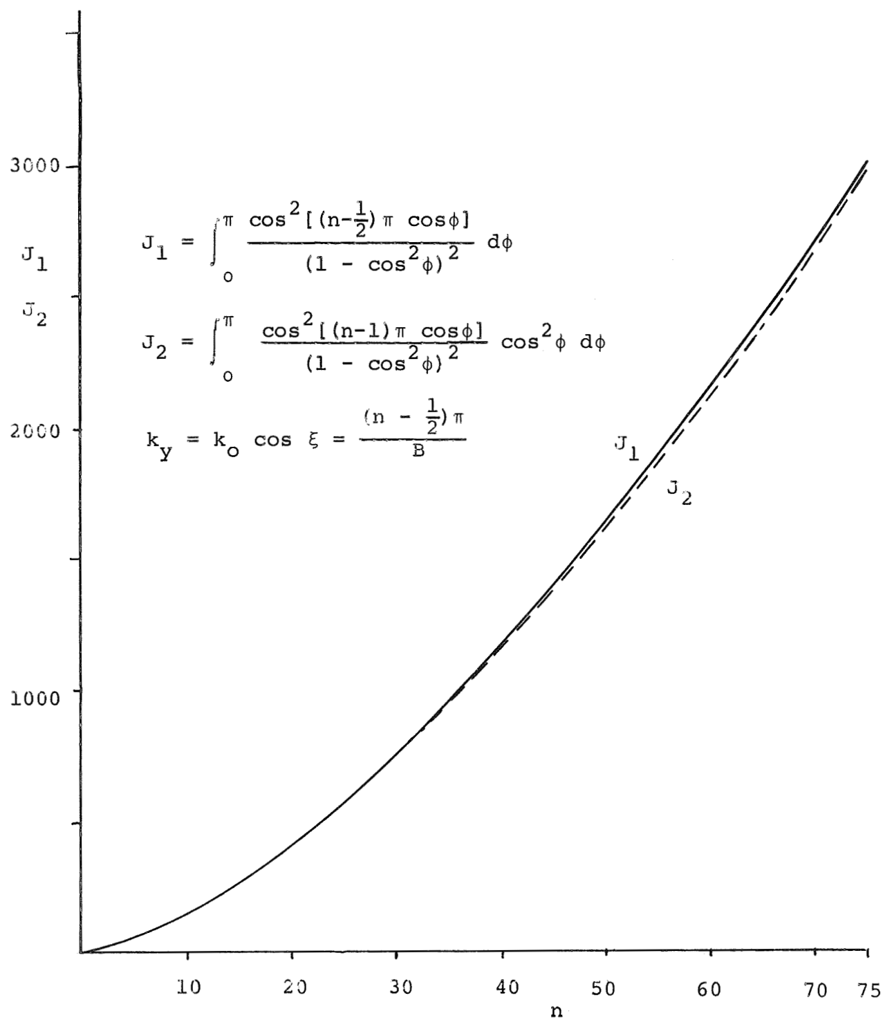
Fig. 3.7 Integrals J_1 and J_2 vs. n .
