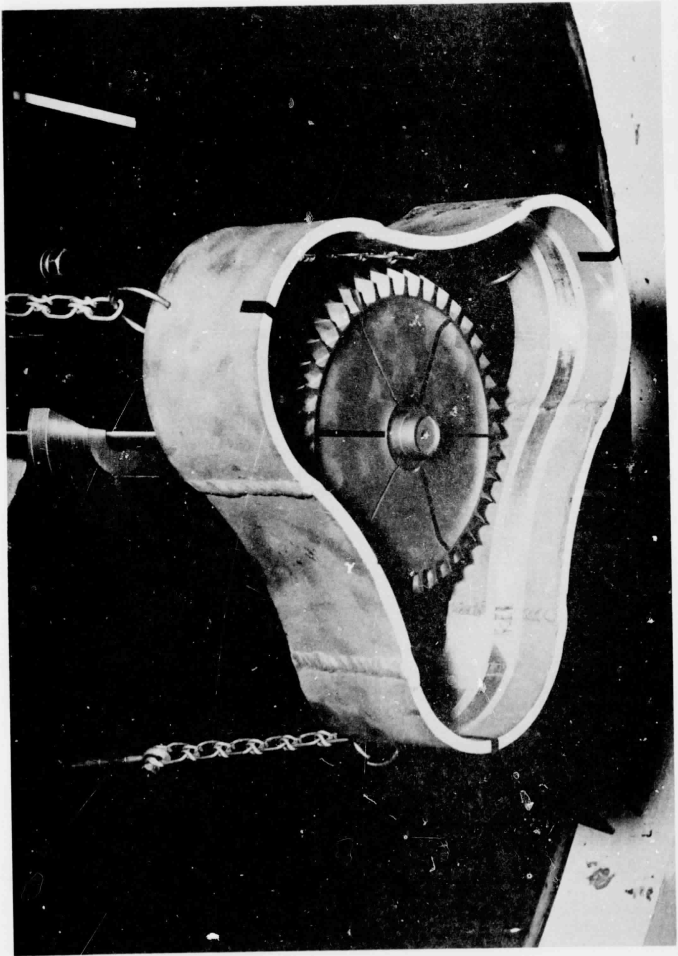
PRE-TEST 26 MOMENTUM TRANSFER FRAGMENT CONTROL DEVICE INSTALLATION
