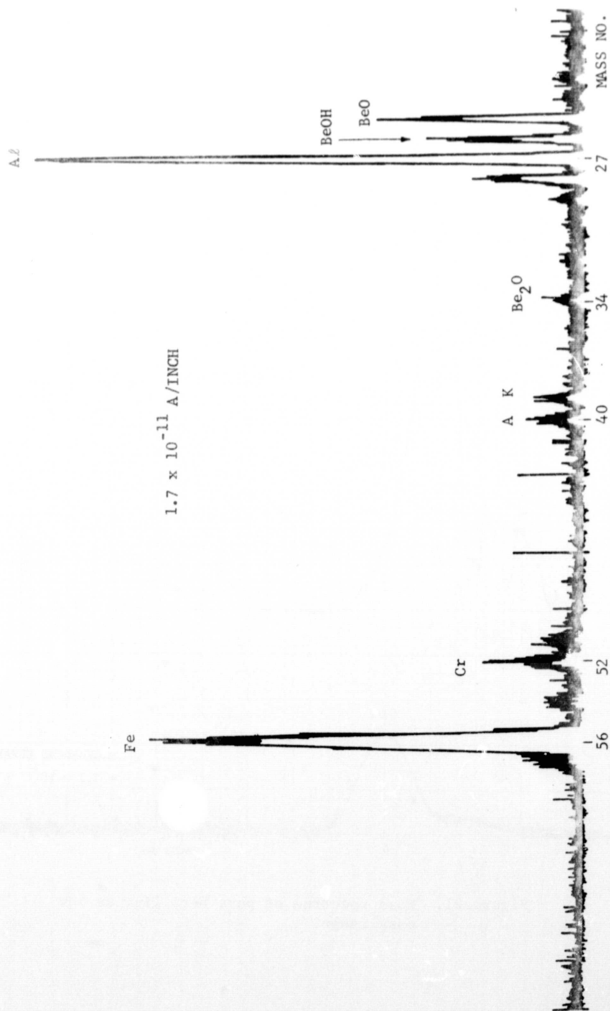
Figure 20. Mass spectrum of pure beryllium on high mass range.
