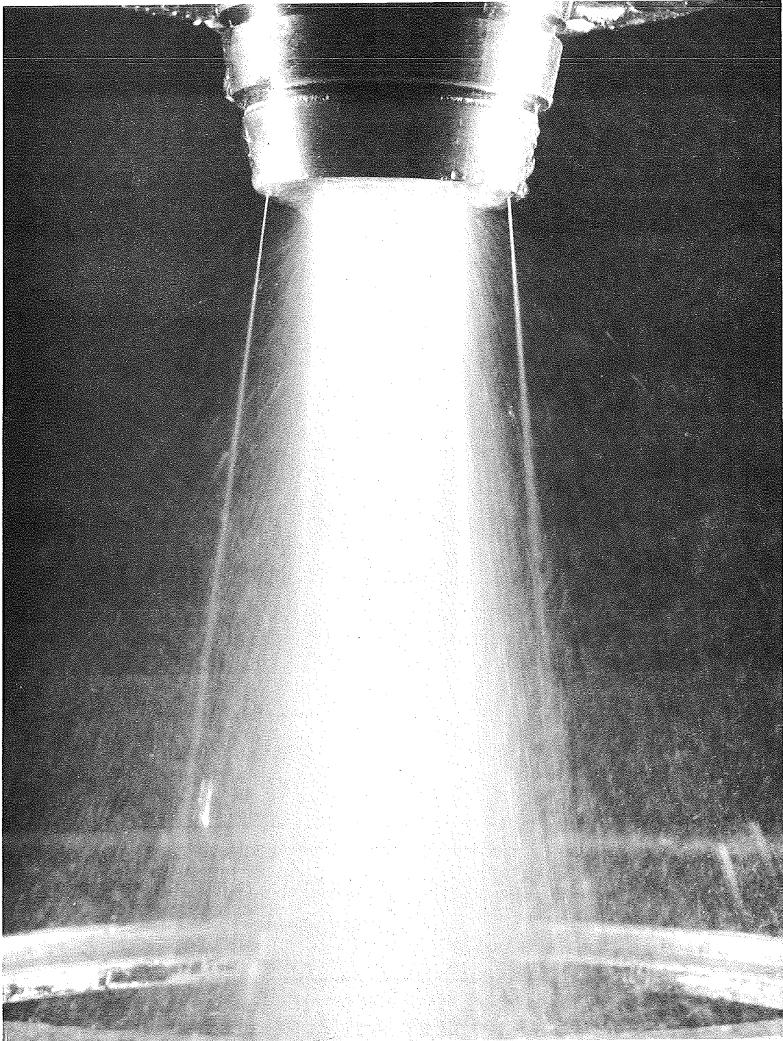
FIGURE 10. Total Spray Pattern from Water Flow Tests of the Serial No. 001 FLOX/Methane Injector
