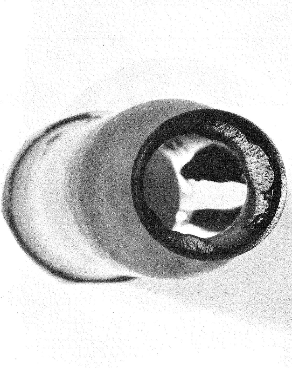
FIGURE 21. End View of Thin Wall PG Chamber Exit after Run 45
