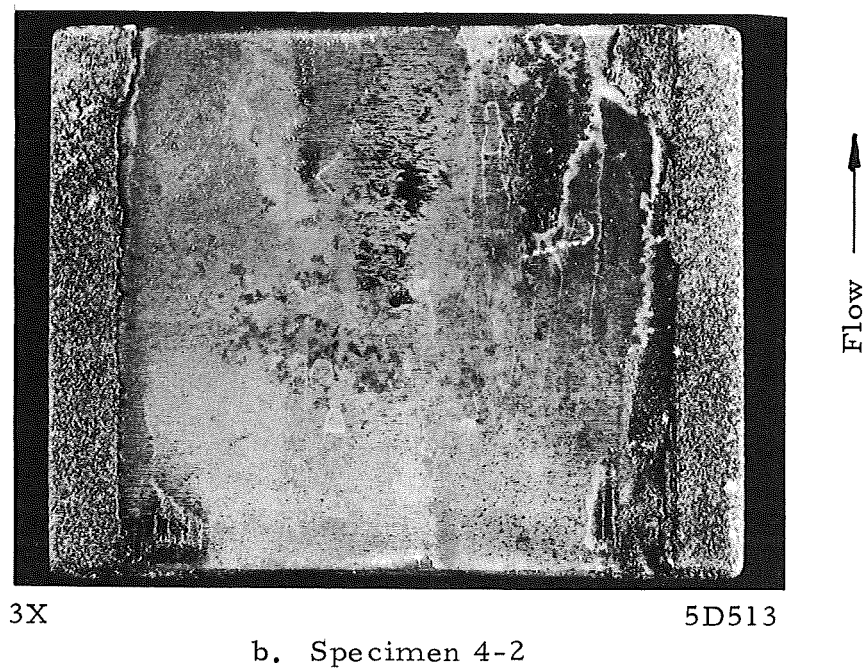
FIGURE 26. UNCOOLED, SOLID-BLOCK SPECIMENS (COATING SYSTEM 4) AFTER SHORT-TERM ROCKET-FIRING TEST
