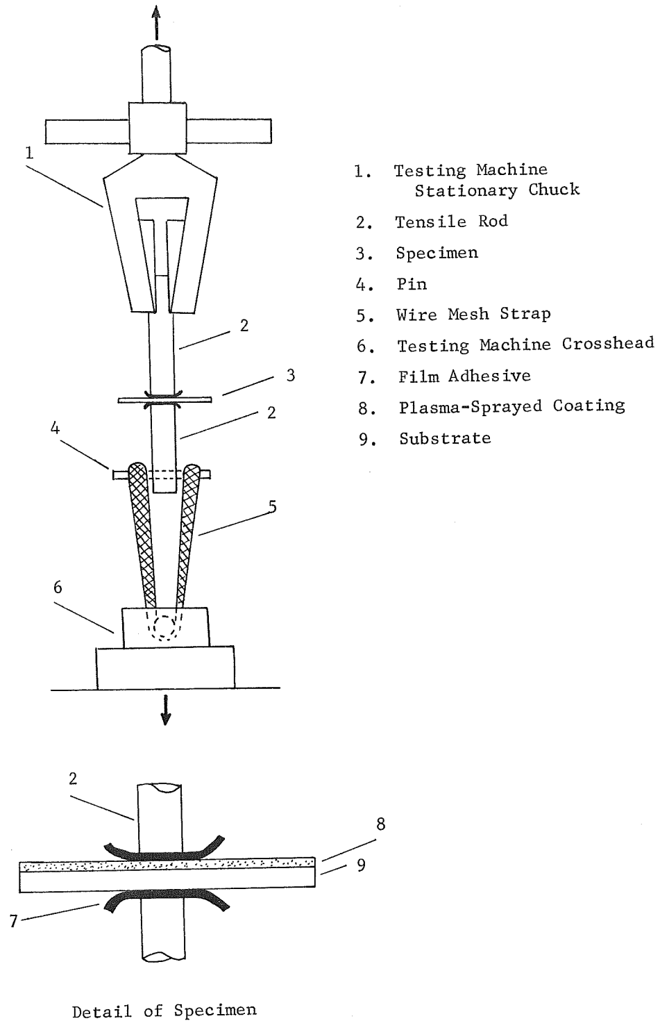
FIGURE 4. TESTING ARRANGEMENT FOR BOND STRENGTH MEASUREMENTS
