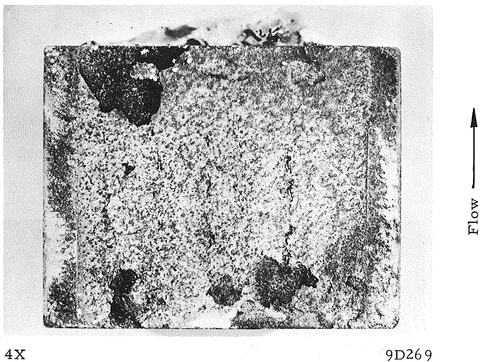
FIGURE 32. SURFACE OF SPECIMEN TC=7 AFTER 1-SECOND ROCKET FIRING
