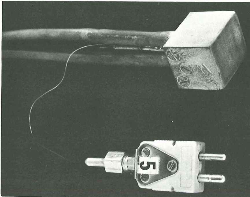
FIGURE 14. WATER-COOLED ROCKET-TEST SPECIMEN
