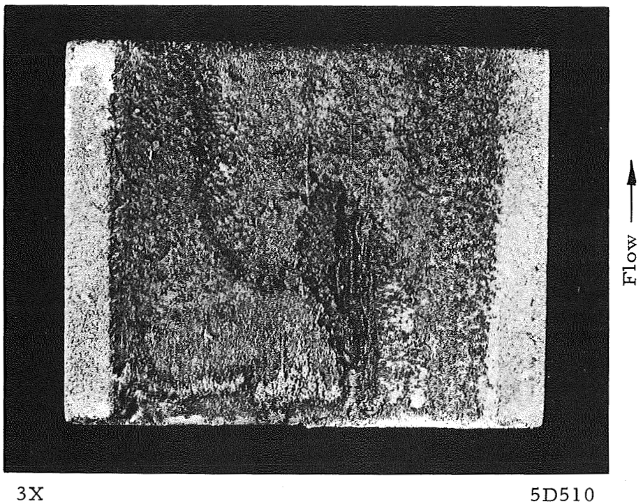
b. Specimen 2-2
