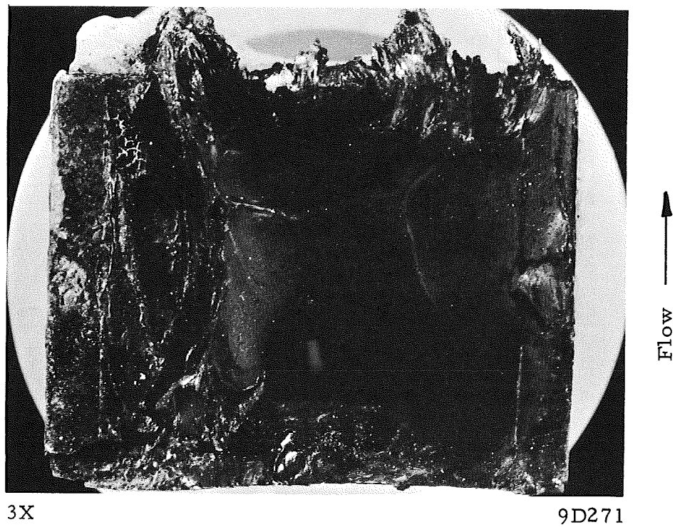
FIGURE 29. WATER-COOLED SPECIMEN DESTROYED BY ROCKET-MOTOR FAILURE
