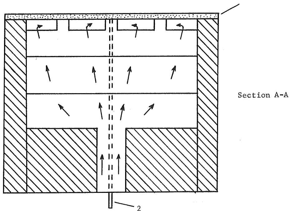
FIGURE 13. BASIC DESIGN OF COOLED SPECIMENS
