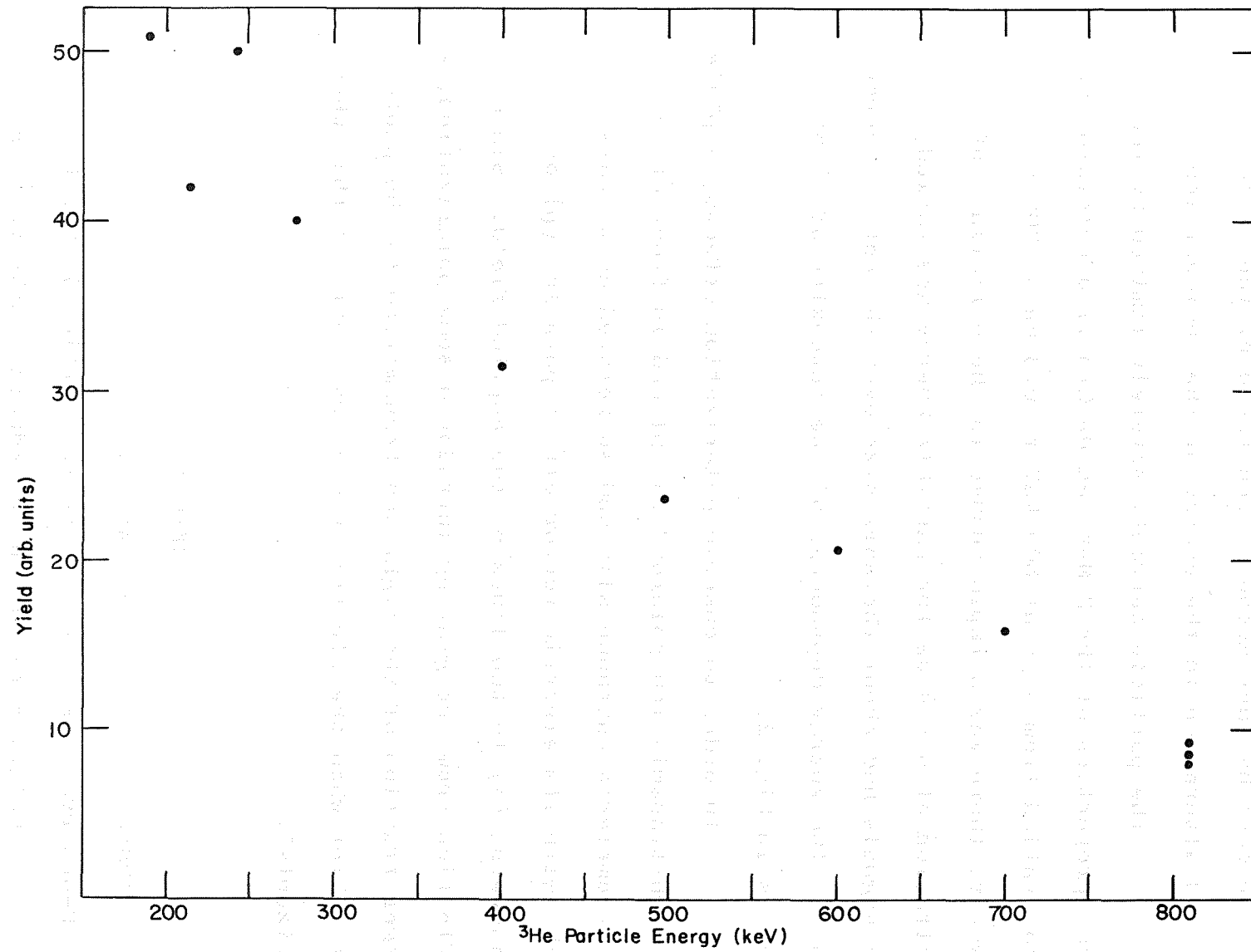
Fig. 2: Yield of \lambda 4686 \text{ \AA} as a function of ^3\text{He} energy.
