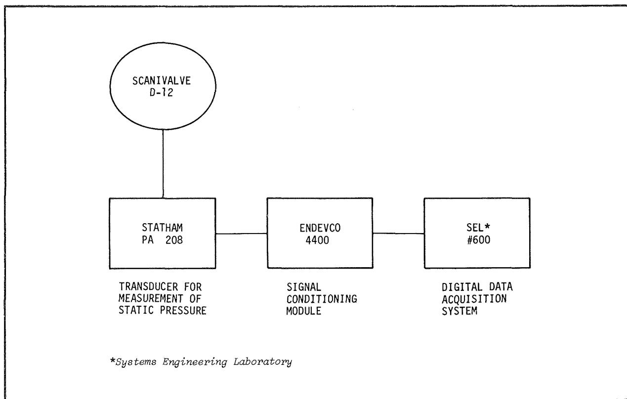
Figure 2-7. STATIC AND TOTAL PRESSURE DATA ACQUISITION SCHEMATIC
