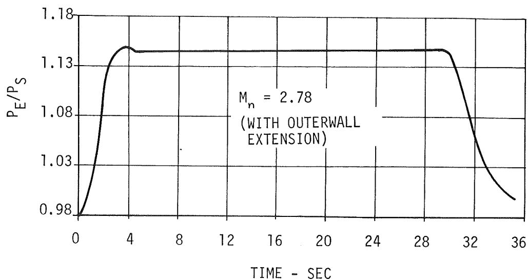
Figure 2-17. VARIATION OF P_E/P_S WITH TIME FOR BOUNDARY LAYER MODEL
