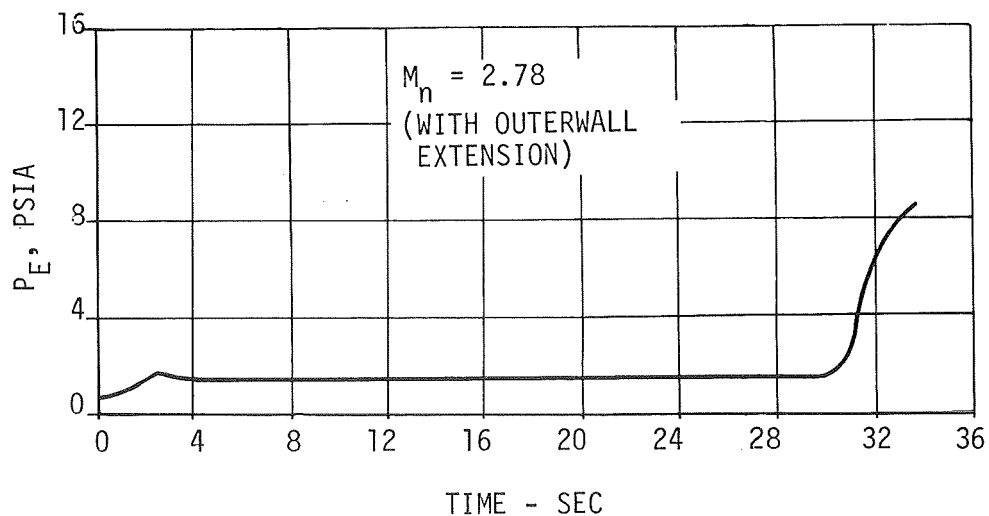
Figure 2-15. VARIATION OF P_E WITH TIME FOR BOUNDARY LAYER MODEL
