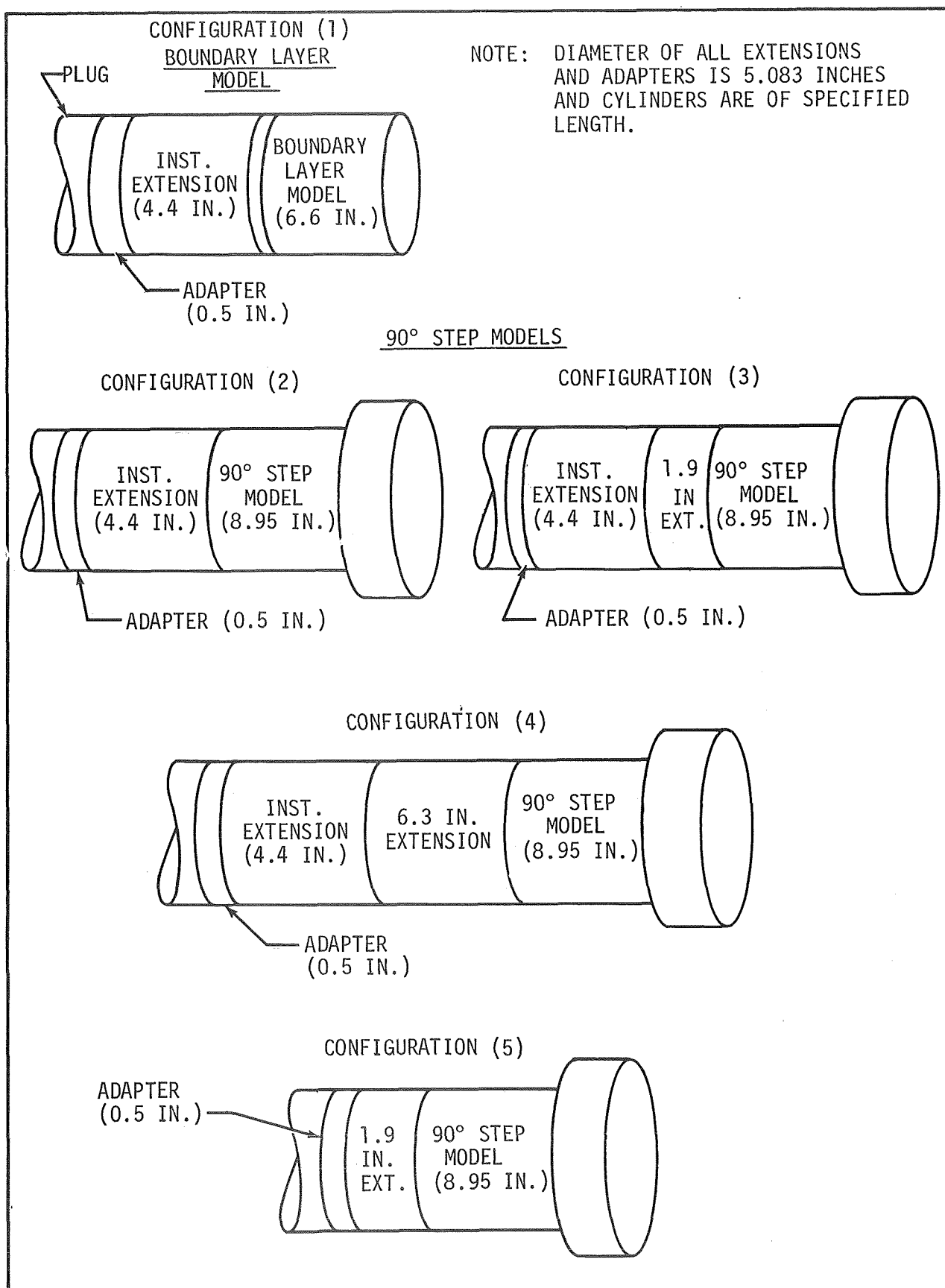
Figure 2-4. MODEL CONFIGURATIONS USED DURING THE TESTS
