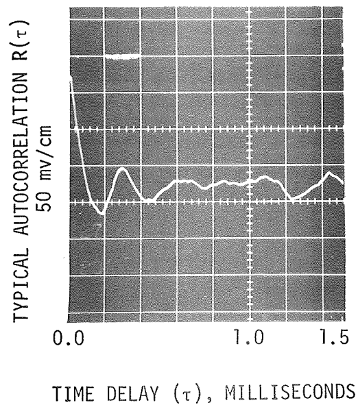
Figure 3-16. TYPICAL AUTOCORRELATION OF E_y , THE VERTICAL TUNNEL WALL ACCELEROMETER, f \approx 1600 CPS
