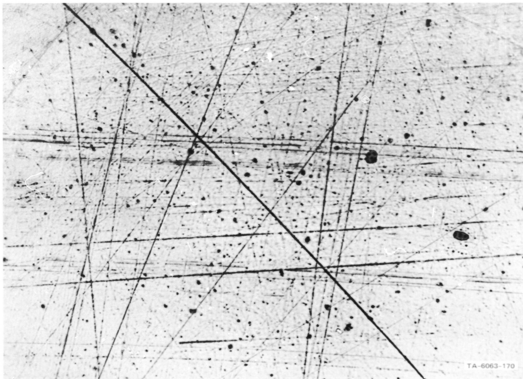
FIGURE 27 FRICTION TRACK ON SPECIMEN 23 (Group III). Rider speed 0.002 in./min. X150
