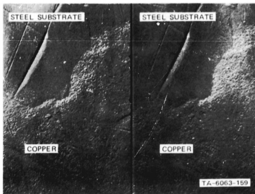
FIGURE 14 STEREO ELECTRON MICROGRAPH OF TAPER SECTION, SPECIMEN 36 (Group IV) X2000
