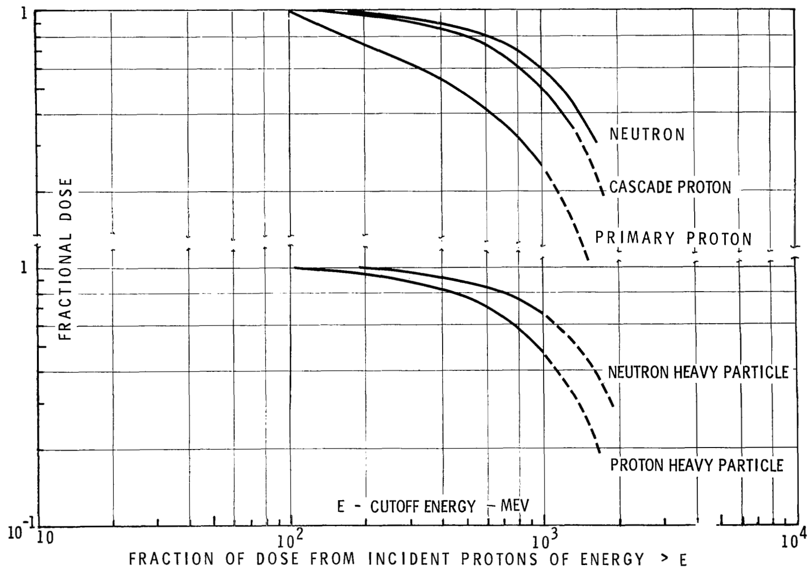
FIGURE 20: GALACTIC PROTONS INCIDENT ON 10 GM/CM 2 OF ALUMINUM
