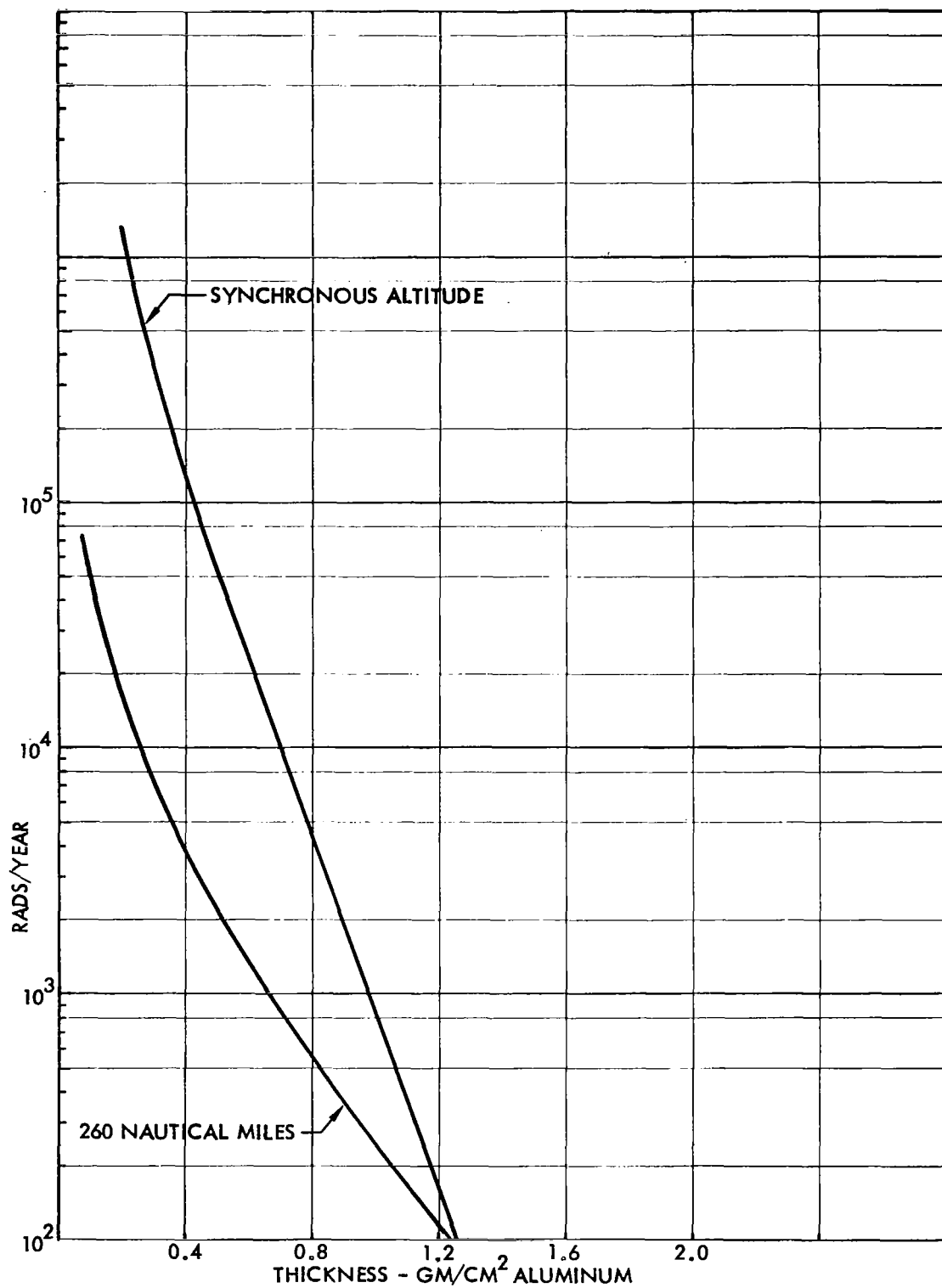
FIGURE 13 YEARLY DOSES FROM PENETRATING ELECTRONS AT SYNCHRONOUS AND 260 NAUTICAL MILES 50° INCLINATION ORBIT
