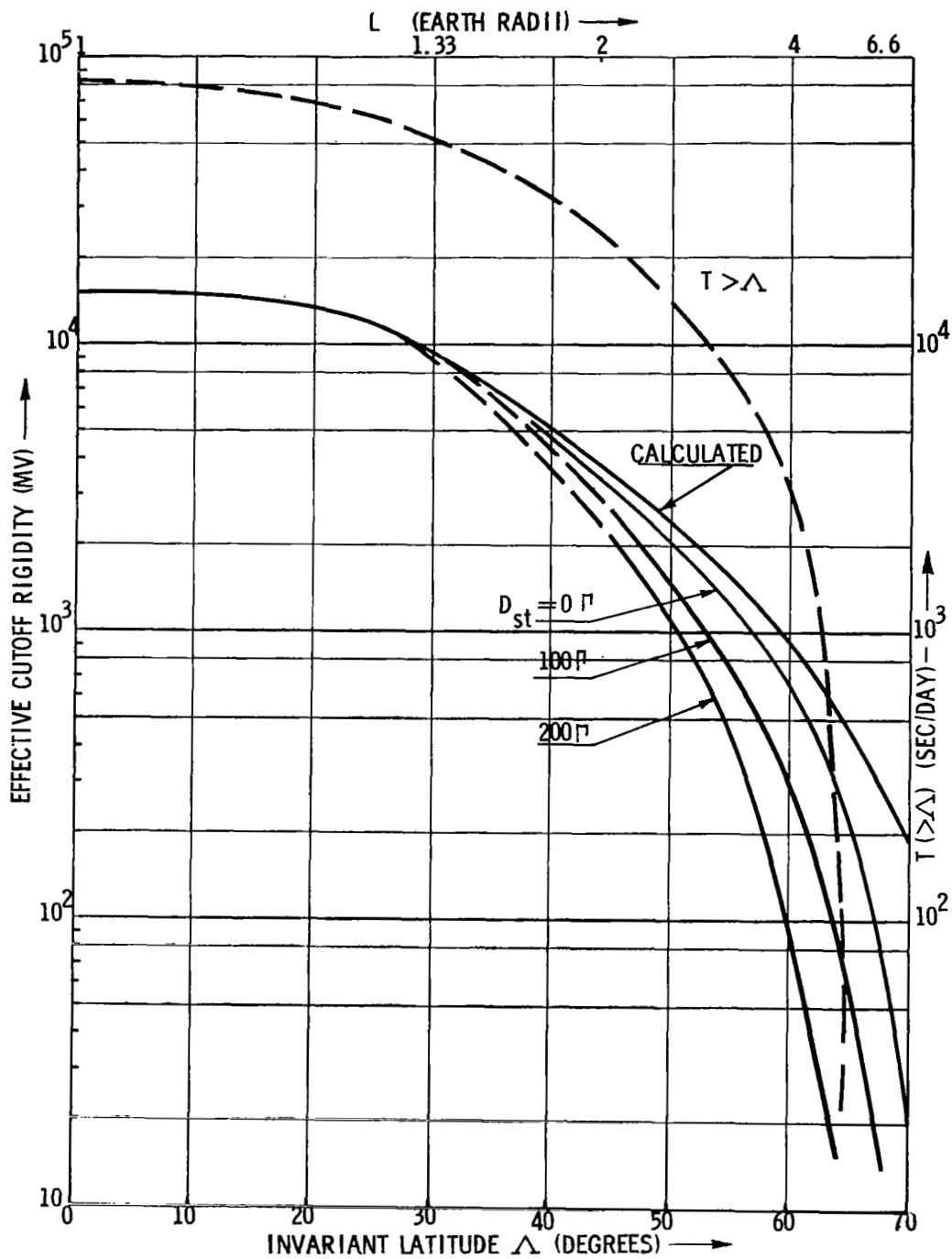
FIGURE 9 EFFECTIVE CUTOFF RIGIDITIES AND INTEGRAL TIME OF ENCOUNTER FOR A LOW ALTITUDE 50° INCLINATION ORBIT • 260 N. M. ALTITUDE
