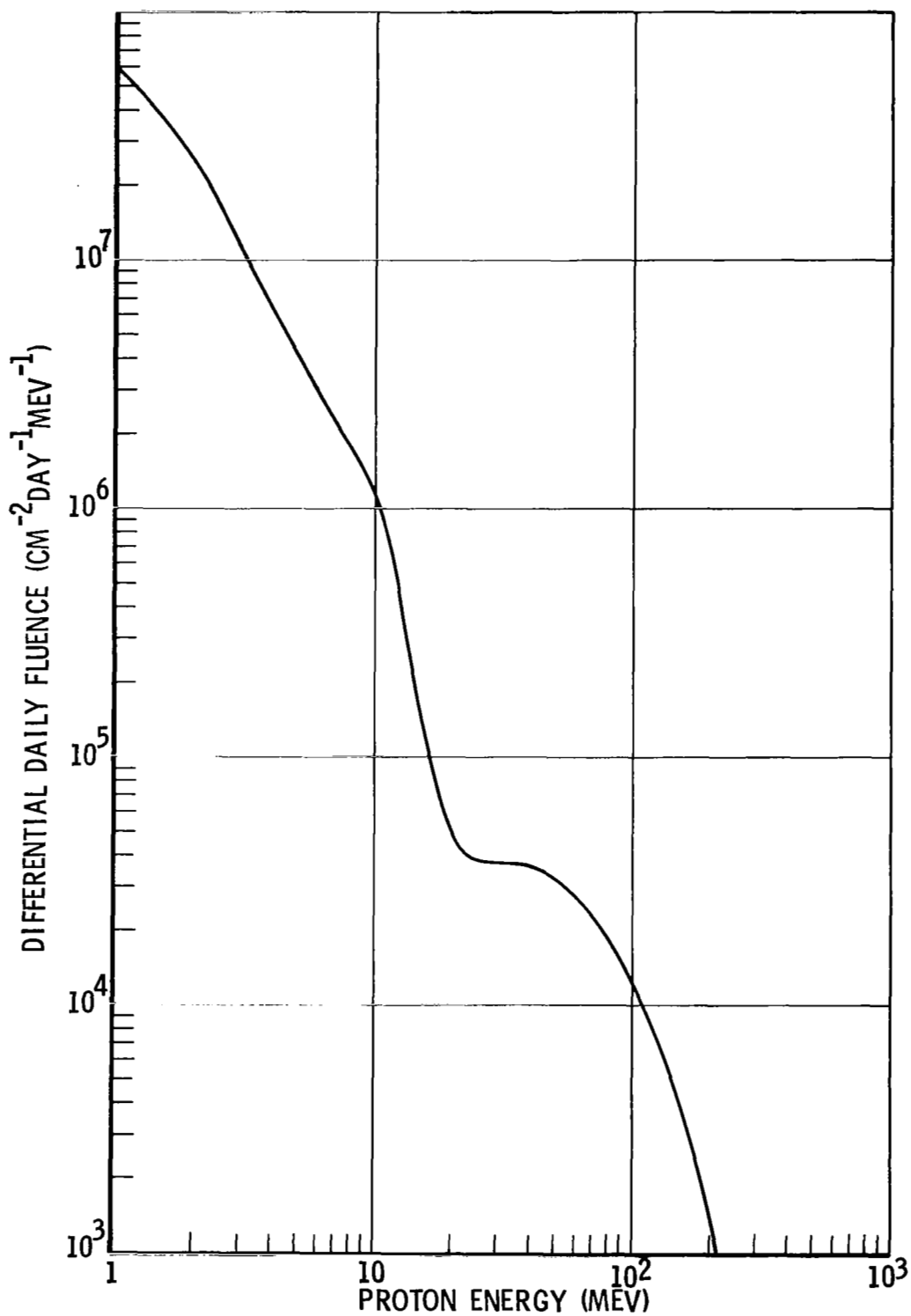
FIGURE 7: DAILY FLUENCE SPECTRUM OF TRAPPED PROTONS IN LOW ALTITUDE ORBIT, 260 N.M. ALTITUDE, 50° INCLINATION
