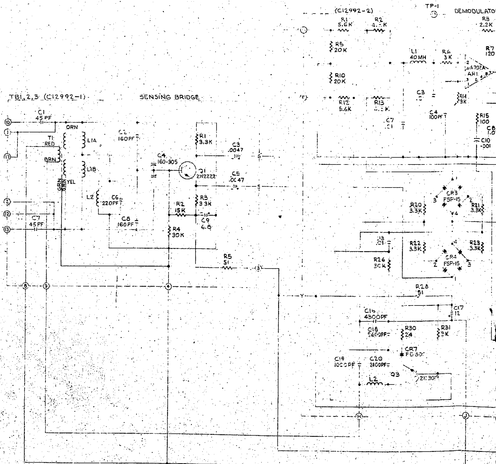
Figure 13. Schematic Diagram of Suspension System
