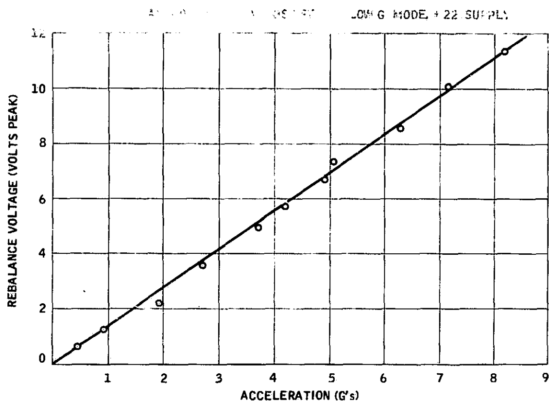
Figure 54. Results of Centrifuge Test No. 1
