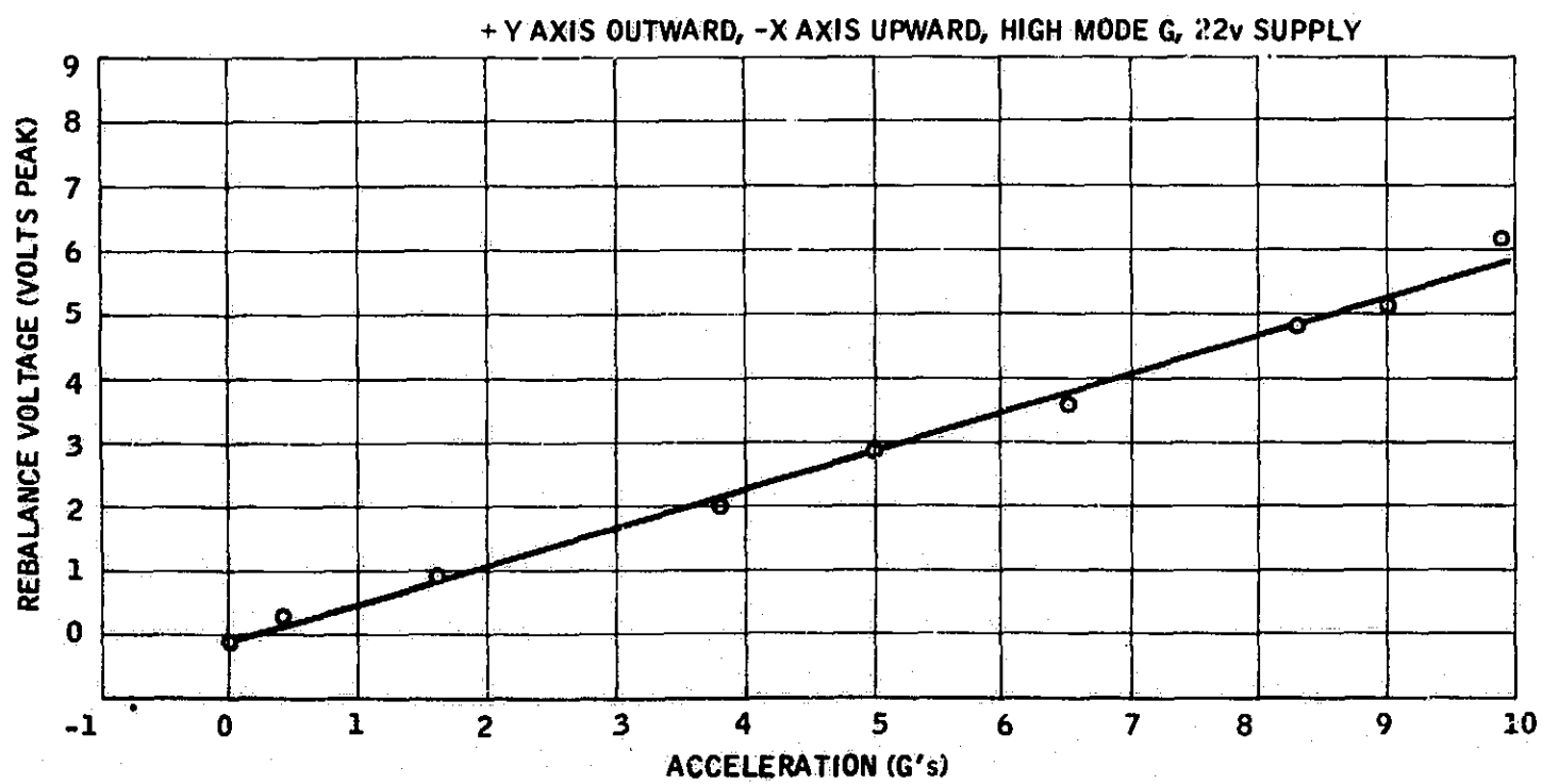
Figure 55. Results of Centrifuge Test No. 2
