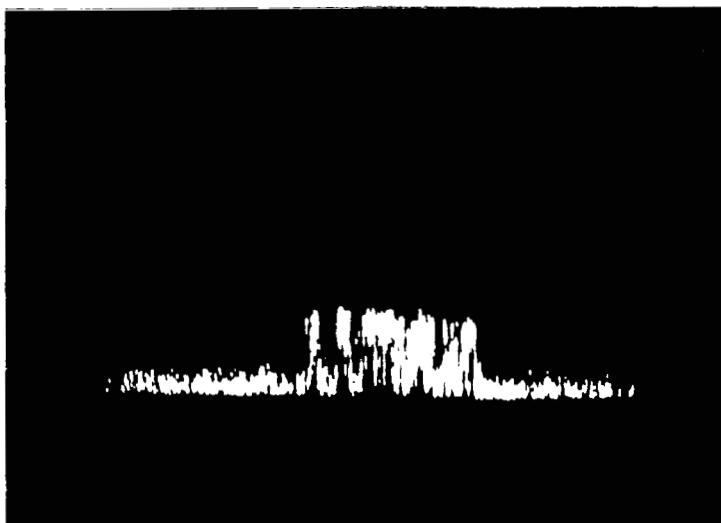
Figure 4. Frequency Domain Representation of Beat Between Two Lasers from HP Spectrum Analyzer 851B/8551B Bandwidth 30 kHz, Scan Width 50 kHz/cm, Sweep Time 10 ns
