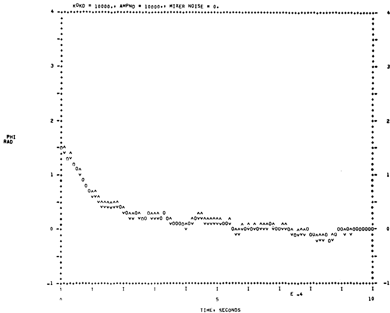
Figure A-6. Loop Gain = 10^4 ; RMS Noise = 10^4
