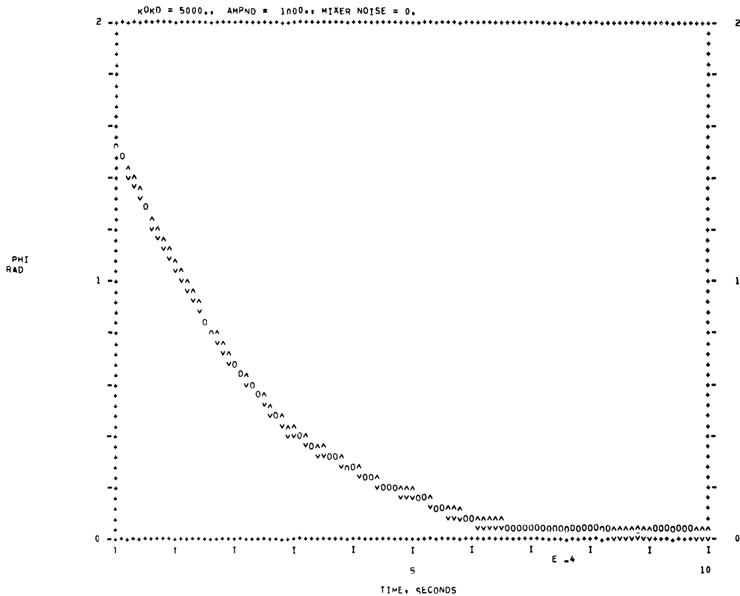
Figure A-8. Loop Gain = 5 \times 10^3 ; RMS Noise = 10^3
