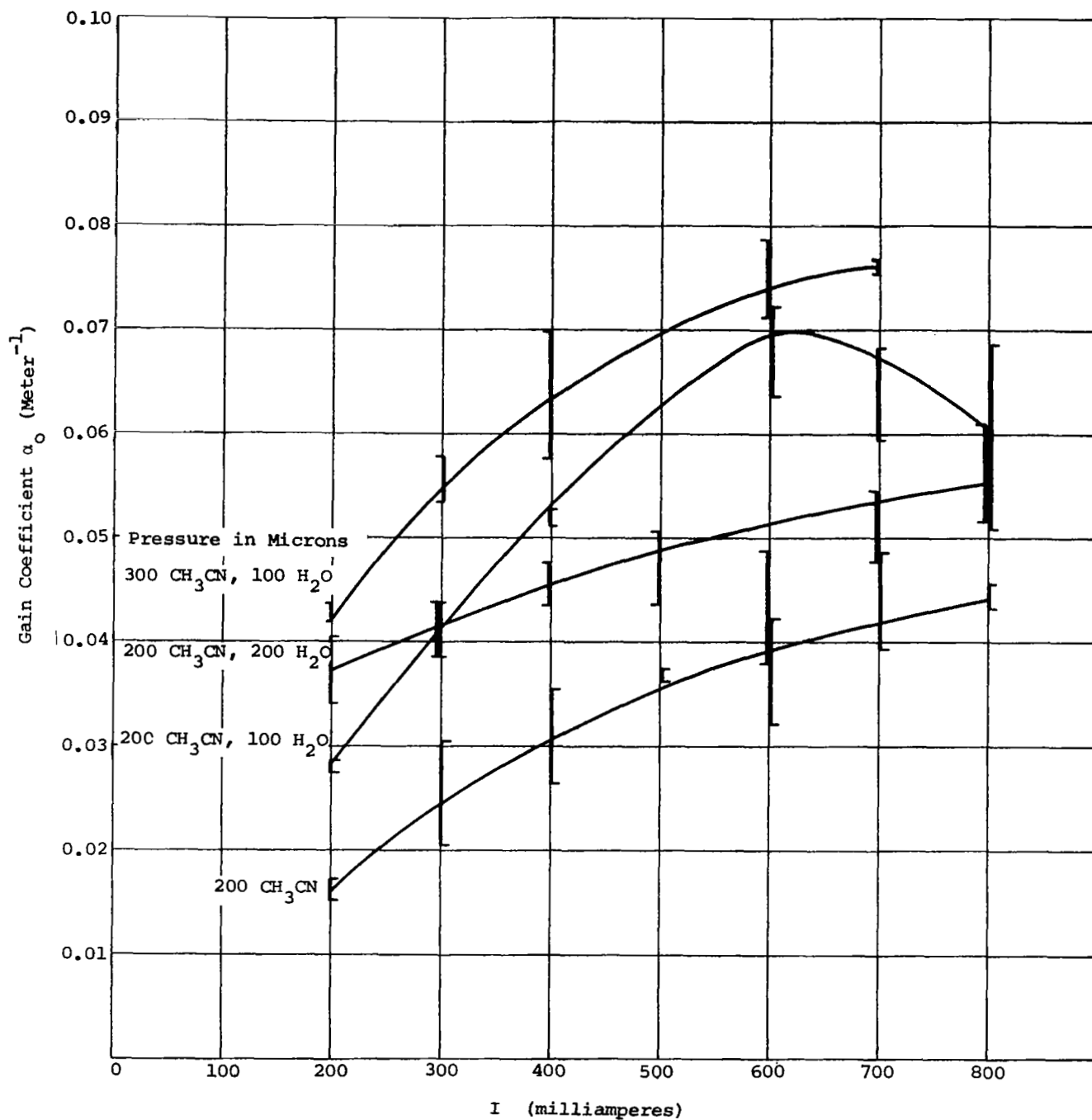
Figure B-2. Curves of Gain per Meter versus Discharge Current for Various Mixtures of \text{CH}_3\text{CN} and \text{H}_2\text{O}
