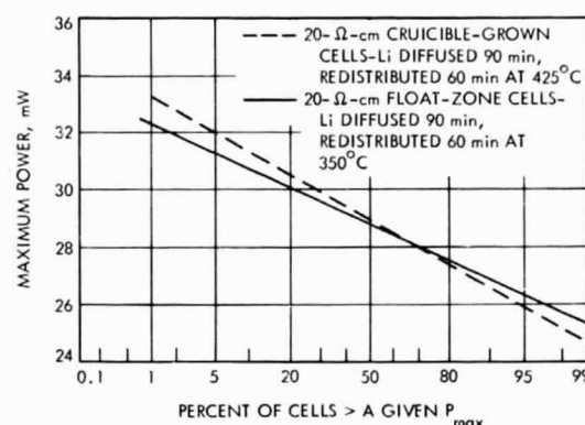
Fig. 7. Comparison of maximum power distributions of lots 9 and 10 at diffusion temperatures of 350 and 450°C
