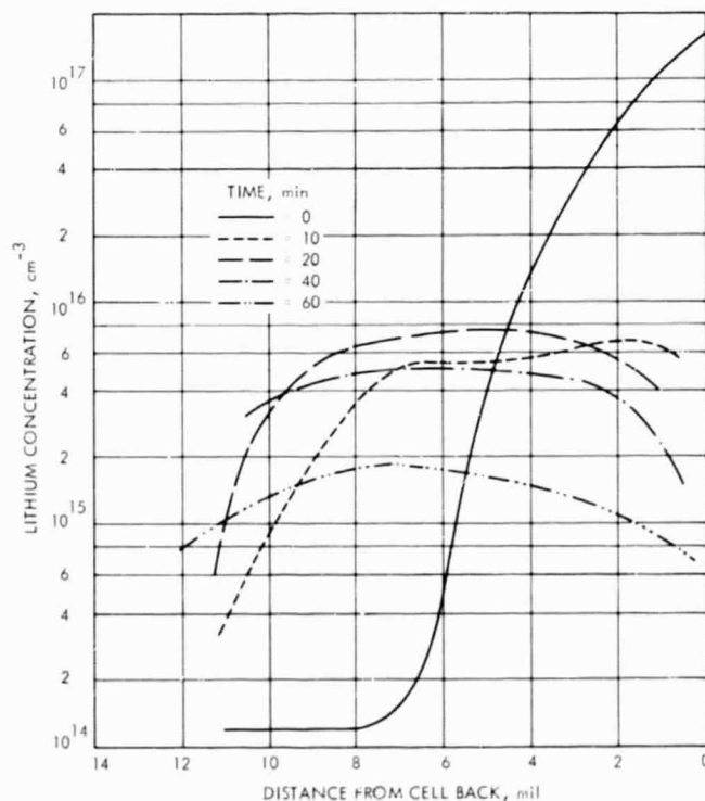
Fig. 1. Lithium concentration profiles following redistribution of a tack-on diffusion
