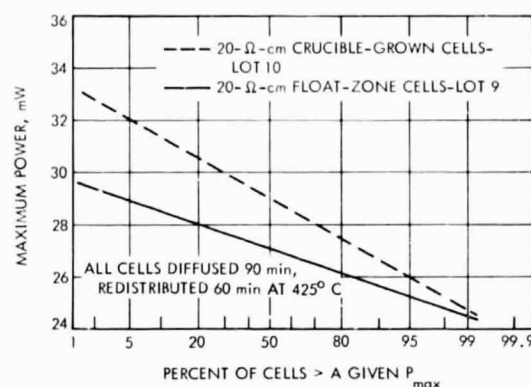
Fig. 6. Comparison of maximum power distributions of lots 9 and 10
