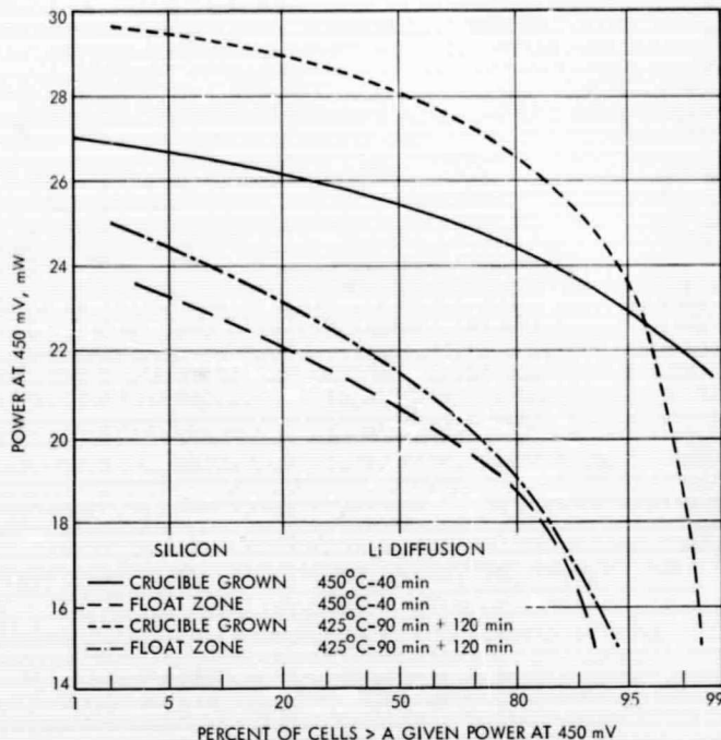
Fig. 9. Cumulative yields for cell shipment group C-5
