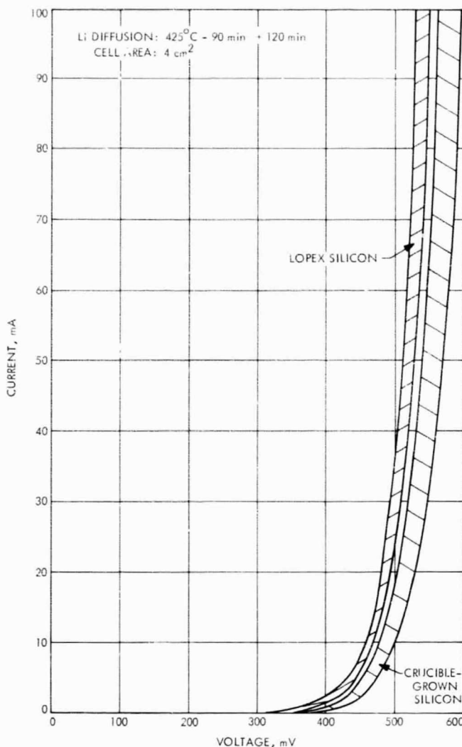
Fig. 6. Envelopes of dark forward I-V characteristics for two forms of silicon with same diffusion schedule
