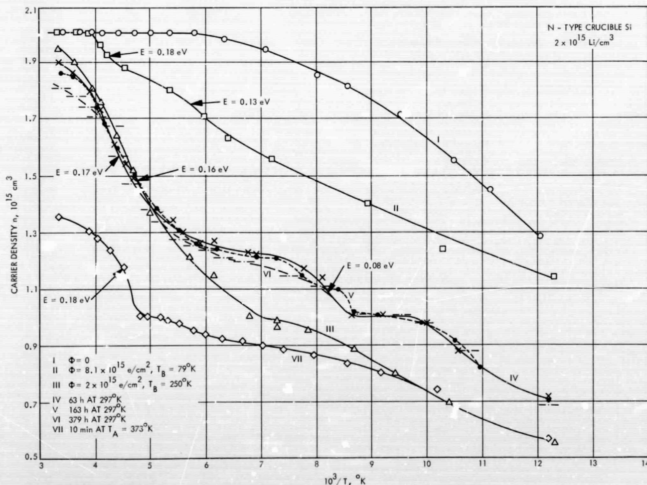
Fig. 14. Carrier-density vs reciprocal temperature for high resistivity (2.5 \Omega -cm) crucible-grown silicon
