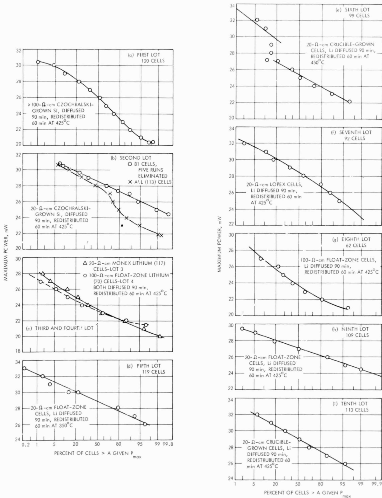
Fig. 4. Maximum power distribution of lithium cells fabricated for the ten shipment lots
