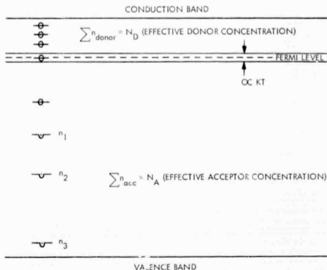
Fig. 1. Two-impurity model
