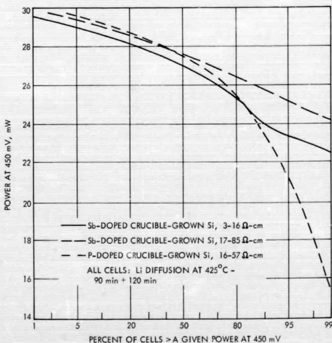
Fig. 10. Cumulative yields for cell shipment group C-6
