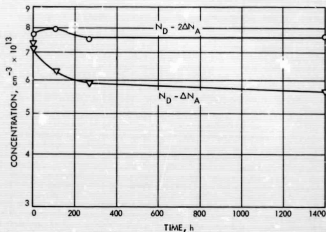
Fig. 6. Relative changes in acceptor and donor concentration
