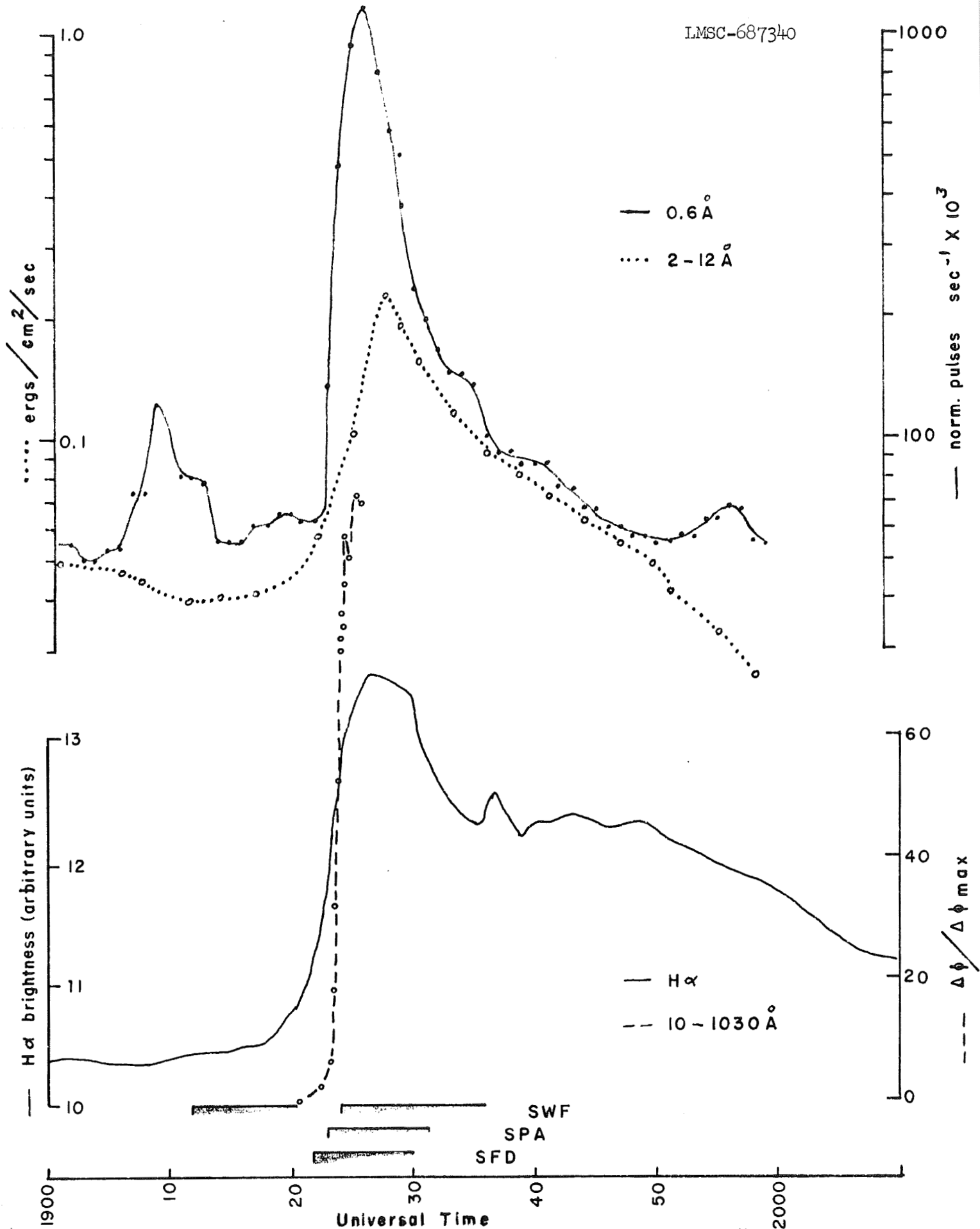
Figure 9. A comparison of H-alpha brightness, hard x-rays ( <0.6\text{\AA} ) and soft x-rays, (2-12Å) and EUV (10-1030Å) radiation for a flare on 21 May 1967.
