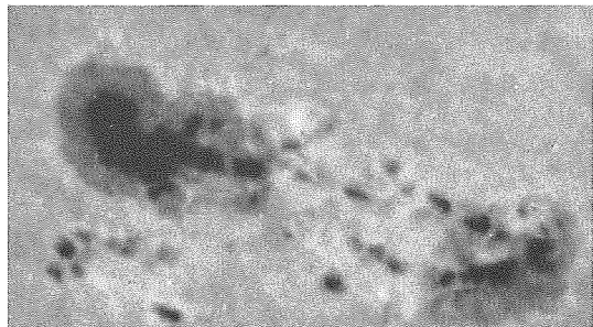
Figure 3. Flare points in the wings of \text{H}\alpha distinctly show an asymmetry favoring the red wing of the line. This red wing asymmetry is typical of flares in \text{H}\alpha (Ellison 1949).
