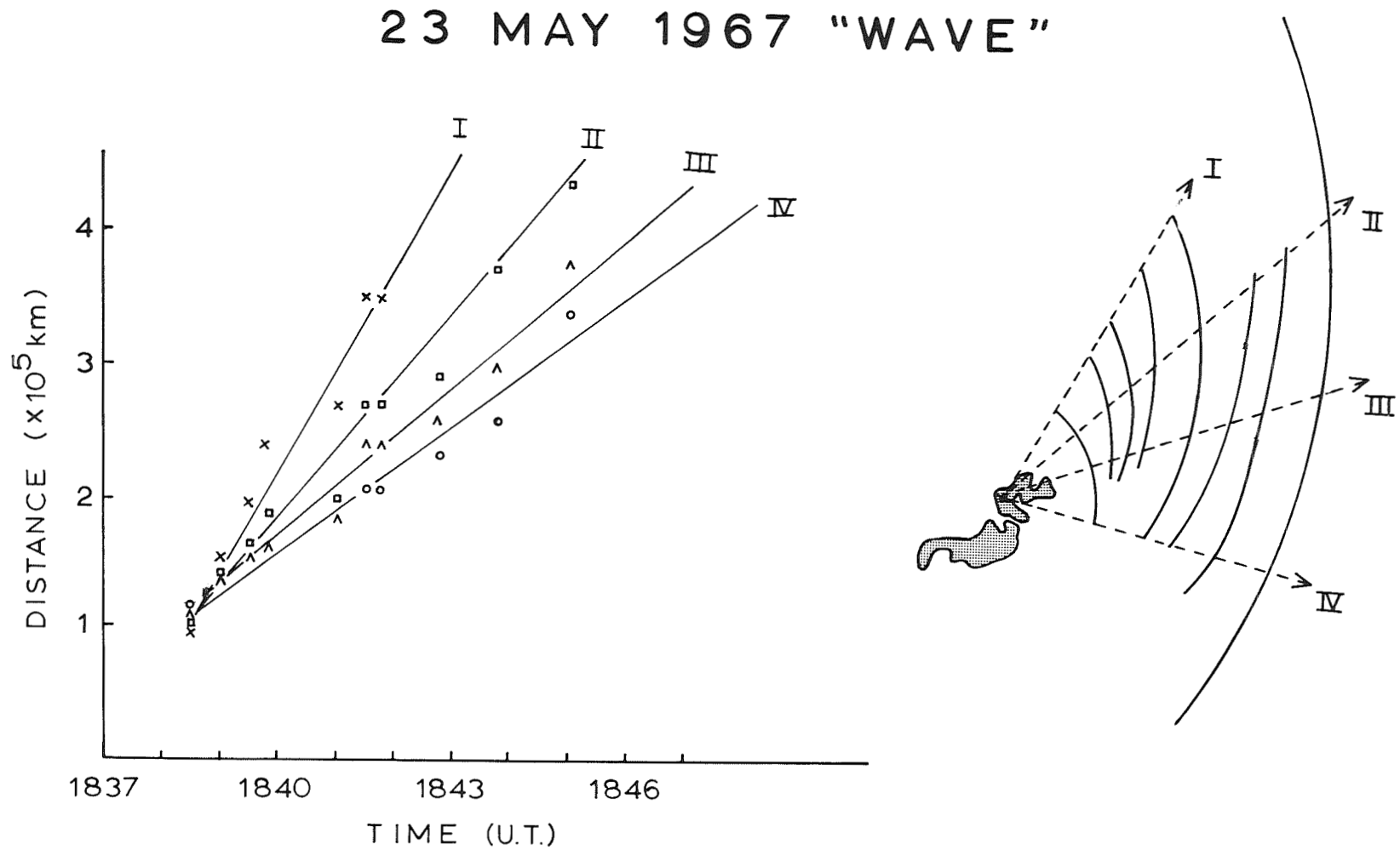
Figure 5. Diagram of the wave associated with the brightest flare on 23 May 1967. The measured velocity of the wave varies from 750 to 1125 Km across the wave front.
