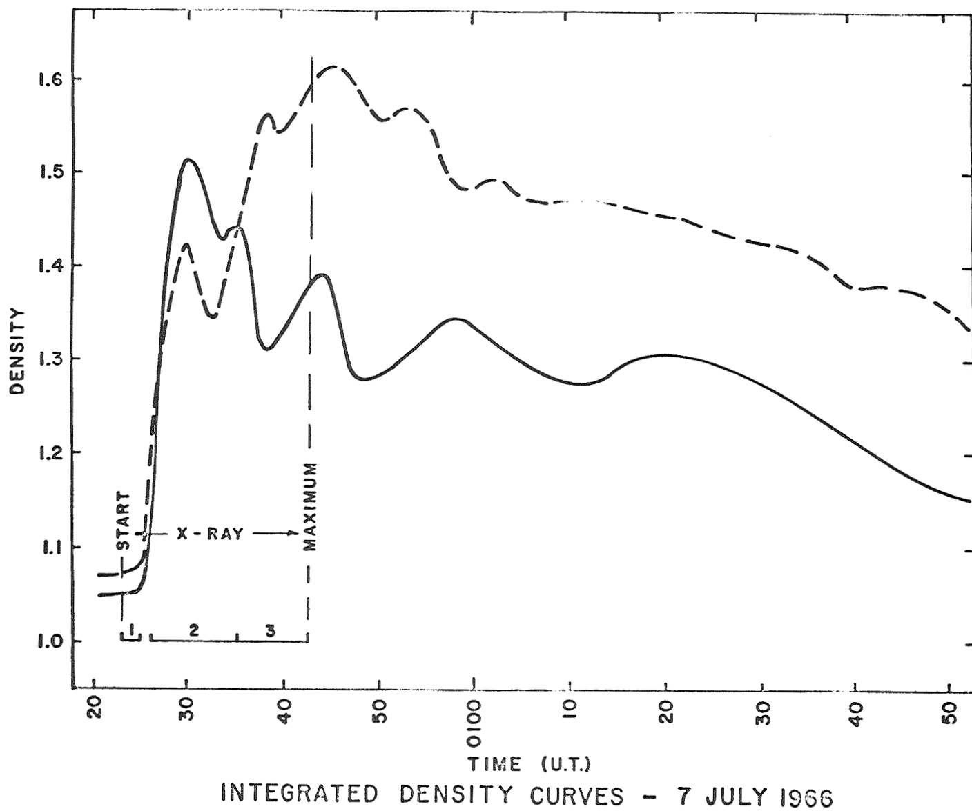
Figure 11. An H-alpha light curve of two segments of a flare compared to 3 phases in the associated x-ray event.
