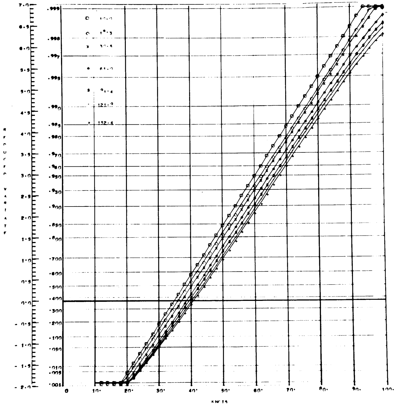
Fig.21 - Surface Wind Cumulative Distributions
