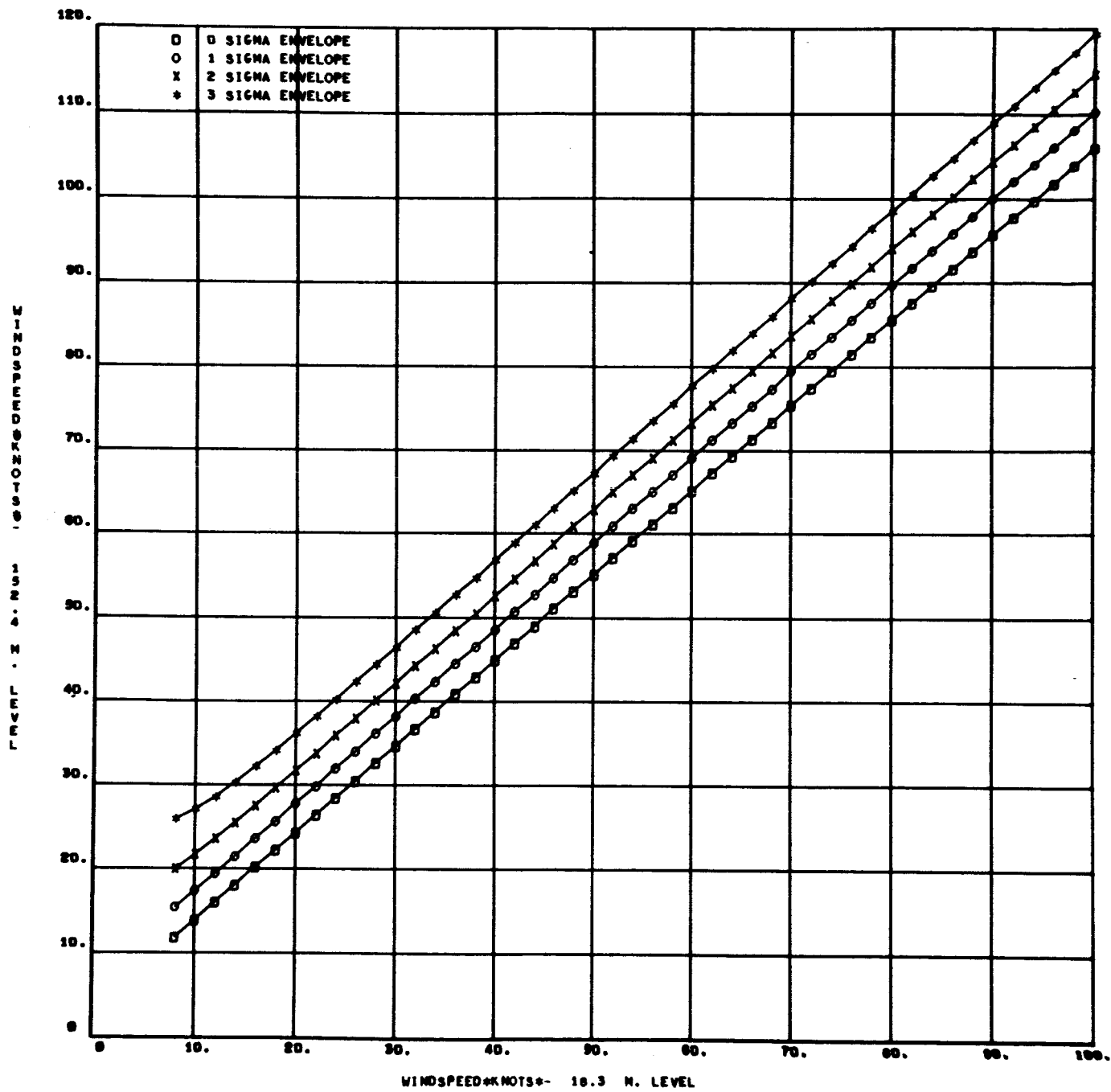
Fig.48 - Wind Profile Plots
