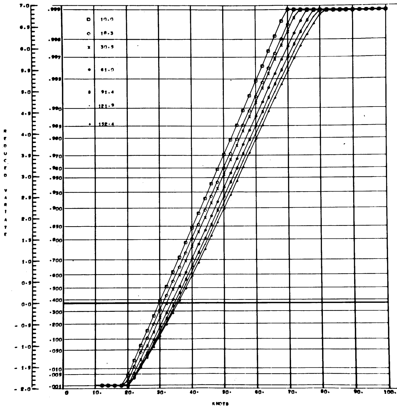
Fig. 9 - Surface Wind Cumulative Distributions
