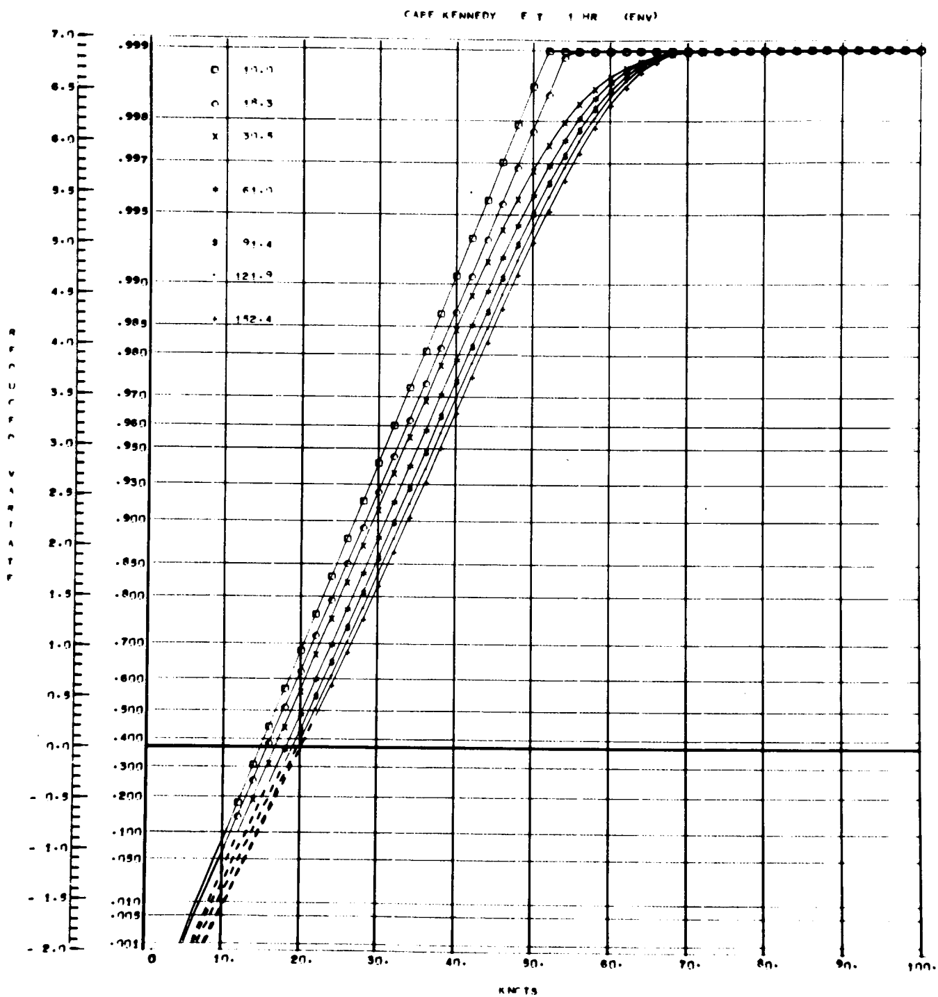
Fig. 15 - Surface Wind Cumulative Distributions
