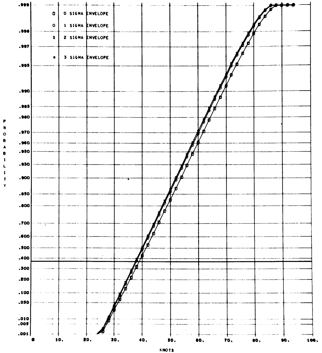
Fig. 33 - Surface Wind Profile Cumulative Distributions
