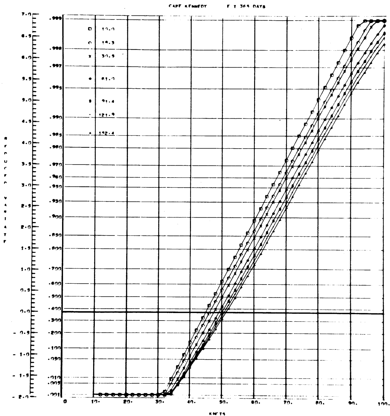
Fig. 14.- Surface Wind Cumulative Distributions
