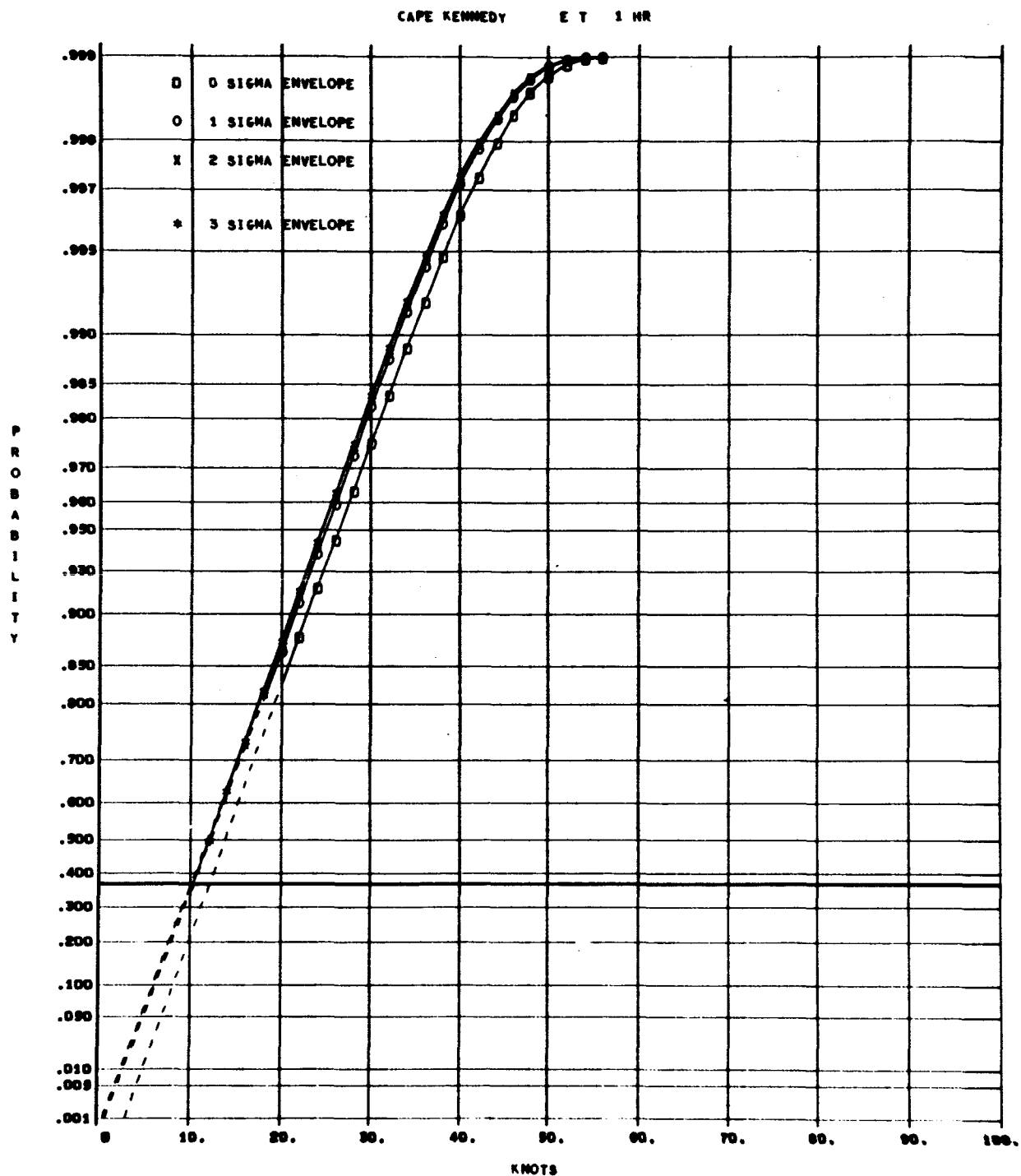
Fig.26 - Surface Wind Profile Cumulative Distributions
