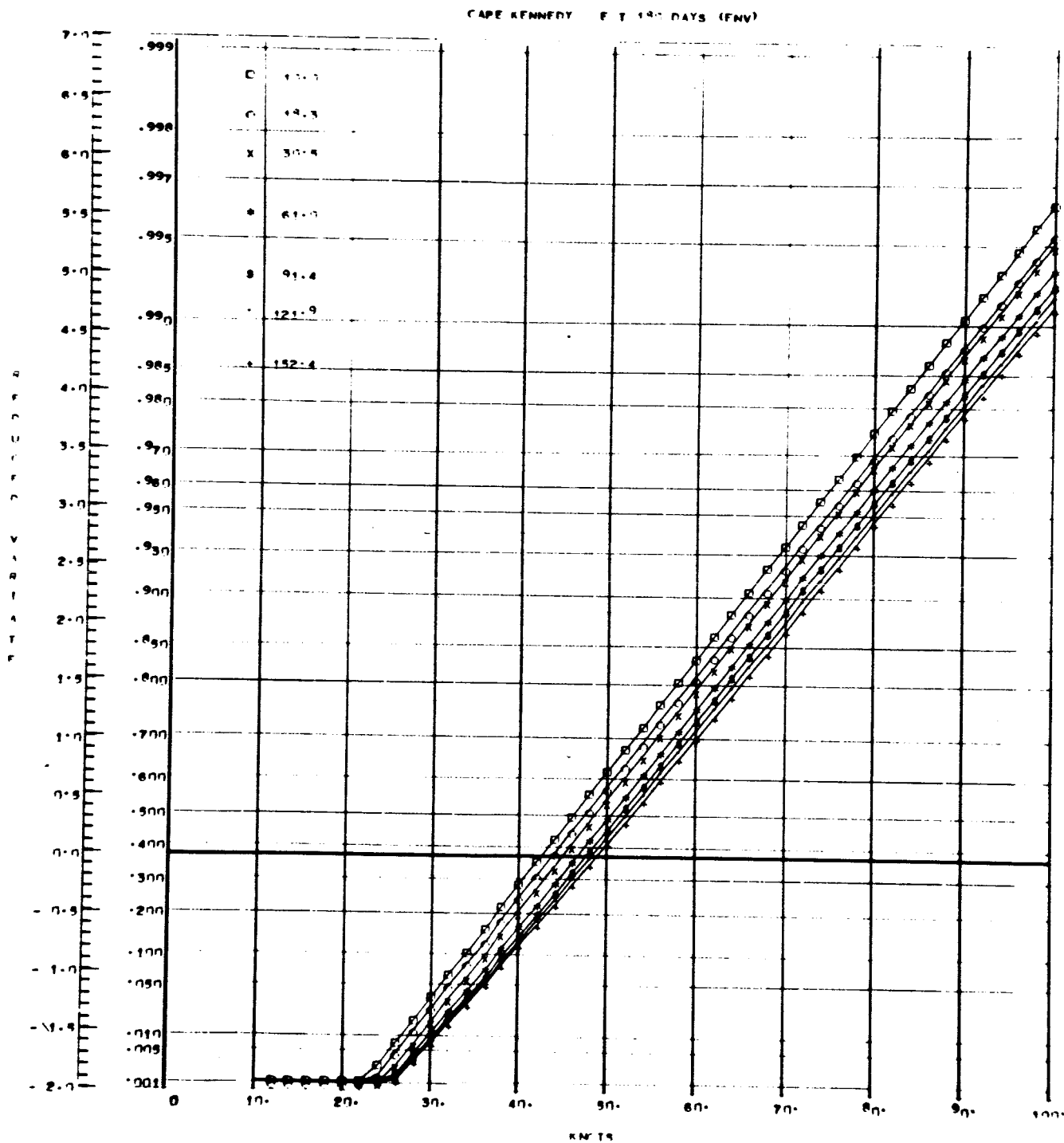
Fig.24 - Surface Wind Cumulative Distributions
