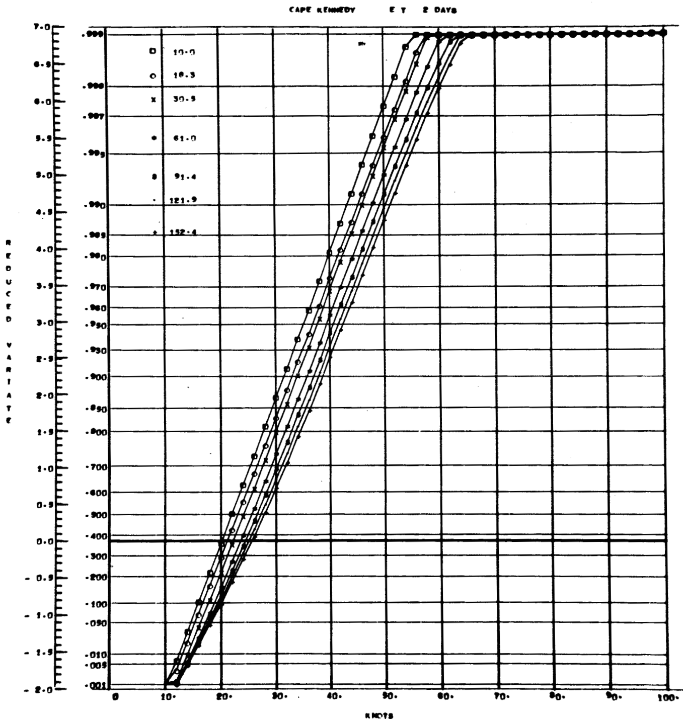
Fig. 6 - Surface Wind Cumulative Distributions
