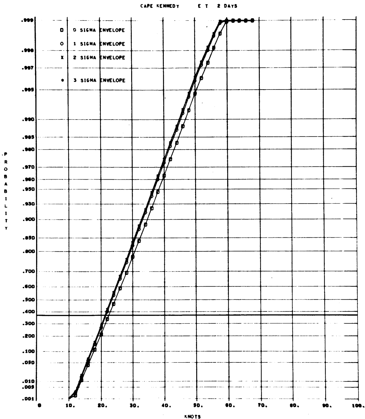
Fig.28 - Surface Wind Profile Cumulative Distributions
