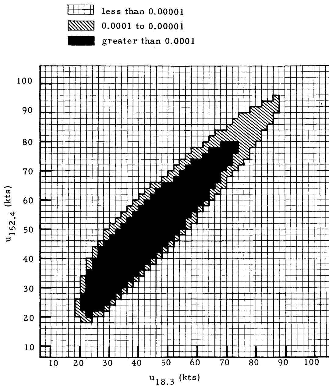
Fig. 3 - Joint Probability Plot for Cape Kennedy (30-Day, Annual Reference Period)
