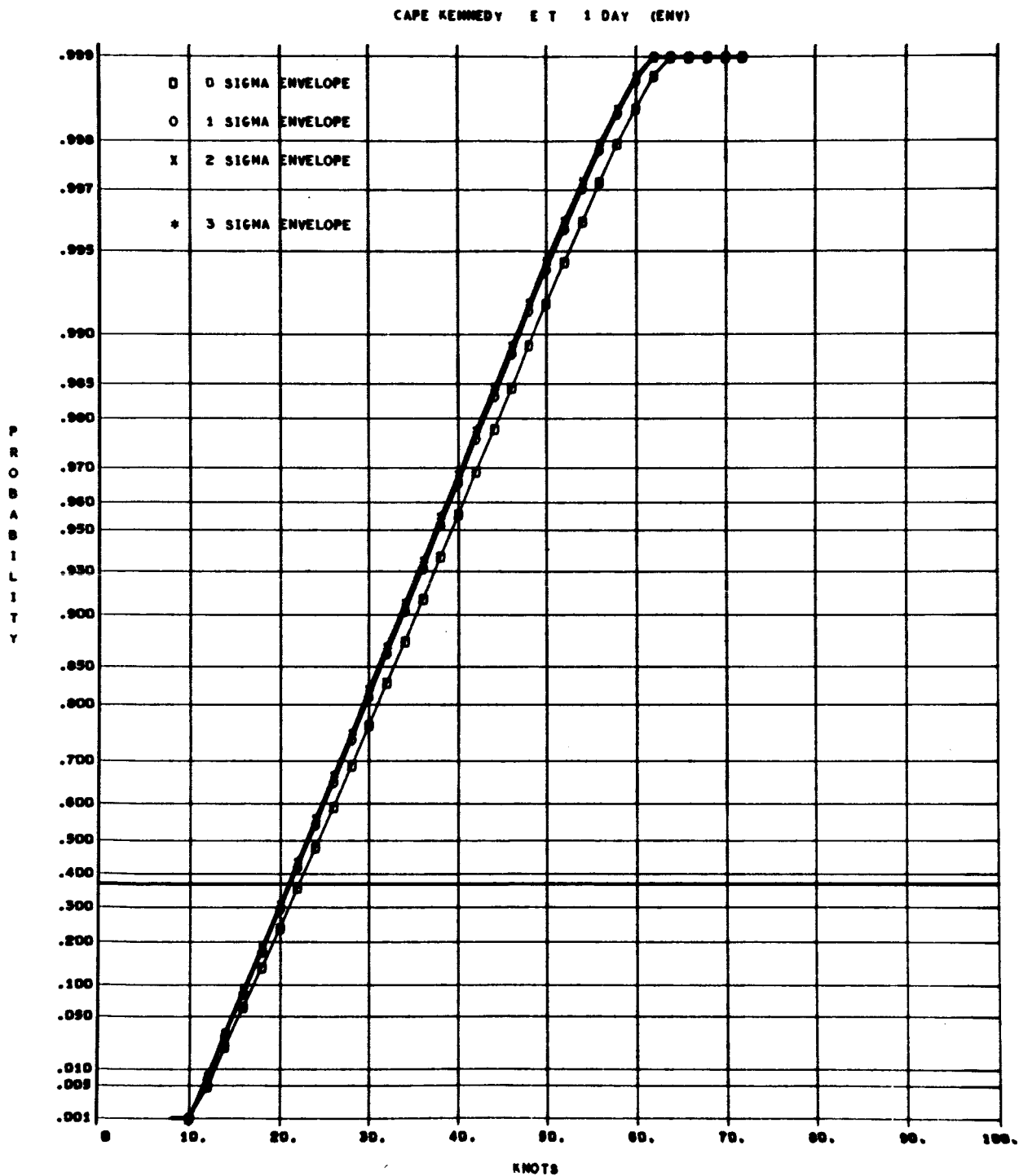
Fig. 38 - Surface Wind Profile Cumulative Distributions
