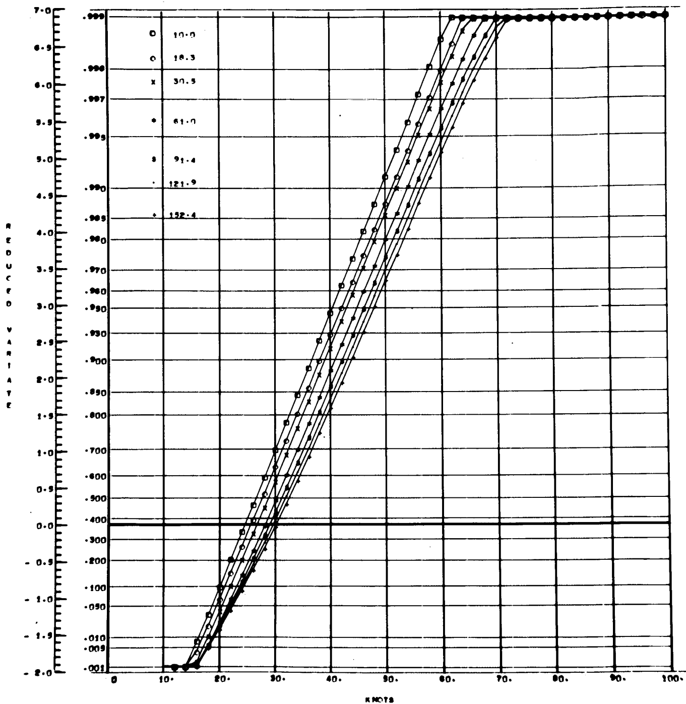
Fig. 7 - Surface Wind Cumulative Distributions
