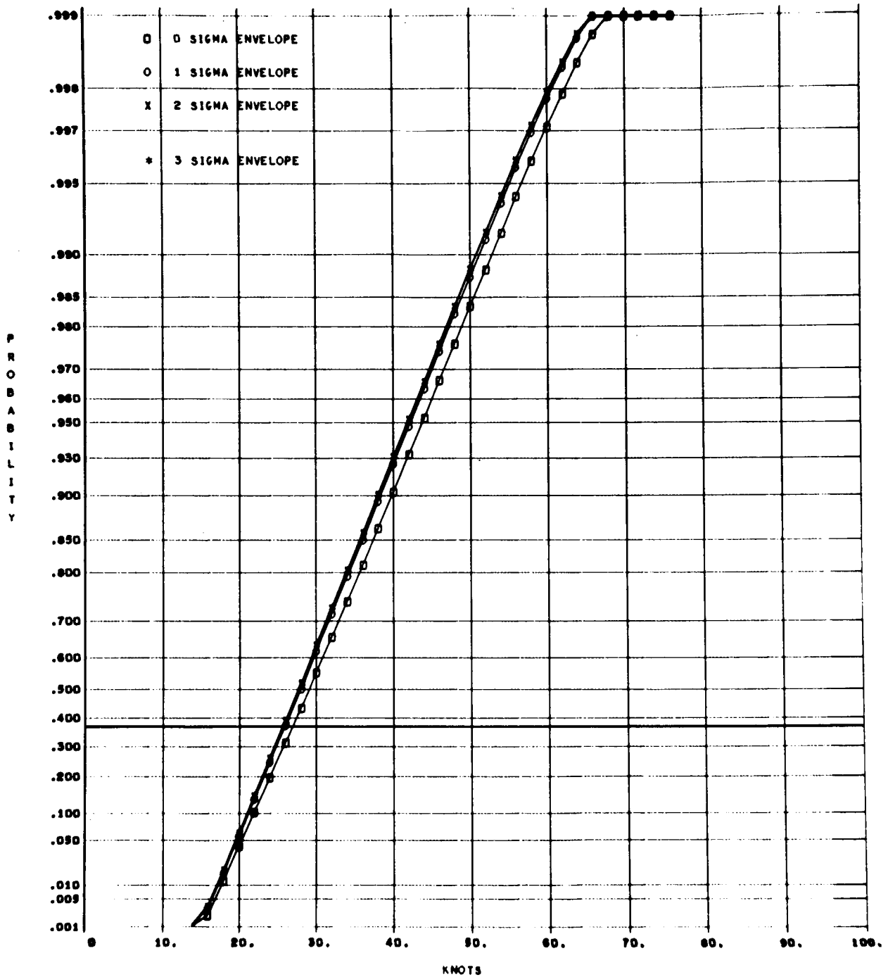
Fig.29 - Surface Wind Profile Cumulative Distributions
