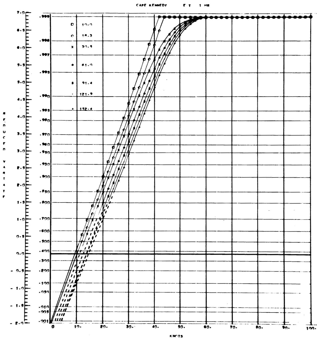
Fig. 4 - Surface Wind Cumulative Distributions
