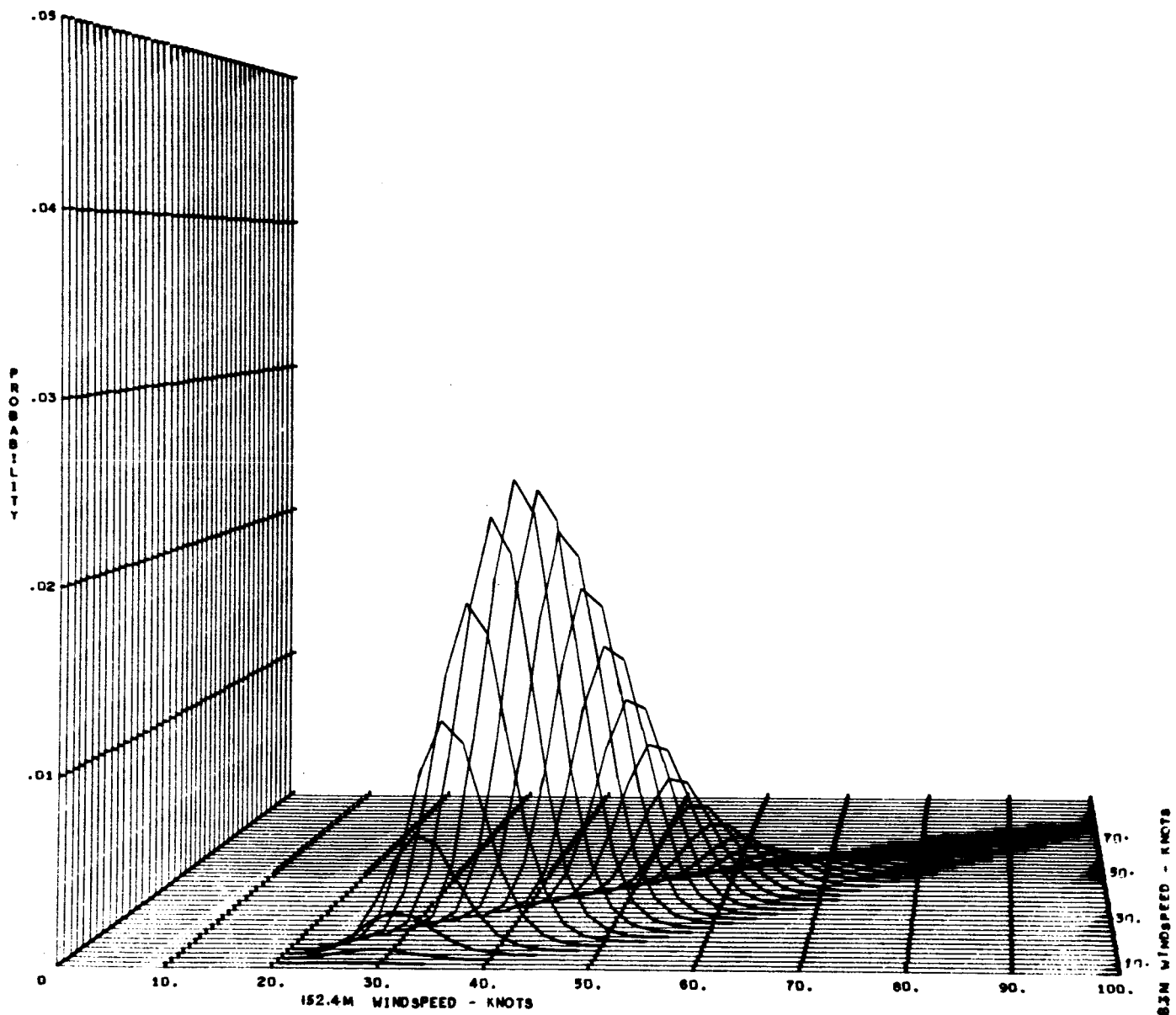
Fig.2 - Joint Probability Curve for Cape Kennedy (30-Day, Annual Reference Period)
