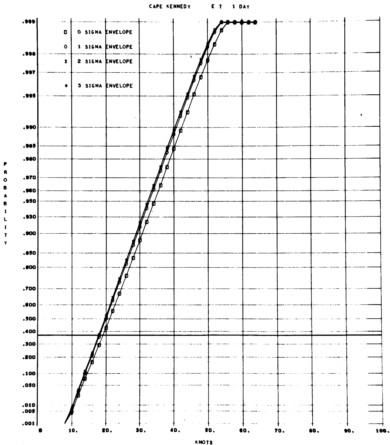
Fig. 27 - Surface Wind Profile Cumulative Distributions
