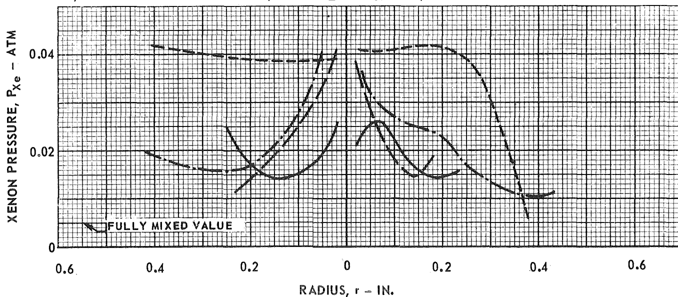
b) XENON PARTIAL PRESSURE (FROM XEI 4671 Å LINE)
