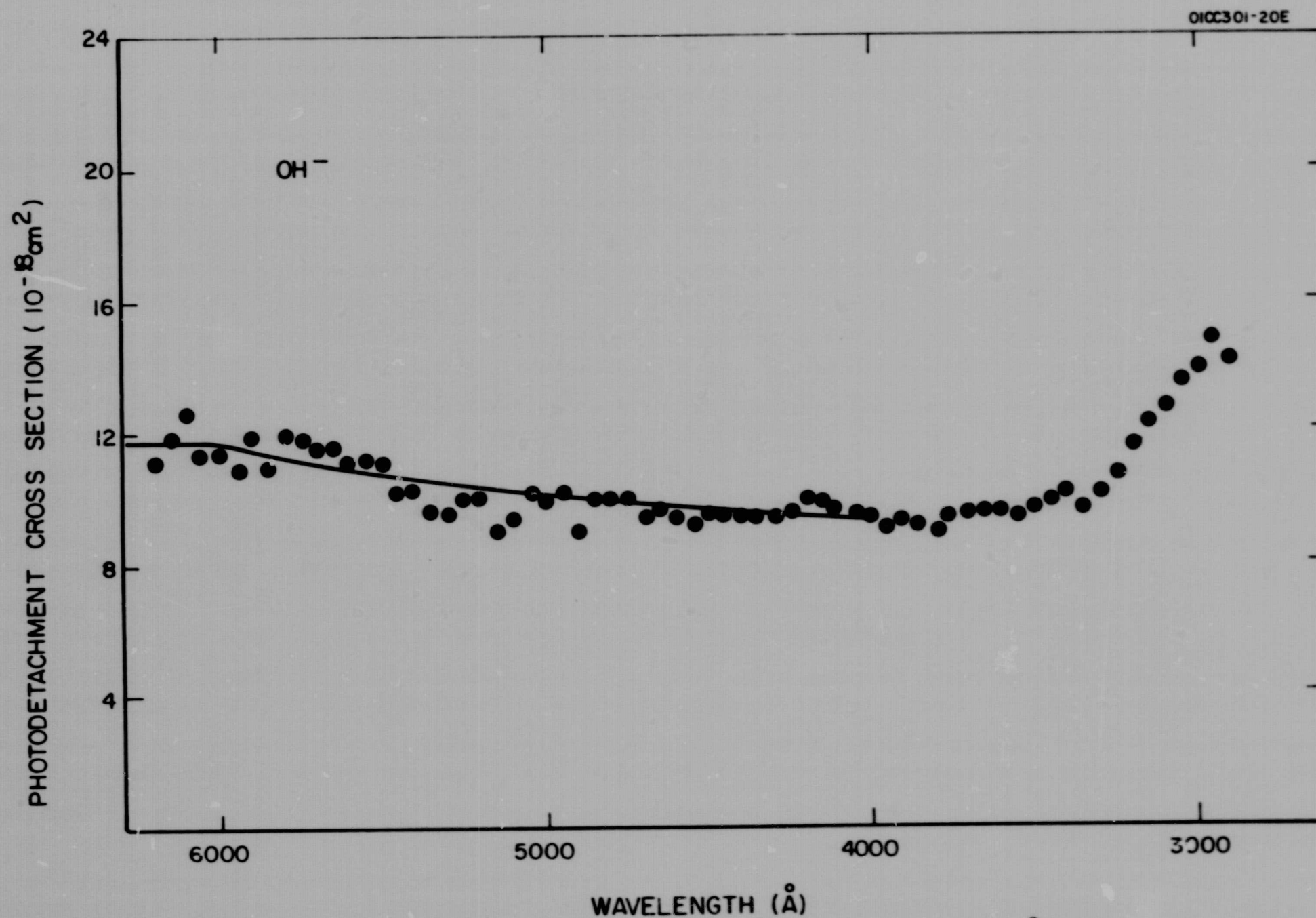
Figure 14. Photodetachment cross sections for \text{OH}^- spectral resolution 180\text{\AA} half width. Solid curve refers to interpolated data by Branscomb (Ref. 26).
