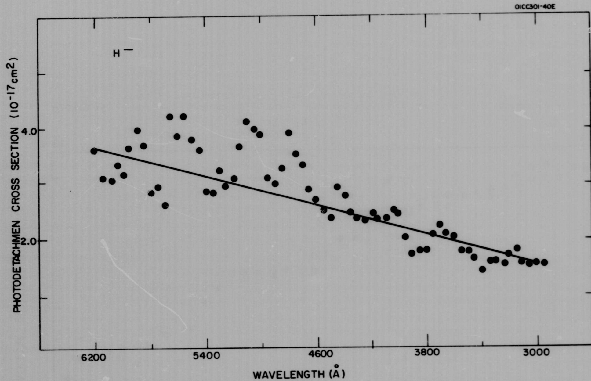
Figure 9. Photodetachment cross sections of H^- versus wavelength, obtained by using O^- as a standard. Spectral resolution 210\text{\AA} half width, solid line refers to theory.
