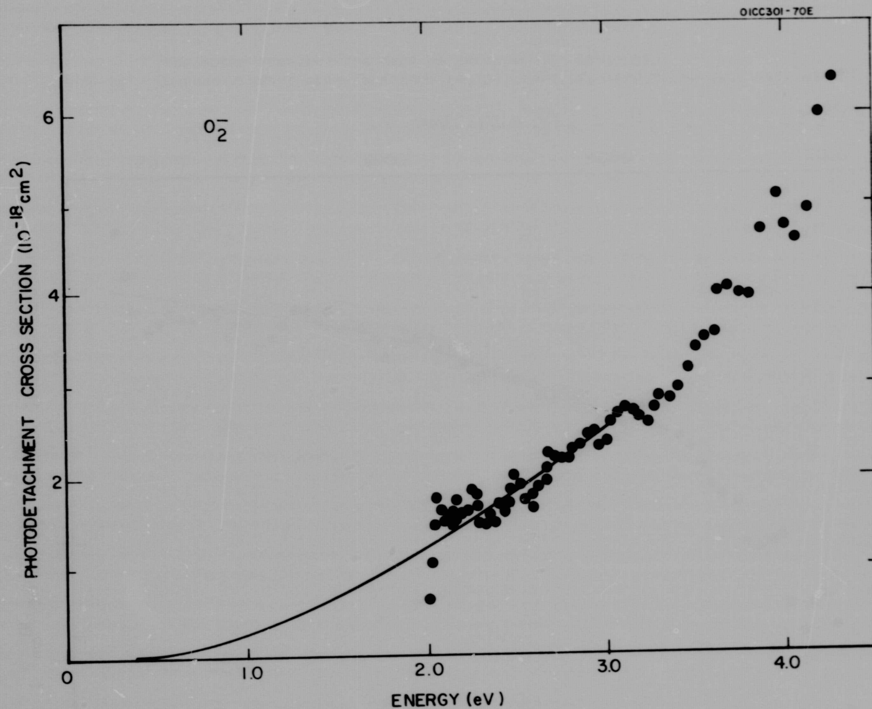
Figure 13. Photodetachment cross sections for \text{O}_2^- similar to Figure 12 but plotted versus energy.
