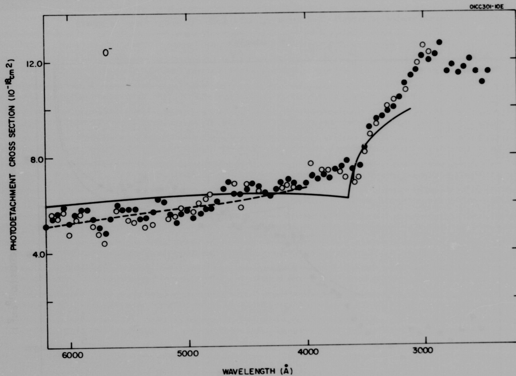
Figure 7. Photodetachment cross sections for O^- . Filled points, without filter; Open points, with Pyrex filter. Spectral resolution 180\text{\AA} half width; Solid line, interpolated data of Branscomb, et al. (Ref. 8); broken line, interpolated data by Branscomb, Burch, et al. (Ref. 9).
