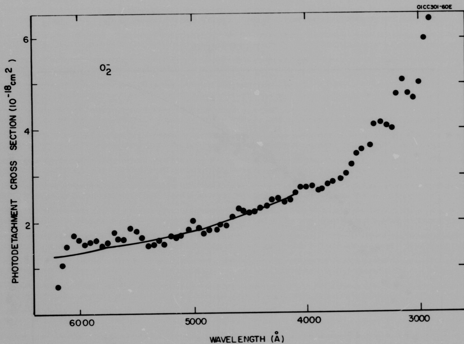
Figure 12. Photodetachment cross sections for O_2^- spectral resolution 180\text{\AA} half width. Solid line shows interpolated data by Burch et al. (Ref. 22).
