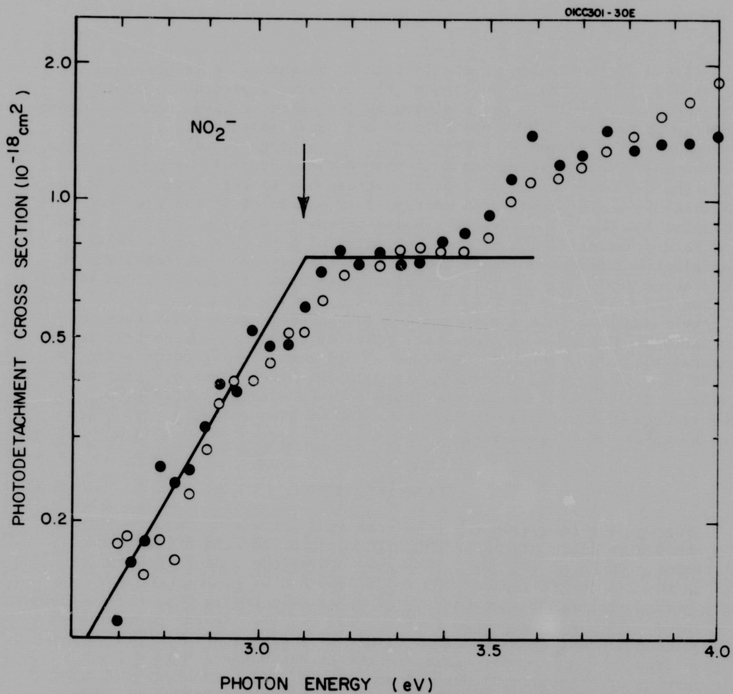
Figure 11. Photodetachment cross sections for \text{NO}_2^- plotted semi-logarithmically versus energy, to show break in the curve of 3.1 eV.
