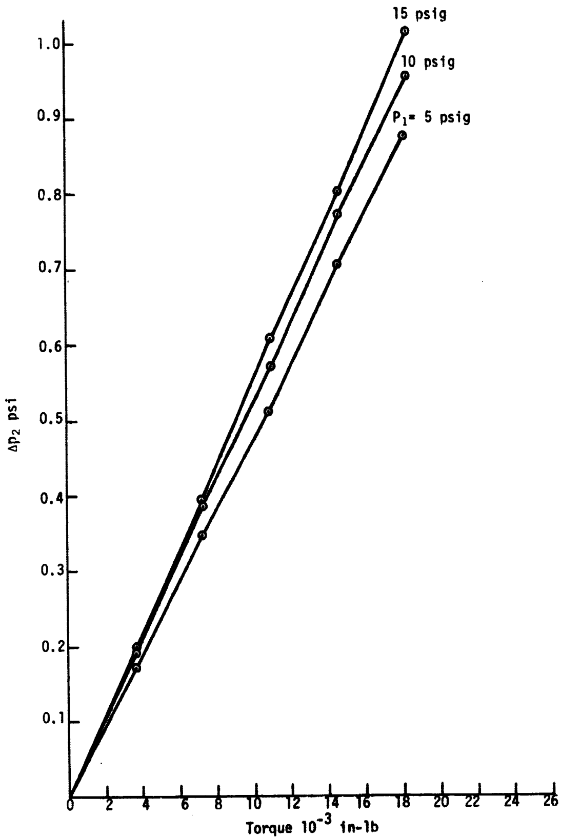
Figure 23. Pneumatic System: P_1 Load Versus Differential Pressure \Delta P_2 for the Closed Loop System at Room Temperature
