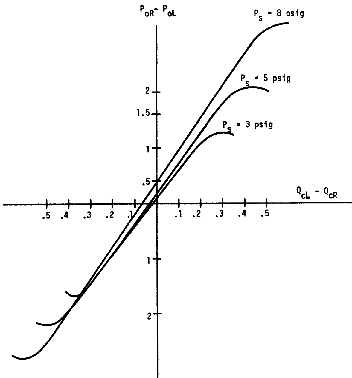
Figure 36. Fluidic Amplifier: Transfer Characteristics - 70°F
