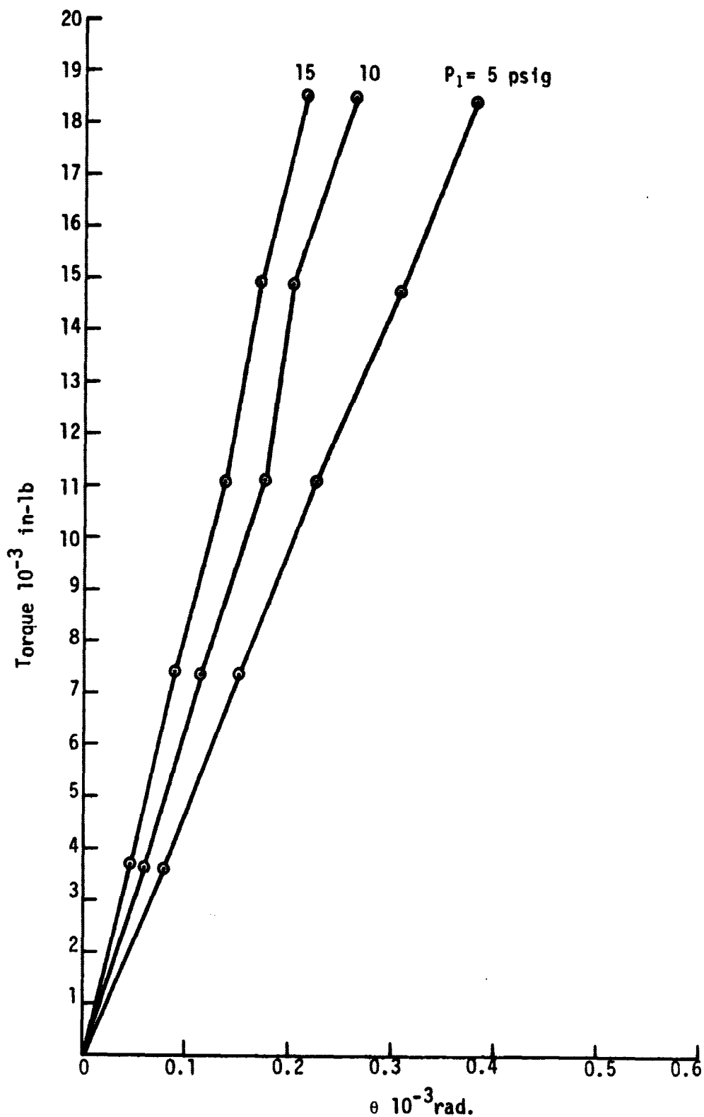
Figure 22. Pneumatic System: Load Versus Deflection Relation for the Closed Loop System at 2000^{\circ}\text{F}
