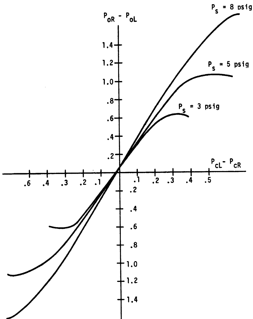
Figure 38. Fluidic Amplifier: Transfer Characteristics - 2000°F
