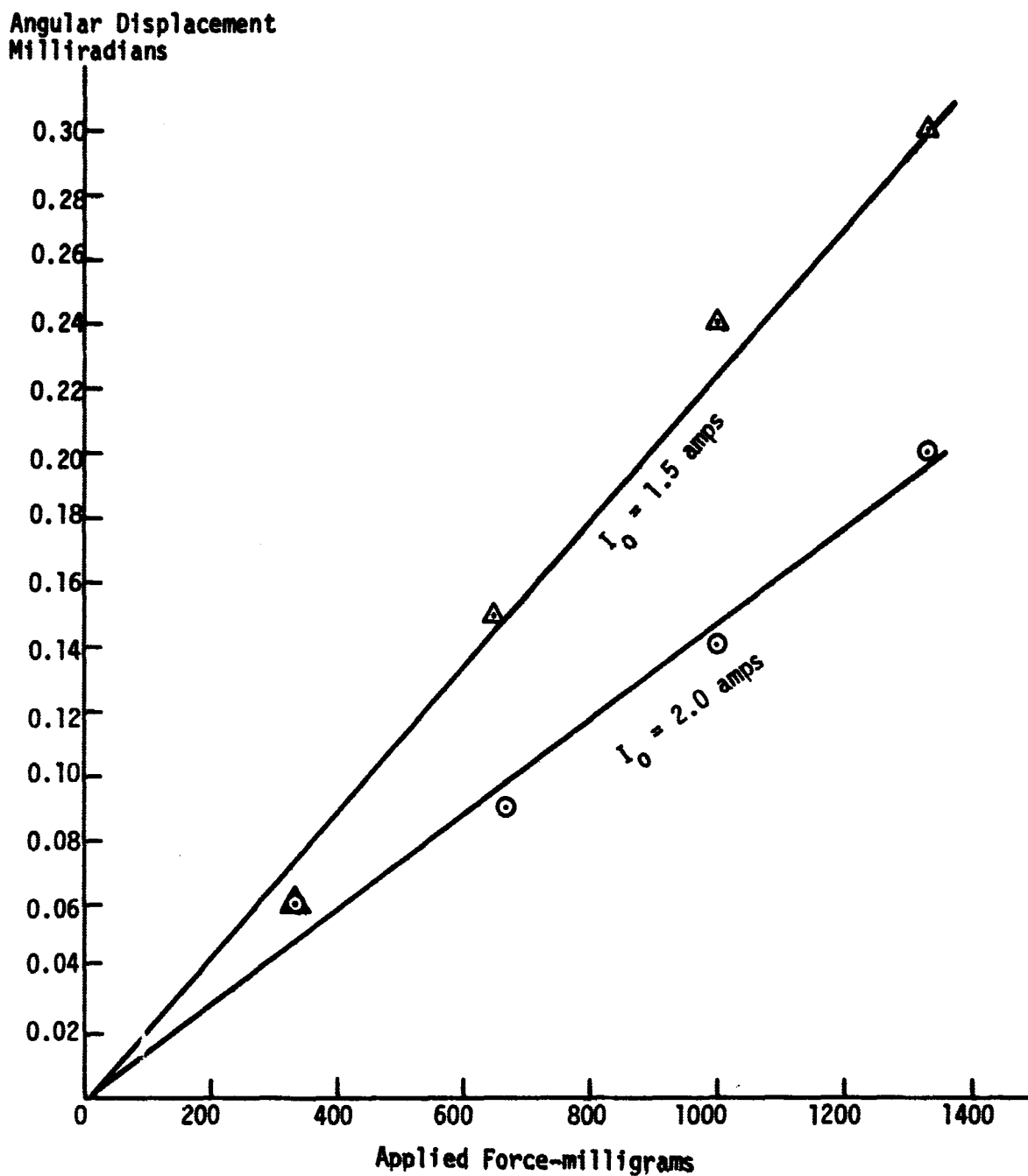
Figure 13. Cobalt Motor-Sensor: Steady-State Displacement Data at Room Temperature (Air Gap = 0.025 inch)
