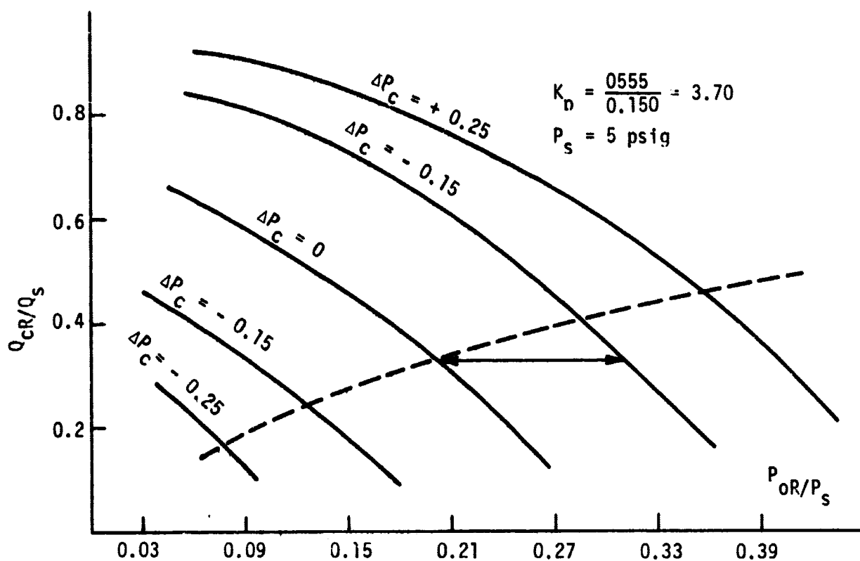
Output Characteristics
