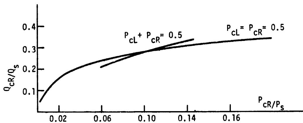
Input Characteristics
