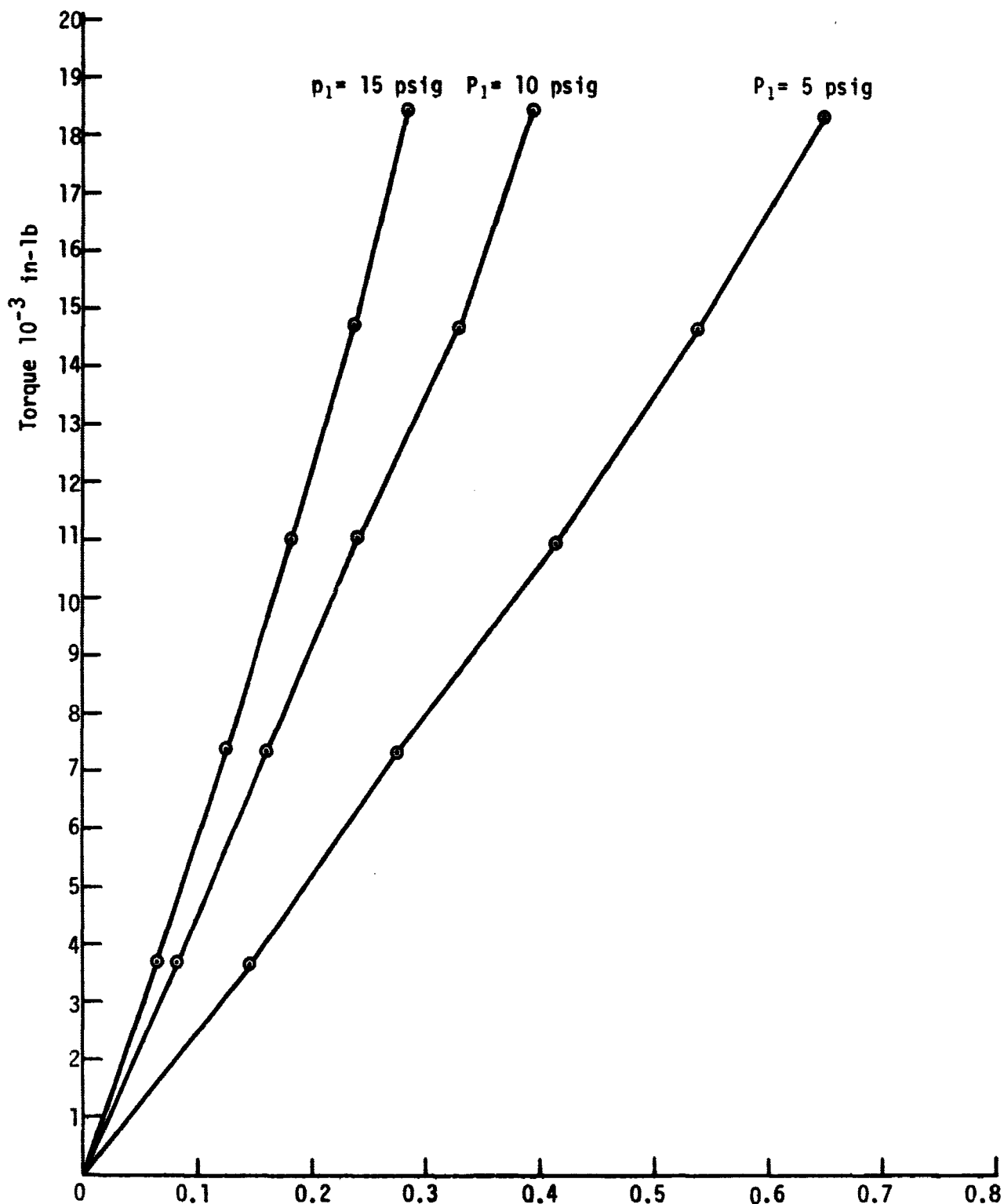
Figure 21. Pneumatic System: Load Versus Deflection Relation for the Closed Loop System at Room Temperature
