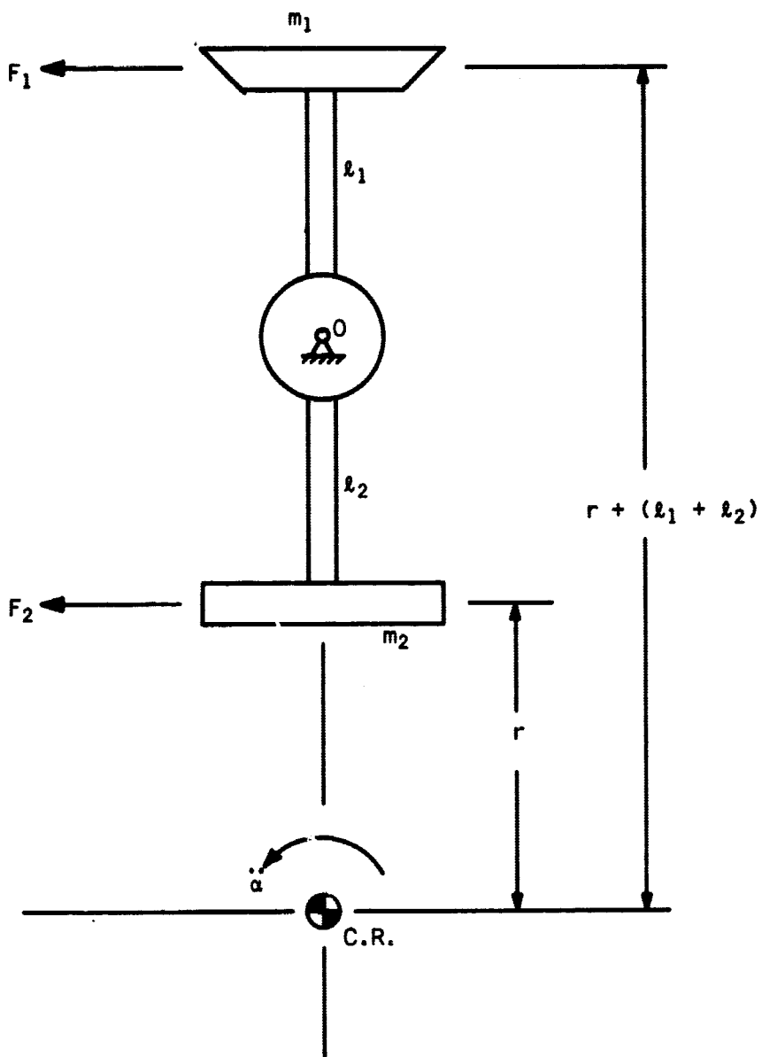
FIGURE 23. mm_1 Component with Forces Due to Angular Accelerations
