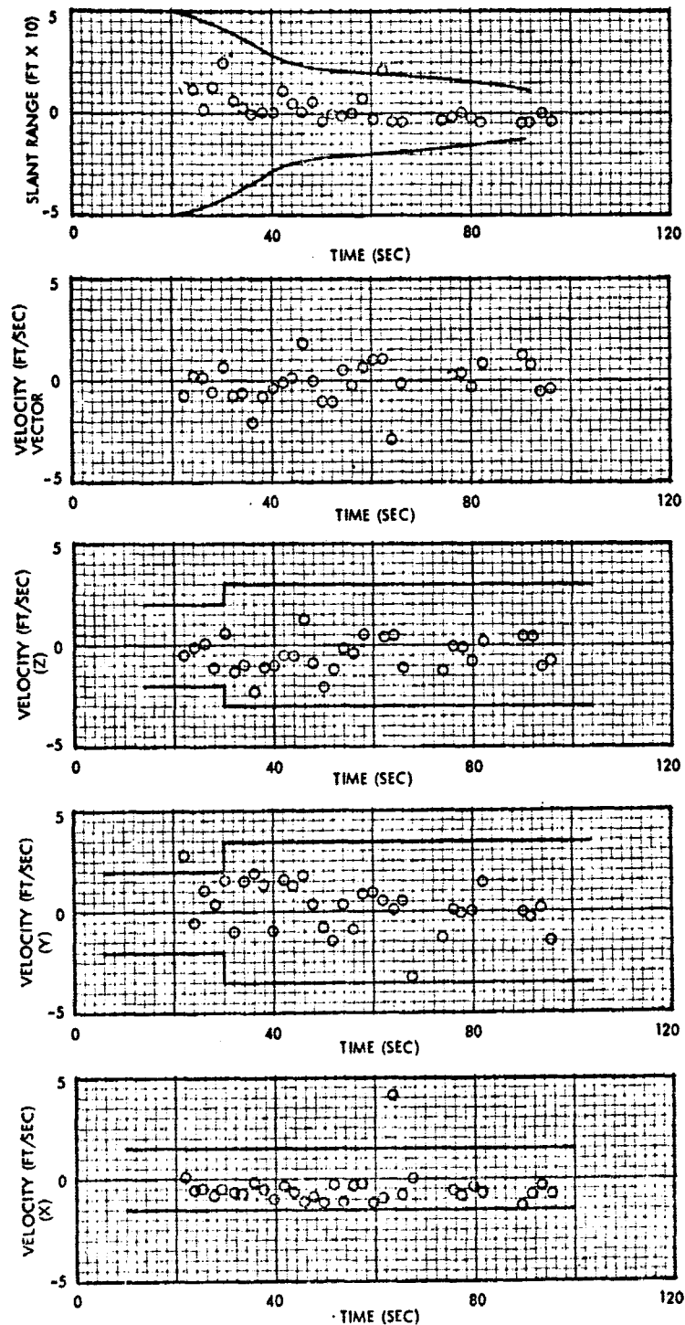
Figure 12. LR-60J, Pass 7, Cinetheodolite-Landing Radar Differences
