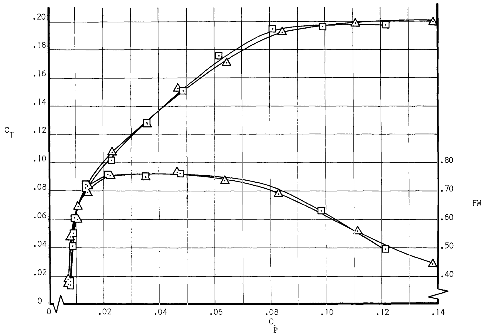
Figure 9 C_T Versus C_P For Propeller B
