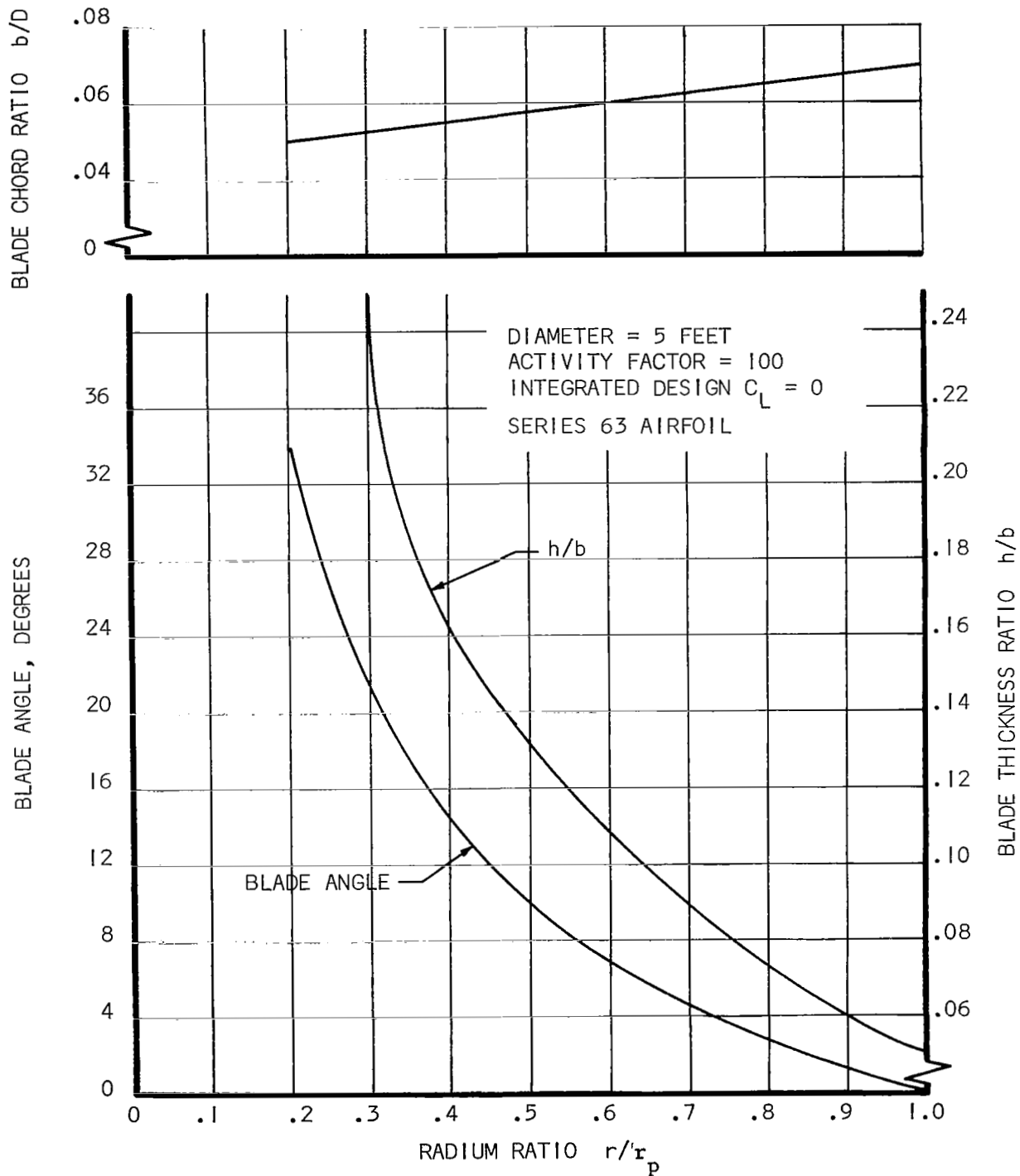
Figure 8 Propeller E
