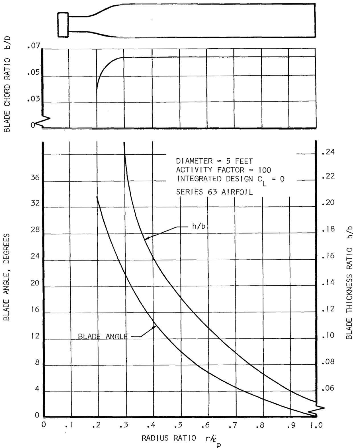
Figure 6 Propeller C
