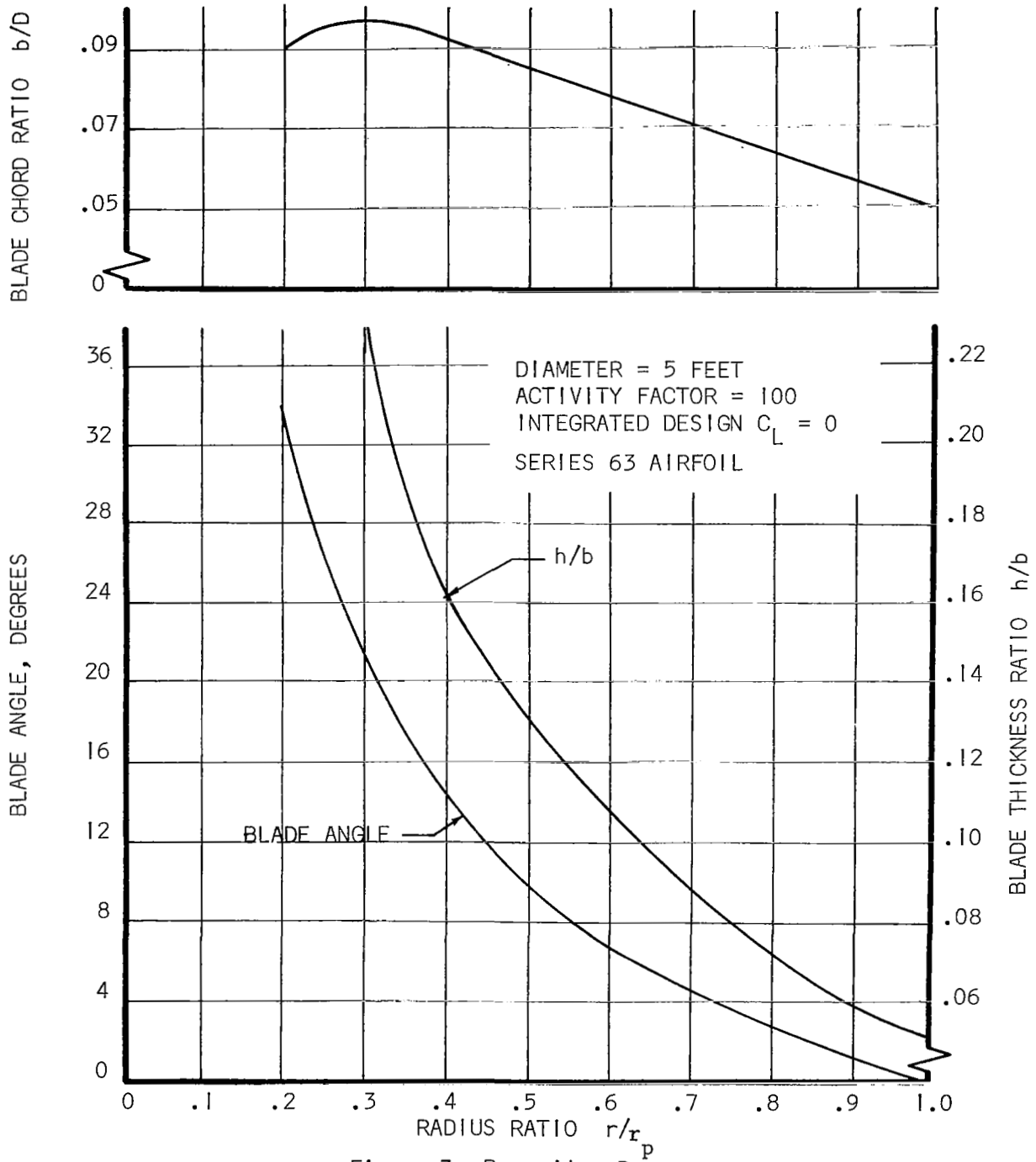
Figure 7 Propeller D
