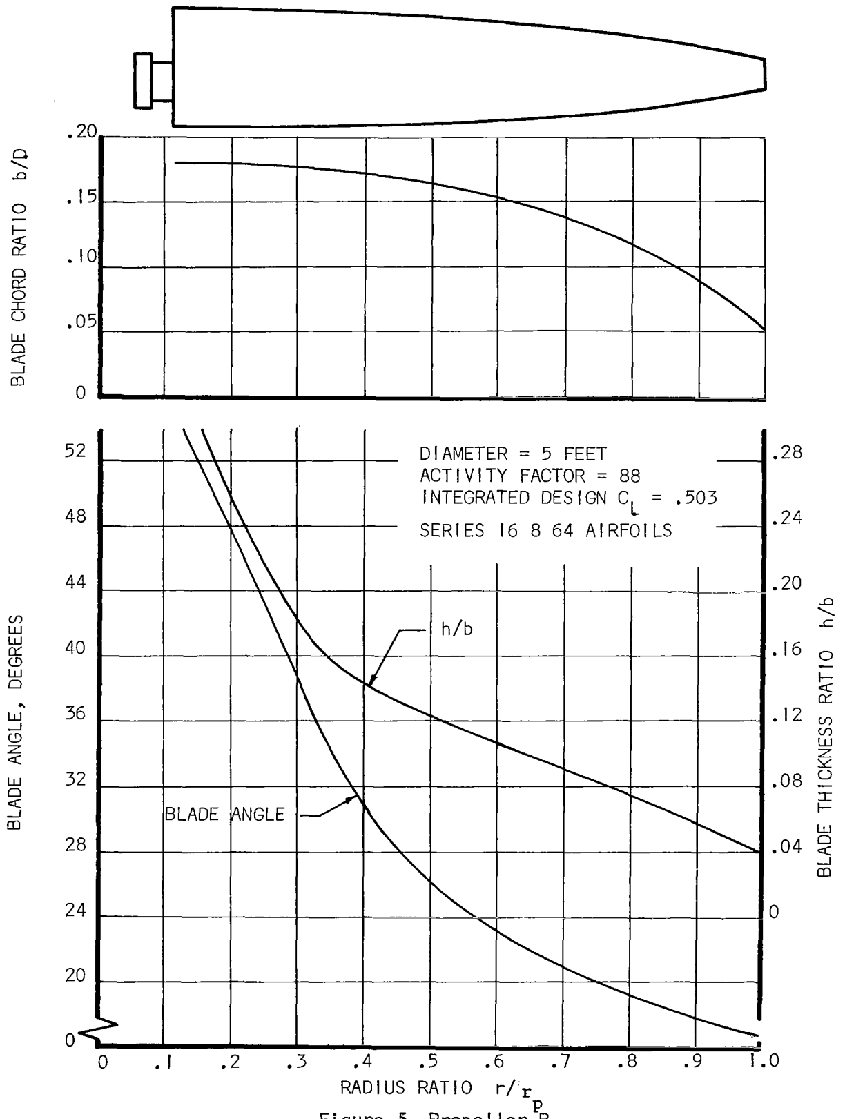
Figure 5 Propeller B
