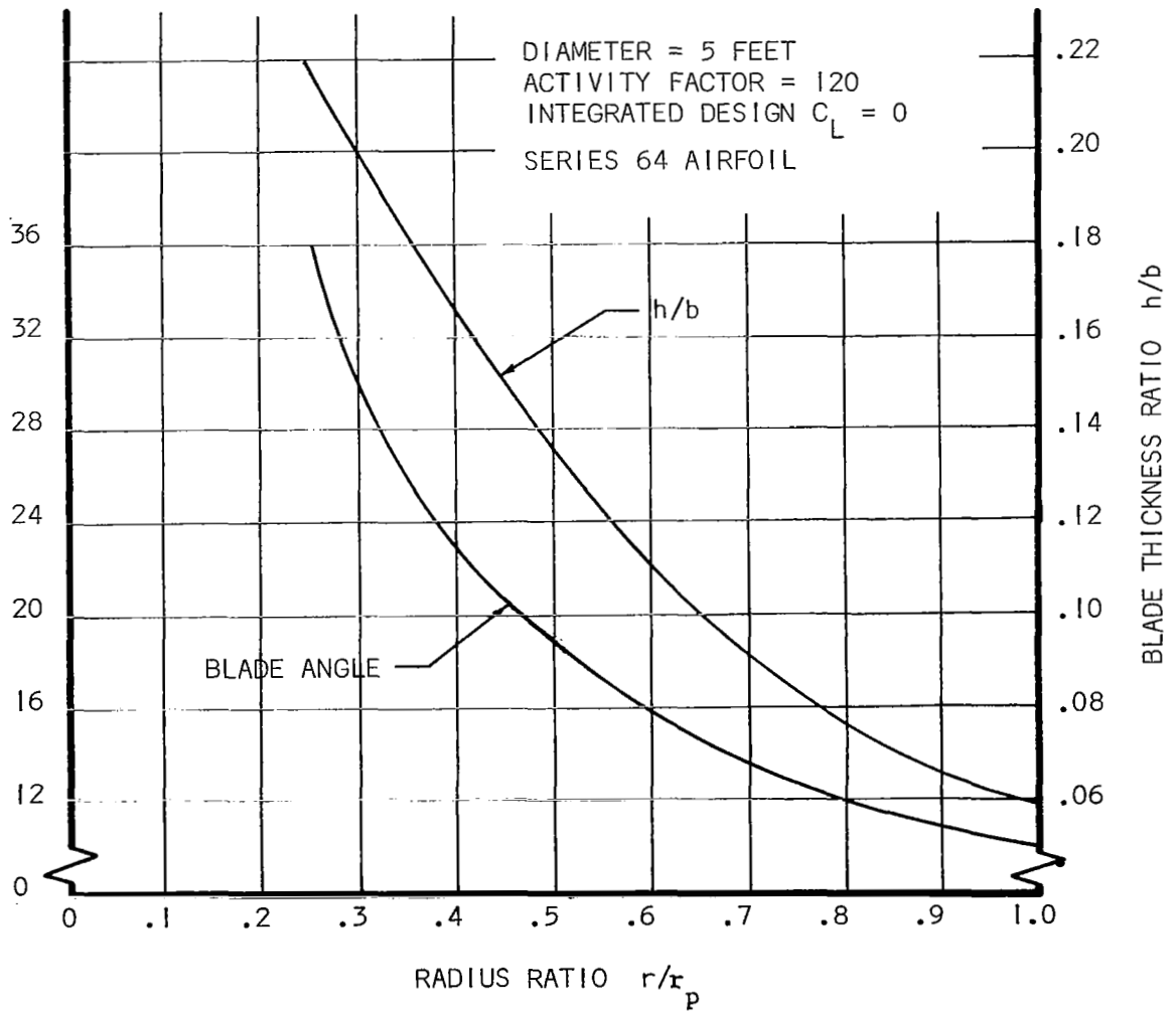
Figure 4 Propeller A
