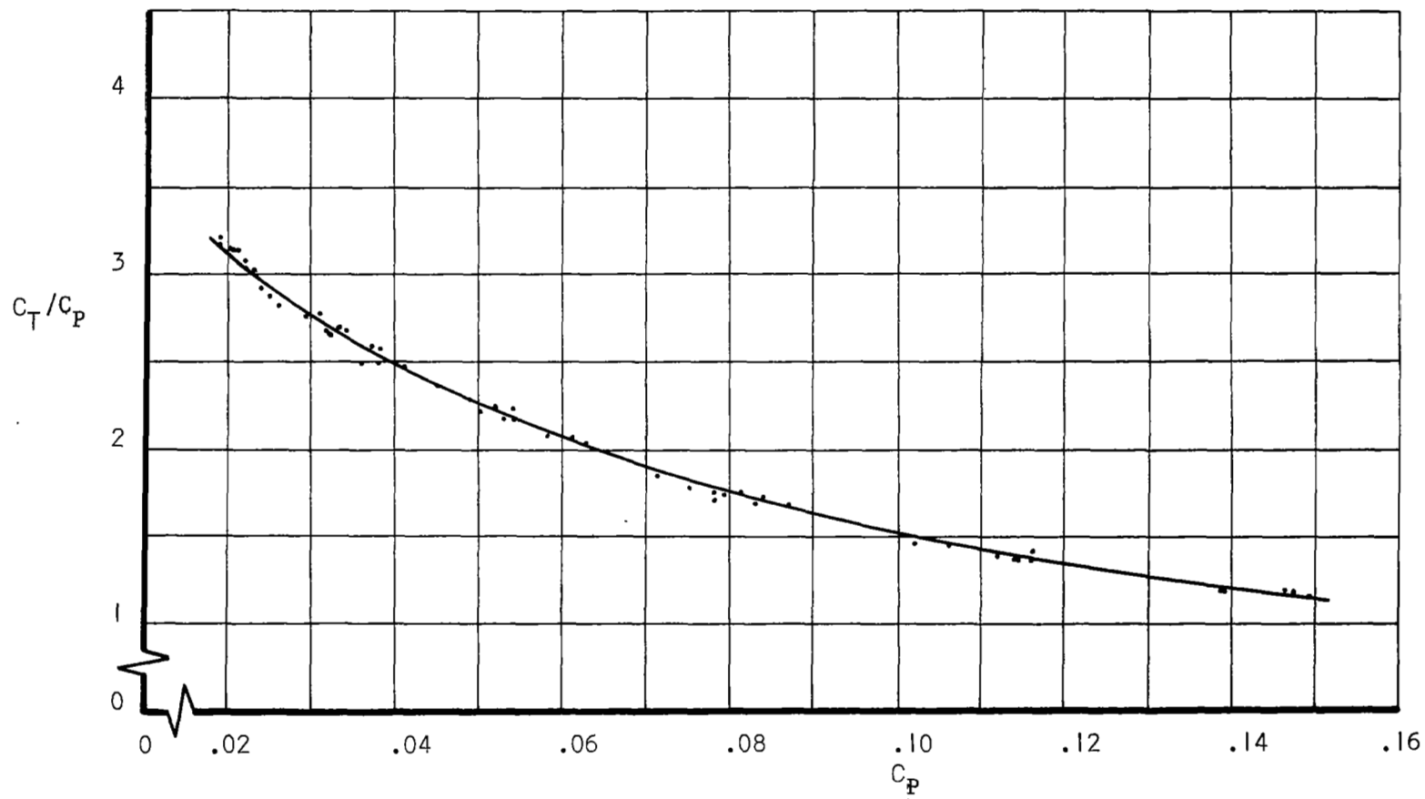
Figure 17 C_T/C_P Versus C_P For All Propellers
