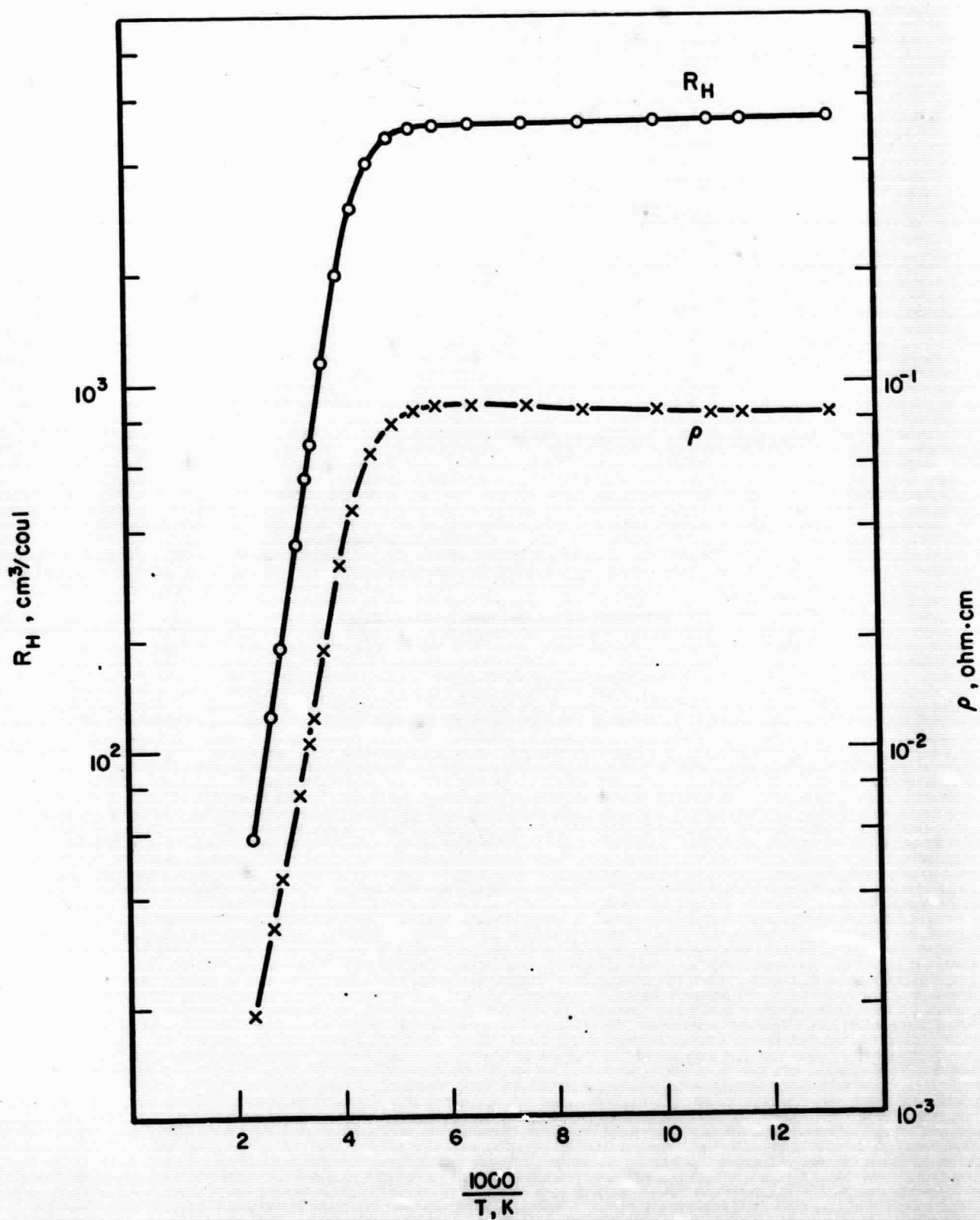
FIGURE 3. TEMPERATURE DEPENDENCE OF HALL COEFFICIENT AND RESISTIVITY FOR \text{Ga}_{0.15}\text{In}_{0.85}\text{Sb}
