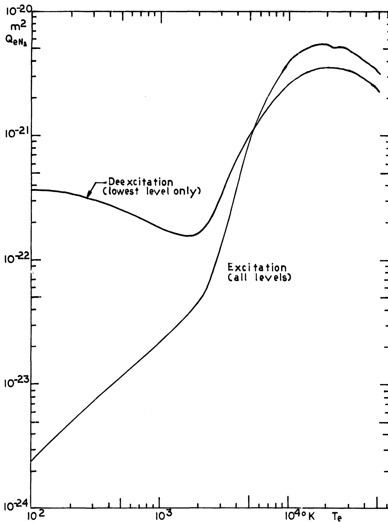
Figure E1. Excitation and de-excitation cross sections, Q_{eN_2, \text{ex}} and Q_{eN_2, \text{de}} , as a function of electron temperature for nitrogen
