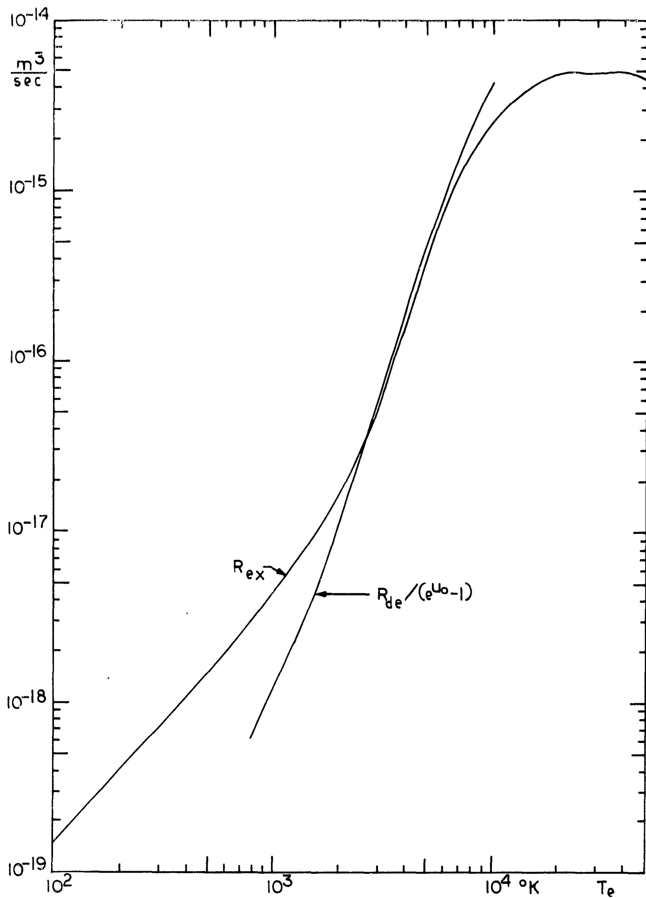
Figure E3. Excitation rate of nitrogen and de-excitation rate weighted by the ratio n_{N_2^*(v>0)}/n_{N_2(v=0)} of the number densities at equilibrium ( T_{vib} = T_e ), as a function of electron temperature
