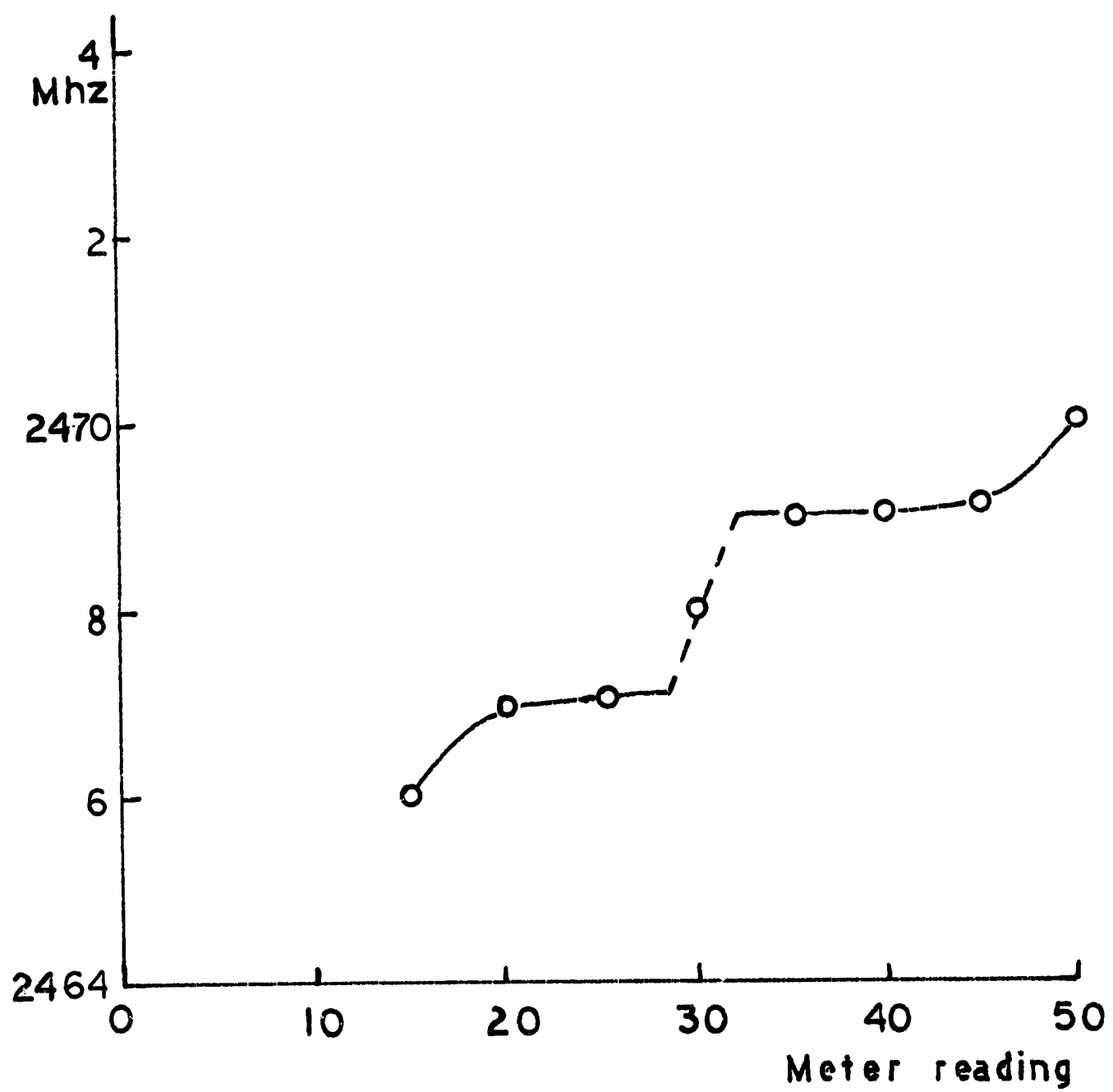
Figure B13. Frequency stability of magnetron
