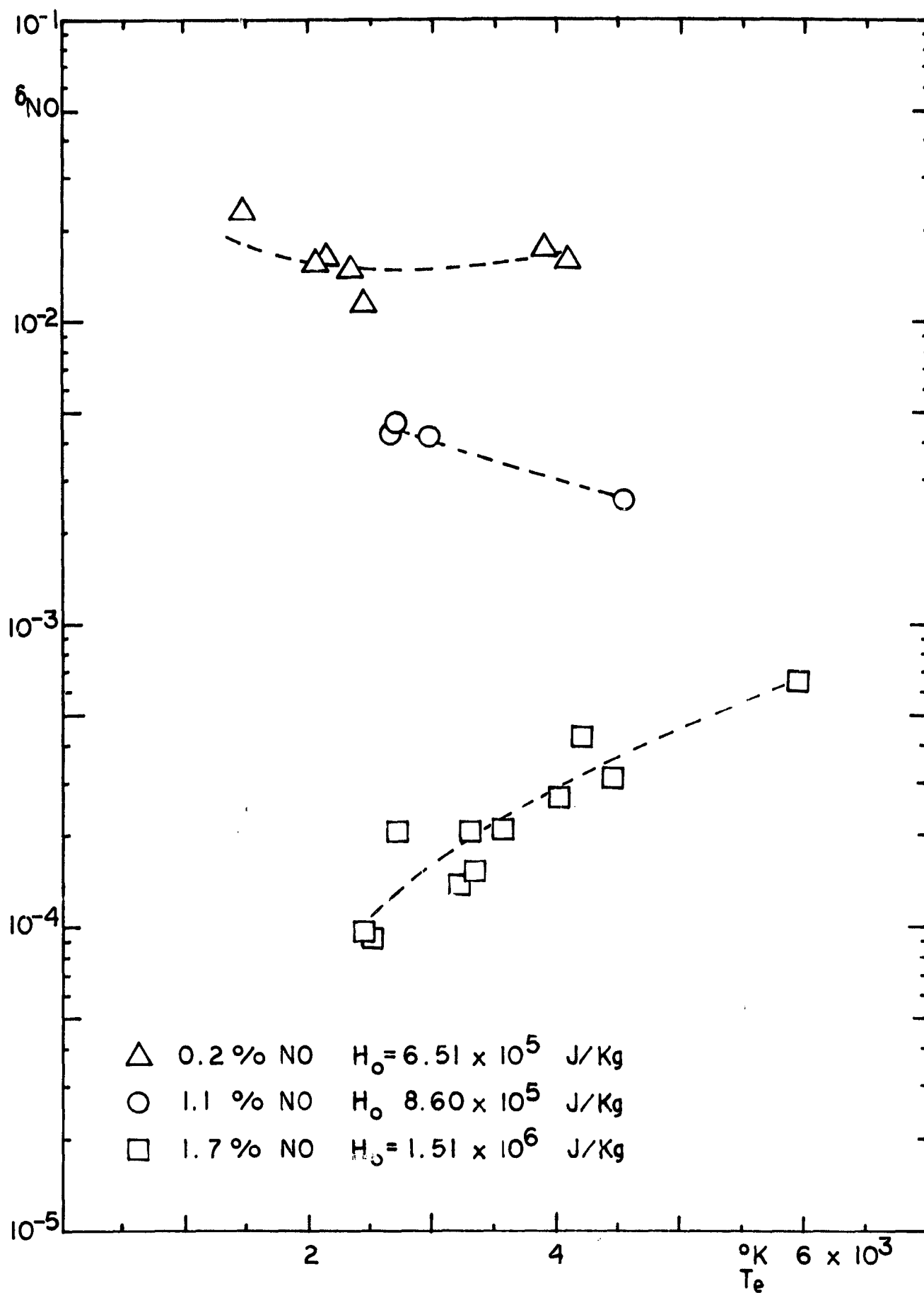
Figure 12. Electron energy-loss factor for nitric oxide as a function of electron temperature, computed from the mixture rule for three molecular concentrations of NO in argon and plasma stagnation enthalpy conditions
