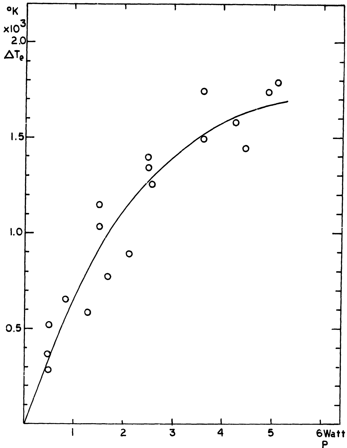
Figure 6. Measured electron temperature rise, \Delta T_e , as a function of rf power in prepurified nitrogen plasmajet with H_o \approx 1200 BTU/lb produced by Thermal Dynamics 50-N arcjet
