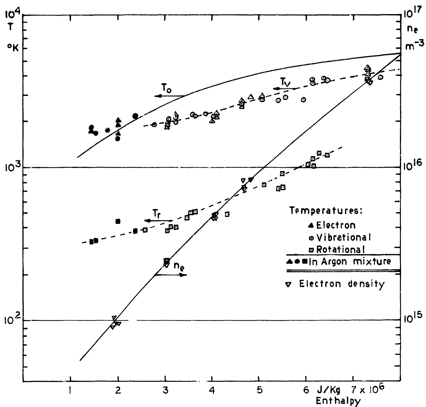
Figure D1. Measured temperatures and number densities in plasmas of pure nitrogen and nitrogen-argon mixtures (55% N 2 - 45% A, by volume), as a function of stagnation enthalpy.
