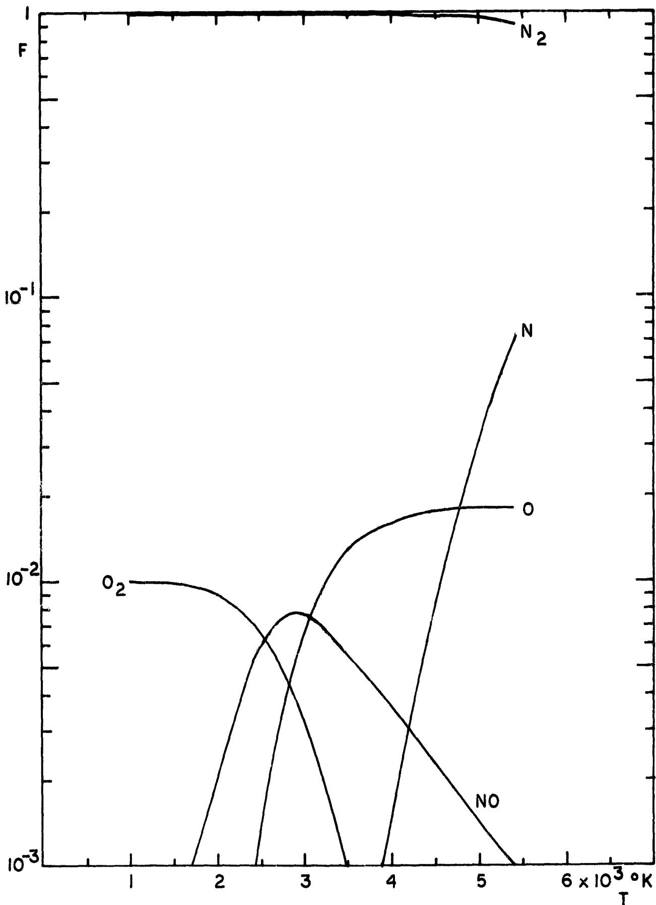
Figure C8. Equilibrium composition of a 1% O_2 - 99% N_2 mixture at 1 atmosphere pressure as a function of temperature (and enthalpy)
