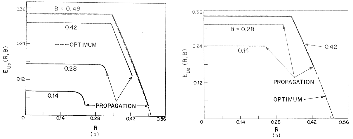
Fig. 11. (a) E(R) for optimum and sequential decoding of a systematic V = 2 convolutional code on a binary symmetric channel. p = 3/64 . (b) E_{Us}(R, B) for equal generator length codes on the same channel as in (a).
