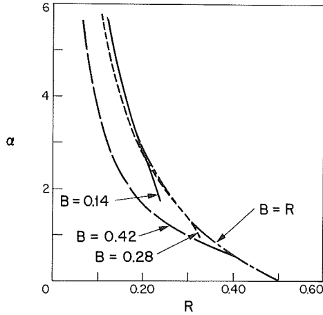
Fig. 11. (a) E(R) for optimum and sequential decoding of a systematic V = 2 convolutional code on a binary symmetric channel. p = 3/64 . (b) E_{Us}(R, B) for equal generator length codes on the same channel as in (a).
