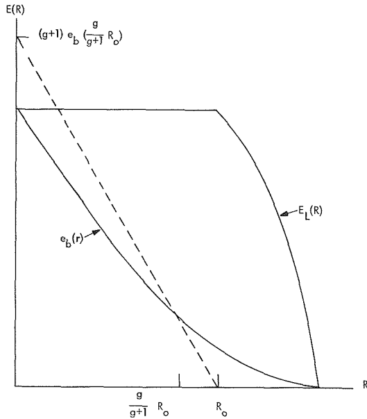
Fig. 3. Construction of E_L(R) .
