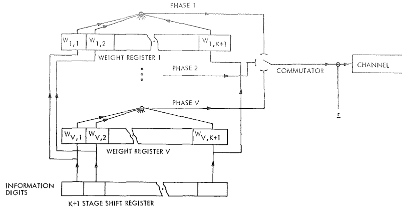
Fig. 1. Convolutional encoder.
