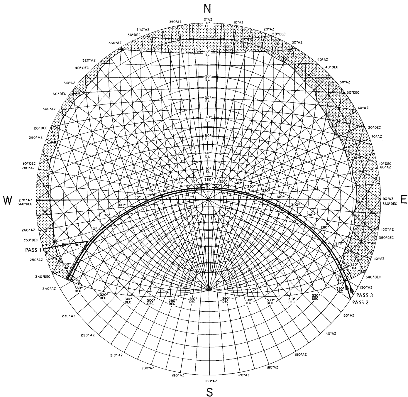
Fig. 30 Stereographic projection for DSS 42
