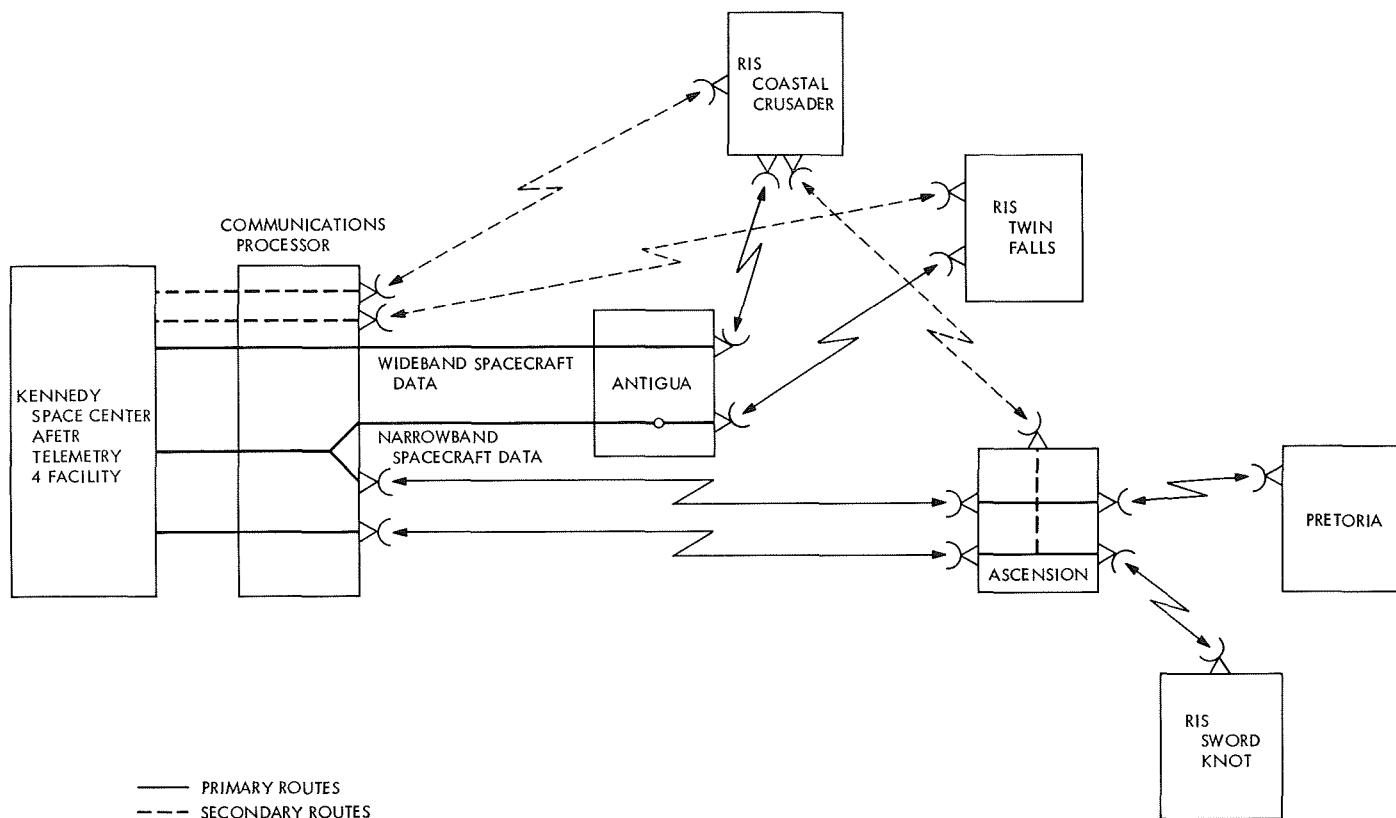
Fig. 25. Real-time telemetry circuits
