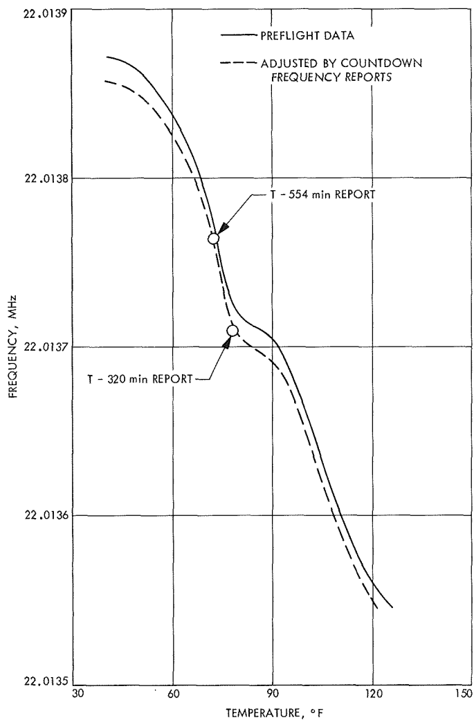
Fig 44. Transponder A frequency vs temperature (two way)
