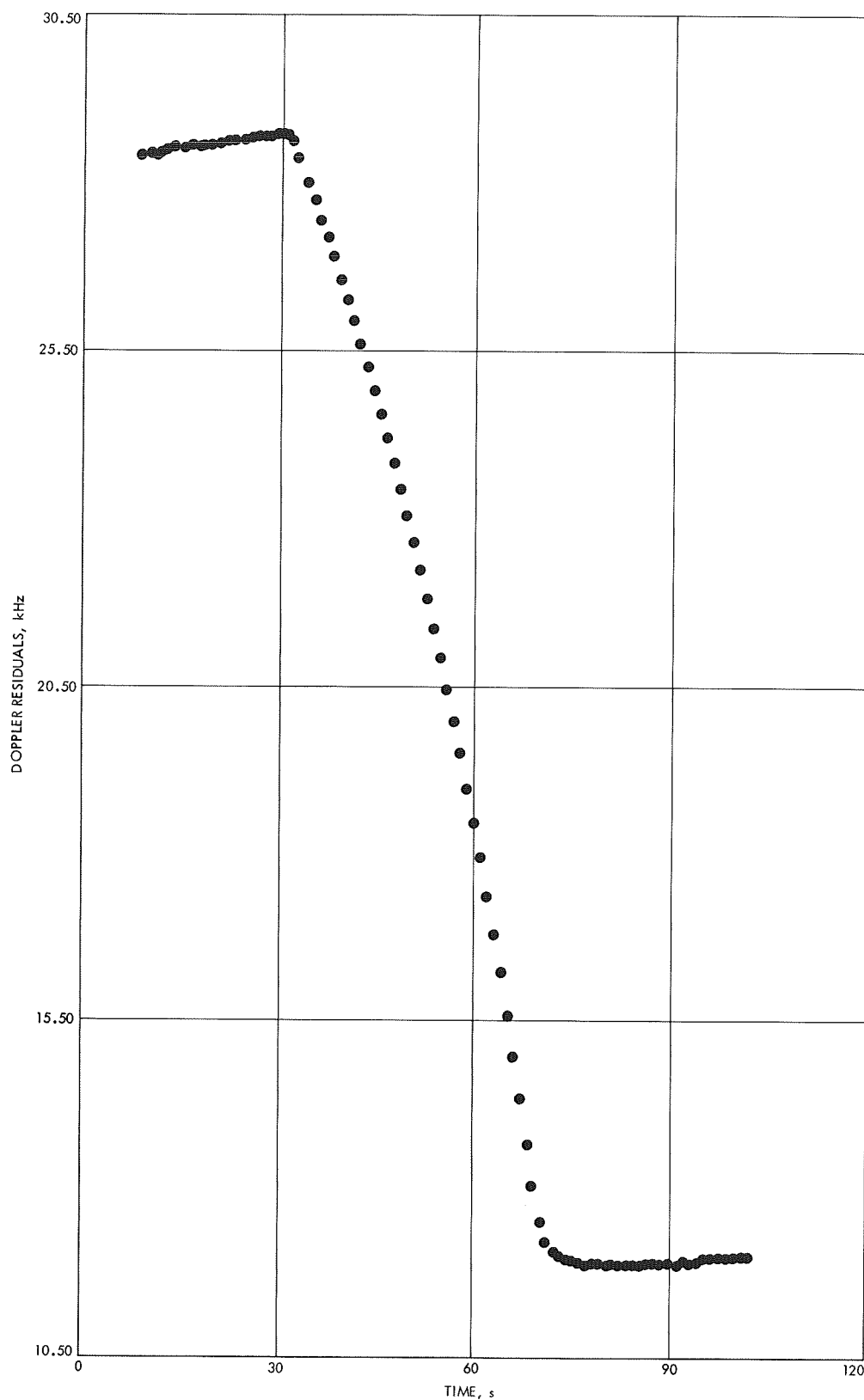
Fig. 73. Main retromaneuver phase one-way doppler residuals received by DSS 11 (time from 00:44:20 GMT on September 11, 1967)
