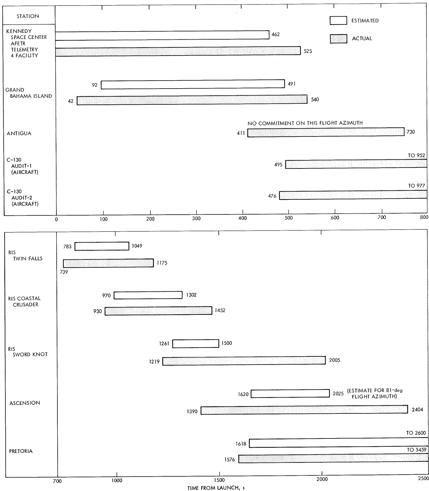
Fig. 35. Estimated and actual AFETR VHF telemetry coverage
