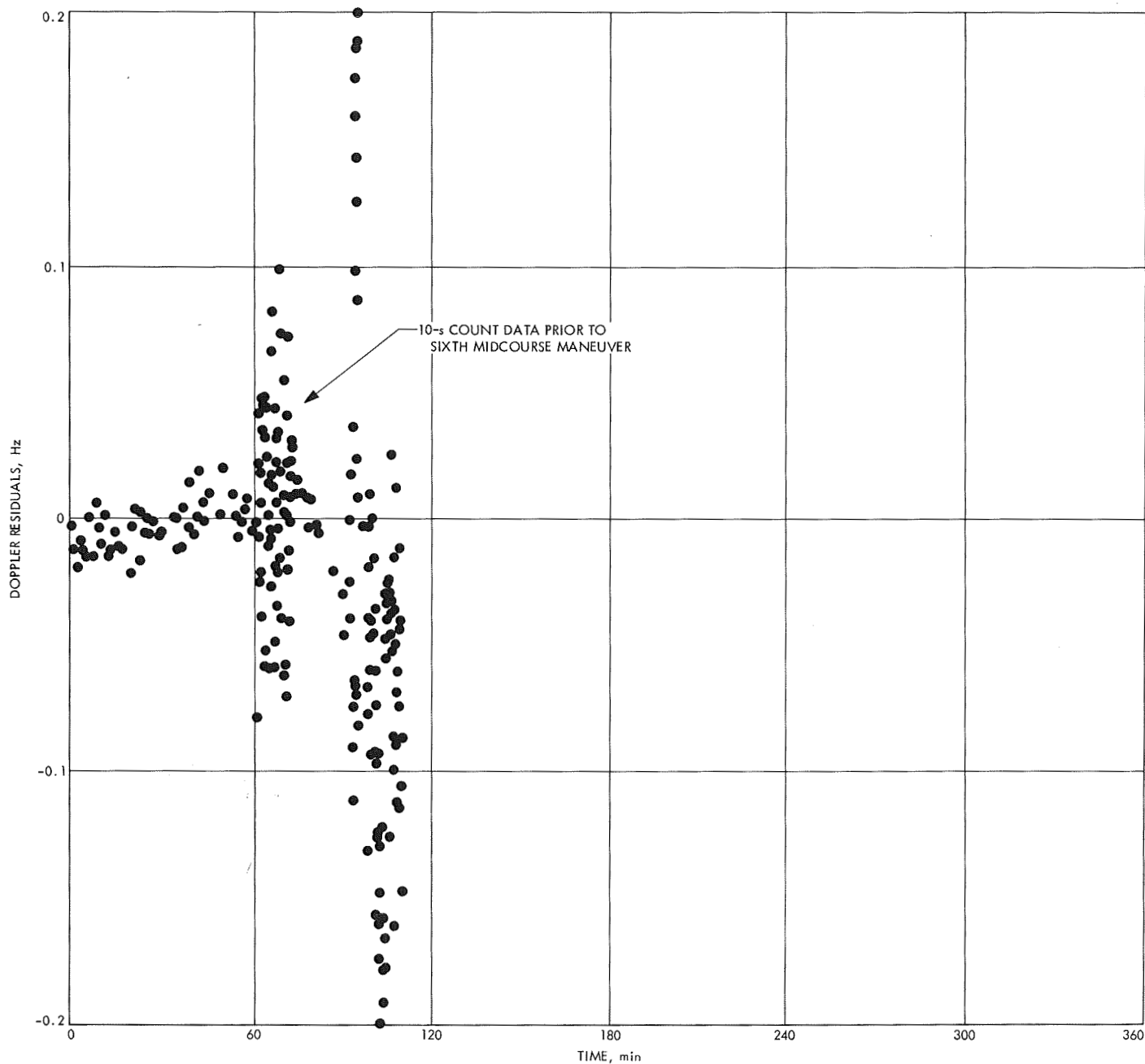
Fig. 62. Second pass two-way doppler residuals received by DSS 11 (time from 21:39:00 GMT on September 9, 1967)
