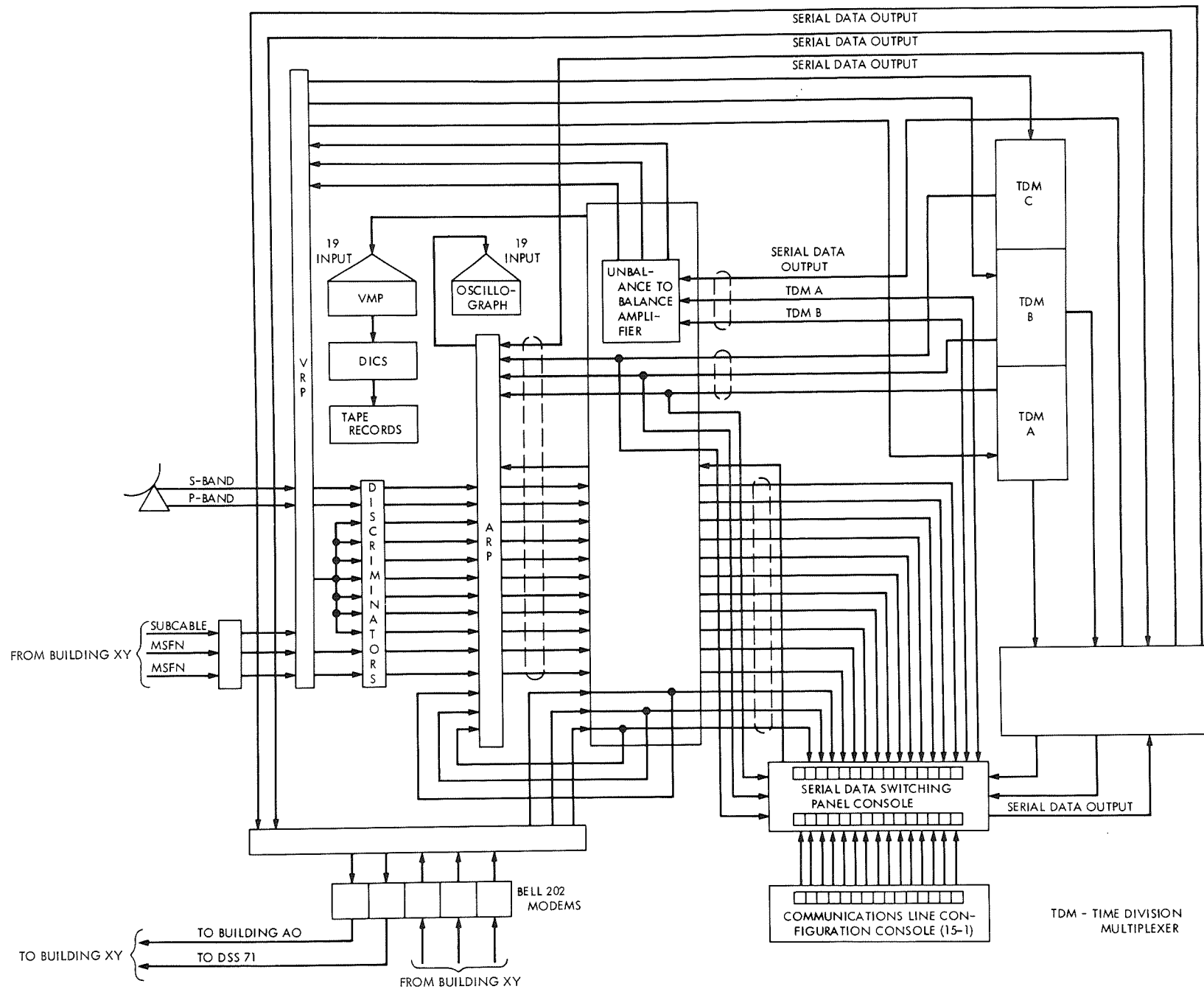
Fig. 12. AFETR serial data routing and switching system
