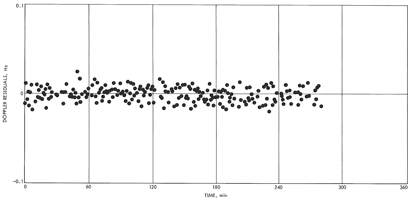
Fig. 53. First pass two-way doppler residuals received by DSS 51 (time from 15:33:00 GMT on September 9, 1967)
