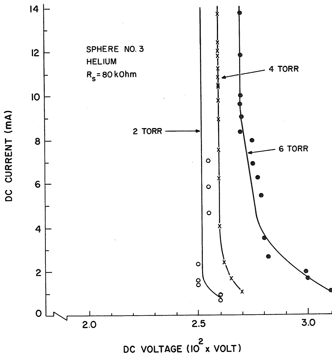
DC Discharge Characteristic
