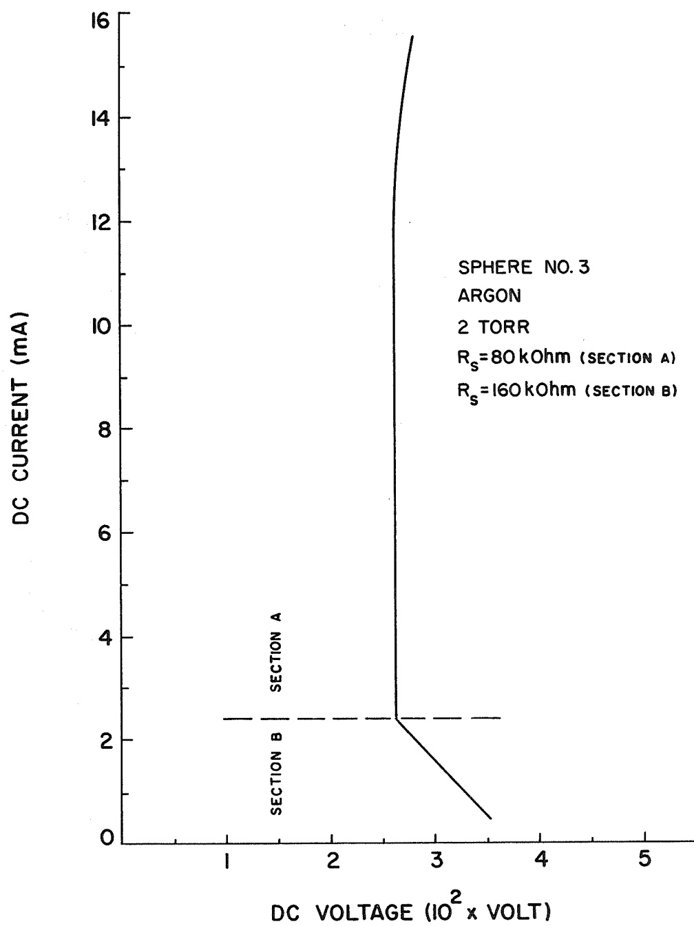
DC Discharge Characteristic
