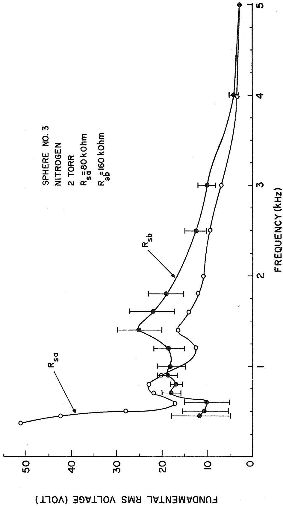
Magnitude of the Fundamental for Different Series Resistance Values vs Frequency
