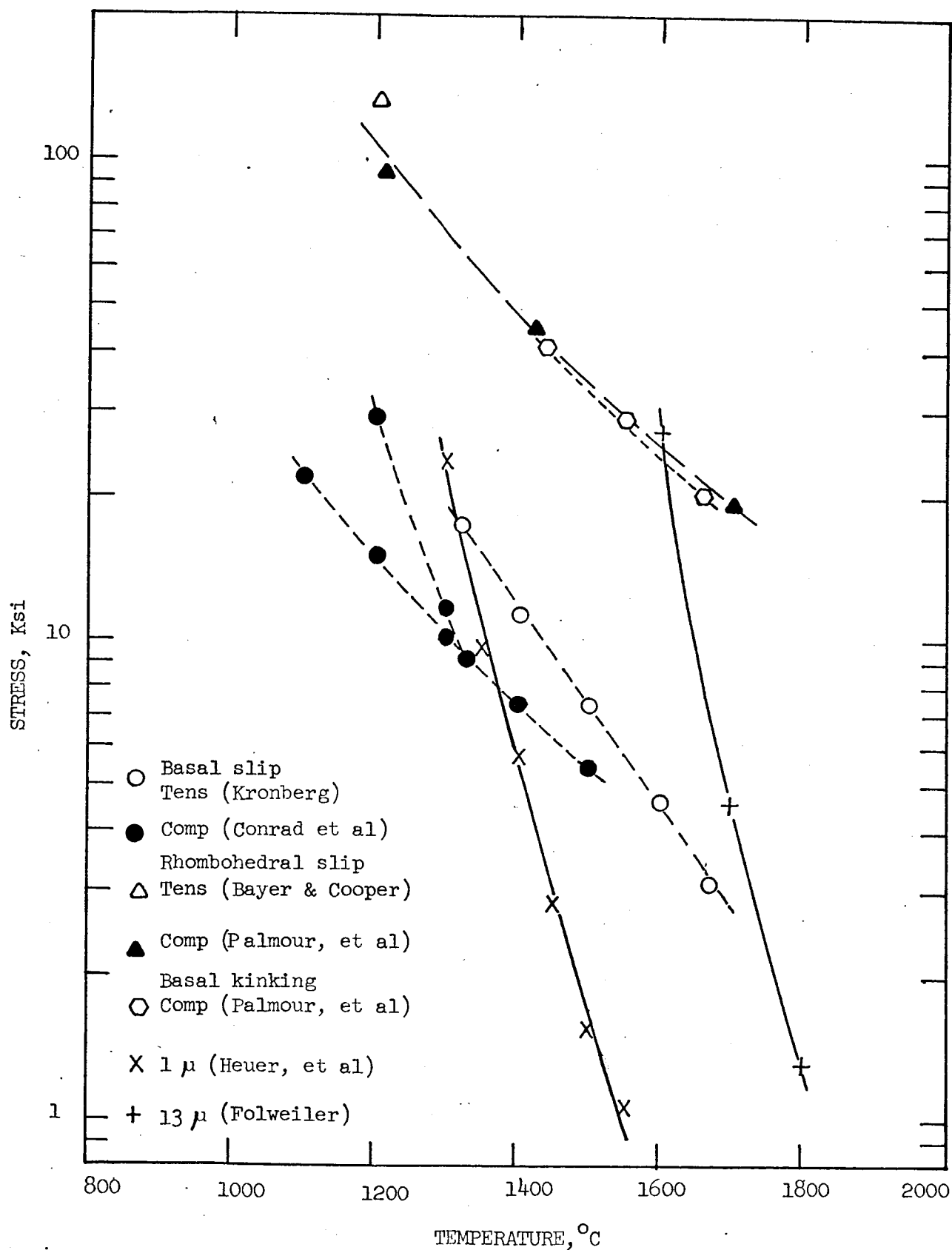
Figure 4. Yield Stress vs. Temperature for 1 \mu , and 13 \mu 24 Poly-crystalline Alumina and for Sapphire Oriented for Basal Slip, 23,48 Rhombohedral Slip, 49,50 and Basal Kinking. 49
